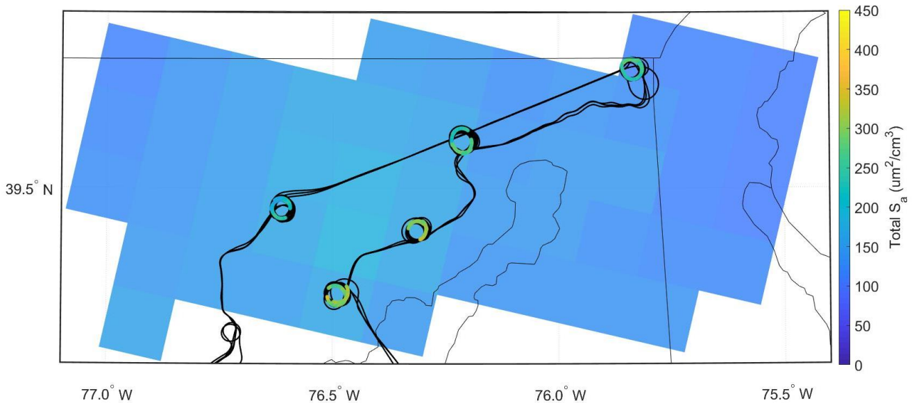
395 Figure 9: Flight path from 28 July with overlaid UHSAS S_a data within the 10 th layer of CMAQ altitude (~850-1000m) and gridded CMAQ S_a from layer 10 in the background. The CMAQ data is specifically at noon EST (UTC 16).
