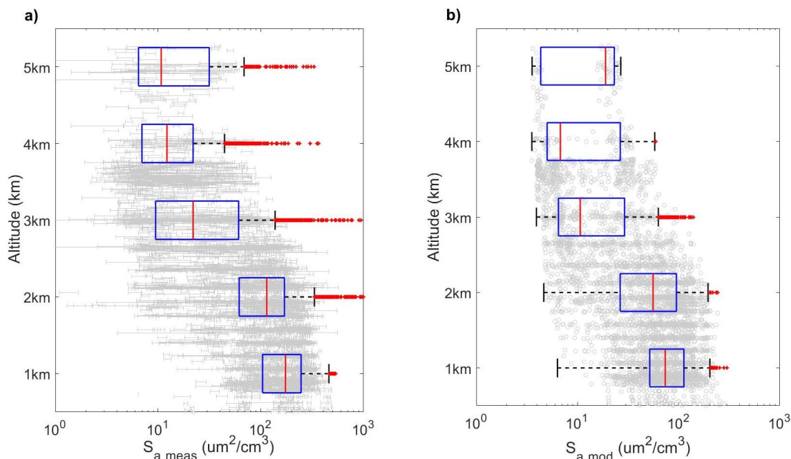
325 Figure 4: Average vertical profile of a) measured DISCOVER-AQ aerosol surface area concentration ( S_{a,meas} ) and b) CMAQ aerosol surface area concentration ( S_{a,mod} ) over the entirety of the DISCOVER-AQ campaign. Each measured point is an average of the points included in that 4D index corresponding to CMAQ. The overlaid boxplots show the median (red line within blue box), and interquartile ranges (blue box with the 25th percentile at the left end and 75th percentile at the right end) in 1km altitude bins. The labels on the altitude axis lie at the midpoint of the 1km altitude bin, and red crosses indicate outliers from the majority of the dataset at that altitude portion.
