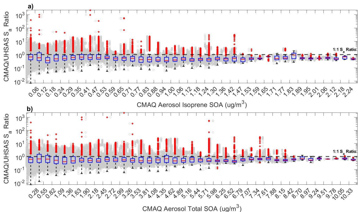
500 Figure 13: Interquartile ranges in S_{a,mod.}/S_{a,meas} as a function of the modeled (CMAQ) a) isoprene SOA concentration and b) total SOA concentration.
