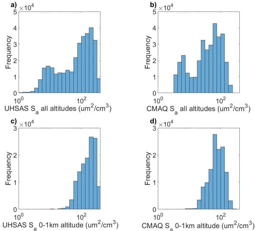
340 Figure 5: Histograms of a) measured aerosol surface area concentration (DISCOVER-AQ) at all altitudes, b) modeled aerosol surface area concentration (CMAQ) at all altitudes, c) measured aerosol surface area in the 0 to 1km altitude bin, and d) modeled aerosol surface area in the 0 to 1km altitude bin over the entirety of the DISCOVER-AQ campaign.
