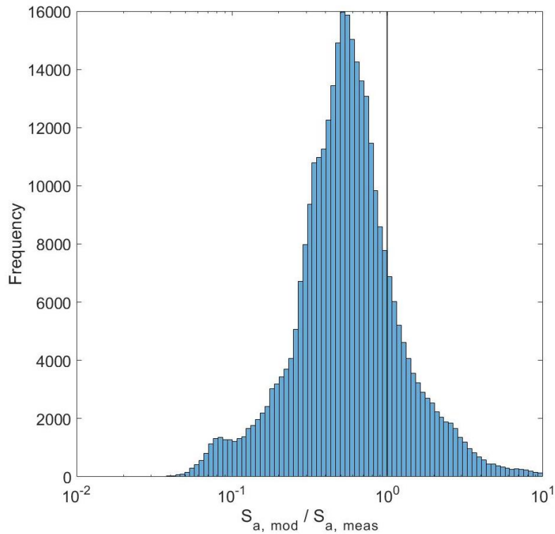
Figure 7: Histogram of the ratio of model to measured aerosol surface area concentration ( S_{a, \text{mod}}/S_{a, \text{meas}} ) over the full DISCOVER-AQ campaign.
