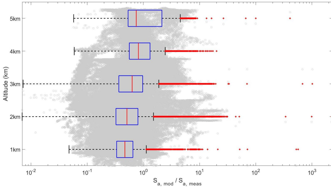
Figure 8: Ratio of modeled to measured aerosol surface area concentration ( S_{a,mod}/S_{a,meas} ) including median (red line within blue box), and interquartile ranges (blue box with the 25 th percentile at the left end and 75 th percentile at the right end) in 1km altitude bins. The red crosses outside of the bounds of the plot note outliers. The labels on the altitude axis lie at the midpoint of the 1km altitude bin.
