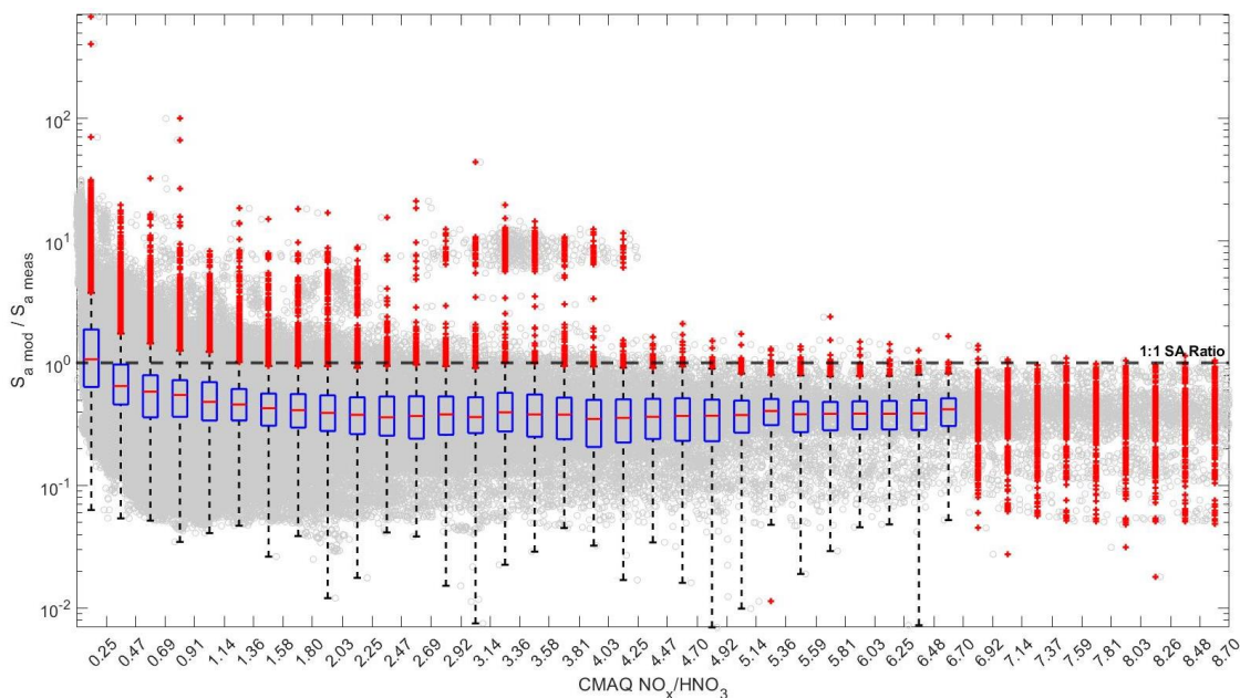
Figure 12: Interquartile ranges in S_{a,\text{mod.}}/S_{a,\text{meas}} as a function of the modeled (CMAQ) \text{NO}_x/\text{HNO}_3 concentration ratio.
