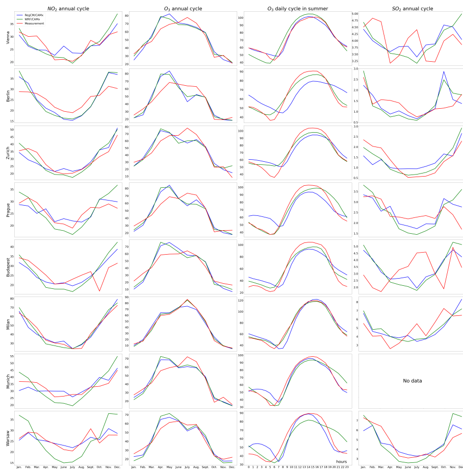
Figure 2. Comparison of modelled (blue – RegCM/CAMx ; green – WRF/CAMx ) and measured (red; AirBase data) urban and suburban average monthly concentrations of \text{NO}_2 ( left 1st column ) and \text{O}_3 ( 2nd column ), the average JJA diurnal cycle of \text{O}_3 ( middle 3rd column ) and the average monthly concentrations of \text{SO}_2 ( right 4th column ) for eight different cities selected from the total 19 considered in the study, namely Berlin, Budapest, Milan, Munich, Prague, Zurich, Vienna and Warsaw. Units in \mu\text{gm}^{-3} . Data are averaged across all available urban and suburban type background stations within the chosen city. No data for \text{SO}_2 in Munich as no corresponding measuring station was available.
