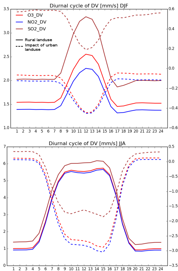
Figure 11. The diurnal cycle of the impact of urbanization on rural deposition velocities (DV; solid lines; left y-axis ) and the impact of urbanization ( dashed lines; right y-axis ) for 2015-2016 DJF (up) and JJA (bottom) for NO 2 (blue), SO 2 (brown) and O 3 (red) in mm.s -1 .
