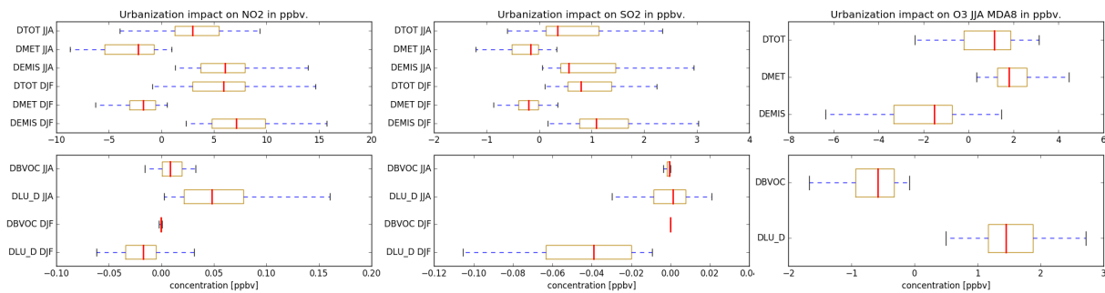
Figure 3. The 2015-2016 DJF and JJA averaged impact of each component-of-contributor to the rural-urban transformation including the total impact averaged over all chosen city for NO 2 , SO 2 and O 3 in ppbv. In case of ozone, only the summer averaged MDA8 (maximum daily 8-hour average) is shown. The boxplots show the 25% to 75% quantiles including the minimum and maximum value across all cities . The red line showing shows the median. Values are taken from model grid-cell that covers the city center. The upper sub-figures show the two main impacts-contributors including the total impact ("DEMIS", "DMET" and "DTOT") while the lower one the minor contributors ("DLU_D" and "DBVOC")
