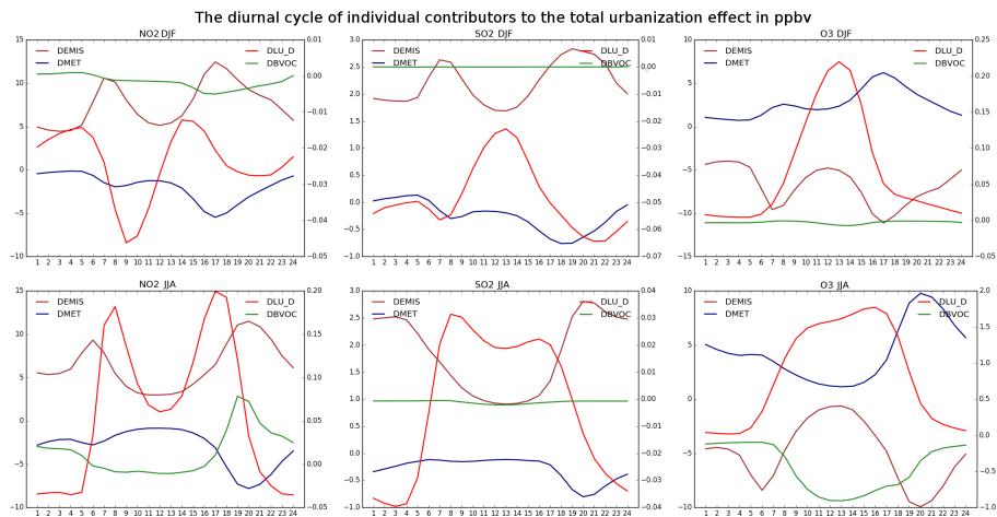
Figure 10. The 2015-2016 average diurnal cycle of the individual components of contributors to RUT for NO 2 (left), SO 2 (middle) and O 3 (right) as DJF (upper row) and JJA (bottom row) average. The brown and blue lines stand for the two stronger contributors ("DEMIS" and "DMET", left y-axis), while red and green stand for minor the weaker contributors "DLU_D" and "DBVOC" (right y-axis). Units in ppbv. Times in UTC (i.e. the local time is +2 hours in JJA and +1 hours in DJF).
