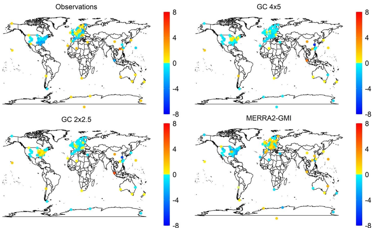
720 Figure 9. Decadal trends (ppb decade -1 ) at surface locations in TOAR-compiled observations, GC 4x5, GC 2x2.5, and MERRA2-GMI. GC 4x5 refers to the GEOS-Chem v12.9.3 simulations at the 4°x5° horizontal resolution, GC 2x2.5 is the same model at 2°x2.5°, and MERRA2-GMI refers to the NASA GEOS GMI at ~50km. Increases are shown in shades of red, and decreases are shown in shades of blue.
