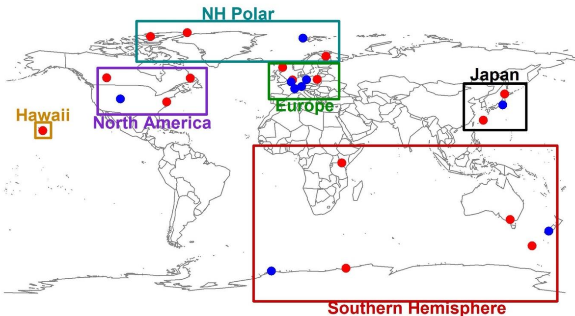
240 Figure 1. Map showing ozonesonde locations. Locations with data spanning 1990-2017 are shown in red, and locations with data extending to the 1980s are shown in blue. The boxes represent the regions into which all ozonesondes are grouped.
