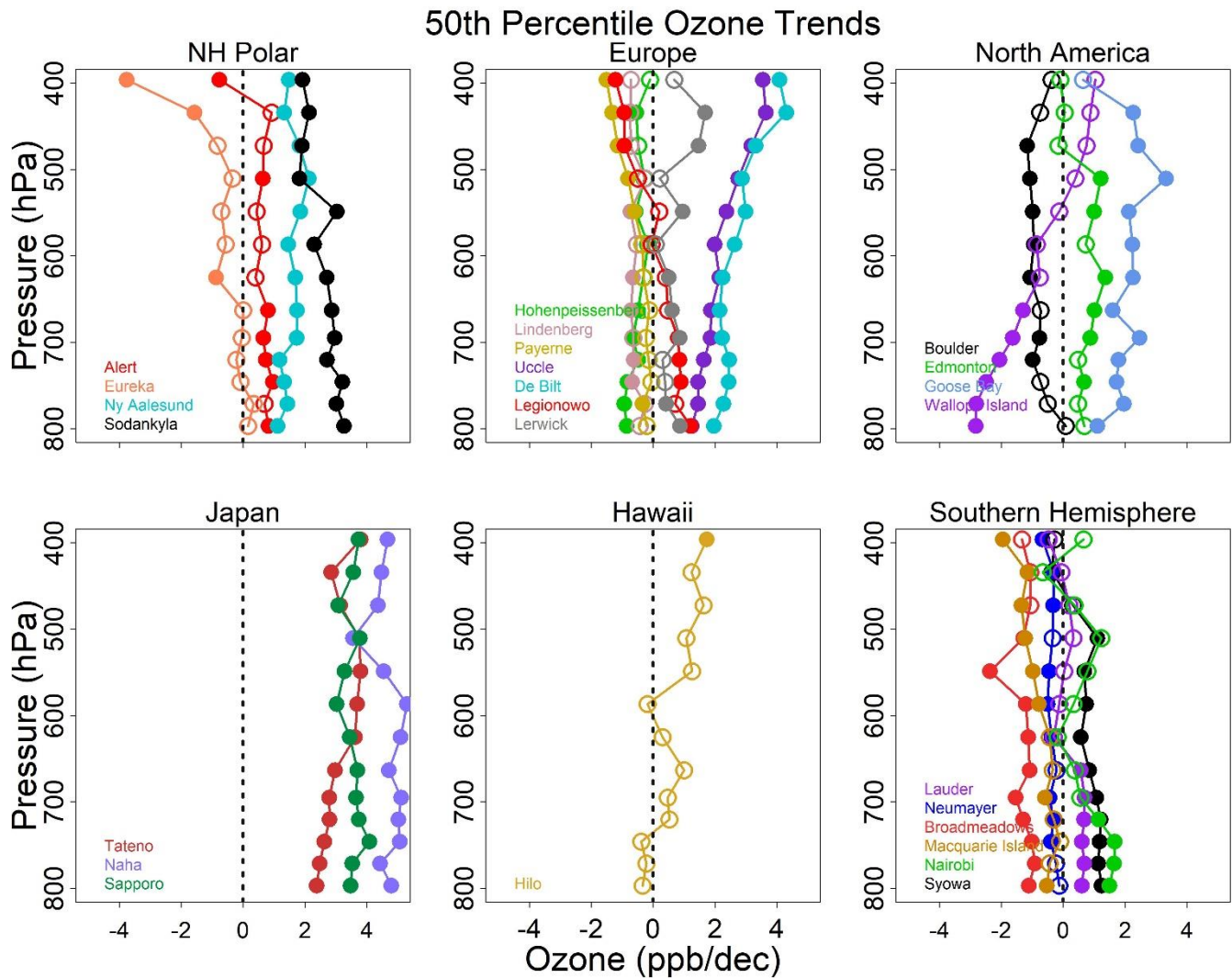
470 Figure 3. Trends ( \text{ppb decade}^{-1} ) through the free troposphere (800-400 hPa, reduced to GEOS-Chem pressure levels ) at the 25 global ozonesonde sites with data from 1990-2017, distributed into six regions. Solid circles indicate that the trends are statistically significant ( p < 0.1 ), while open circles denote statistically insignificant trends.
