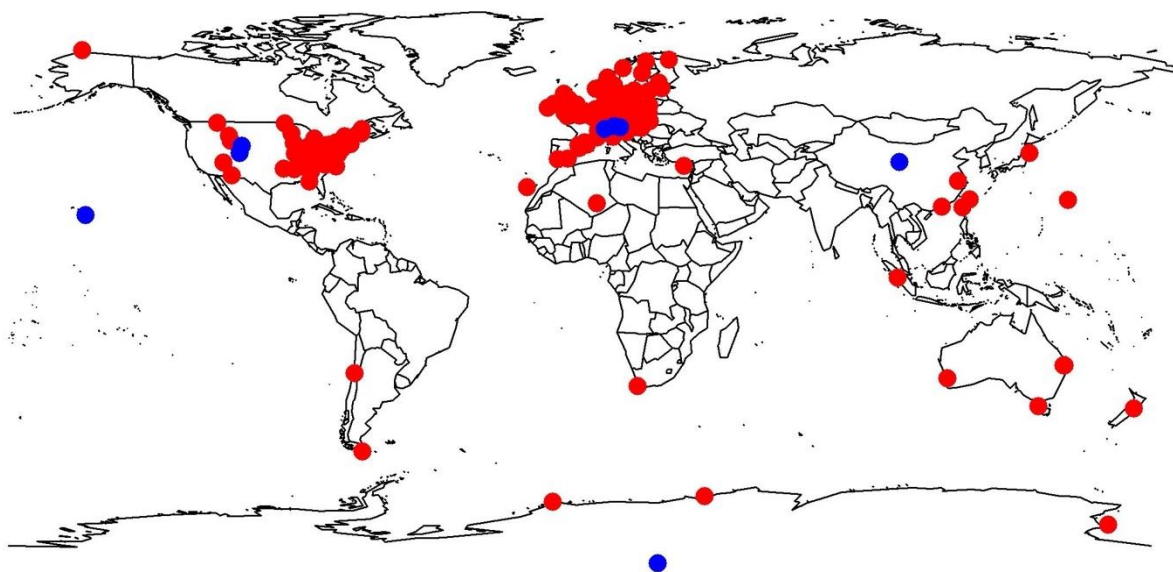
280 Figure 2. Surface site locations of background-baseline ozone monitors with data spanning 1990-2014, compiled and processed by the TOAR (Tropospheric Ozone Assessment Report) Database team. High elevation sites (>2800 m a.s.l.) that represent the lower troposphere or FT are shown in blue.
