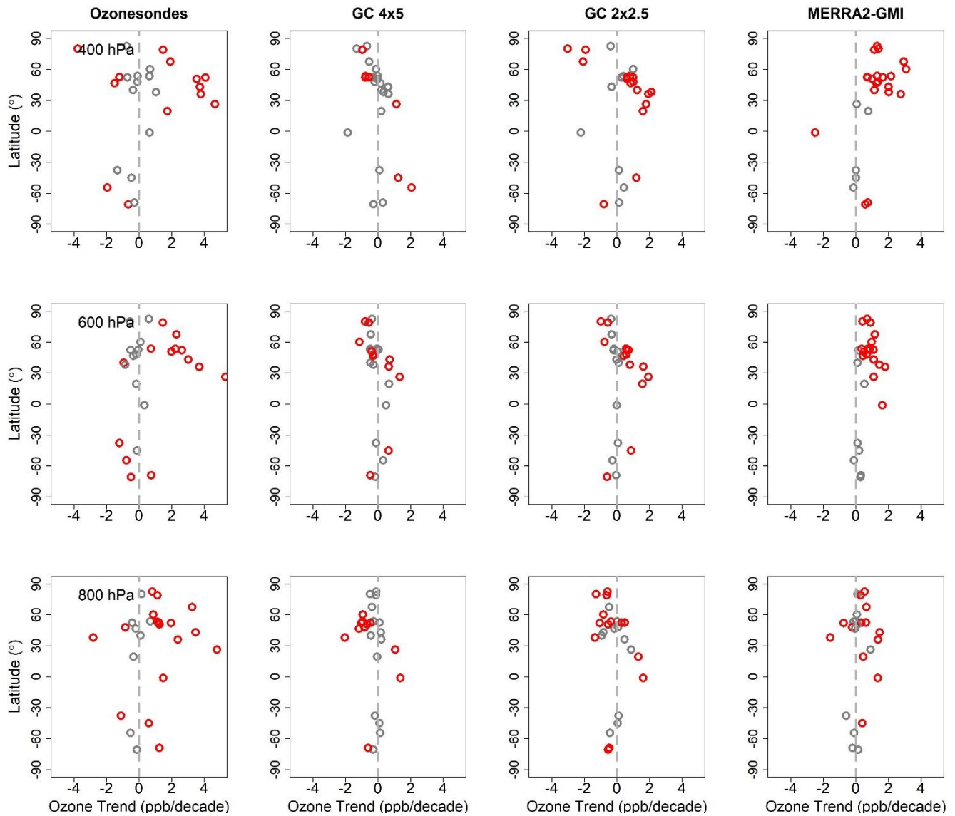
670 Figure 7. Summary of 1990-2017 trends in ozonesondes (left column) and the simulations (other columns). GC 4x5 refers to the GEOS-Chem v12.9.3 simulations at 4^\circ \times 5^\circ , GC 2x2.5 is the same model at 2^\circ \times 2.5^\circ , and MERRA2-GMI refers to the NASA GEOS GMI at \sim 50 km resolution. The trend in \text{ppb decade}^{-1} is plotted as a function of ozonesonde launch site latitude. Red circles indicate significant trends ( p < 0.1 ), and gray circles indicate insignificant trends.
