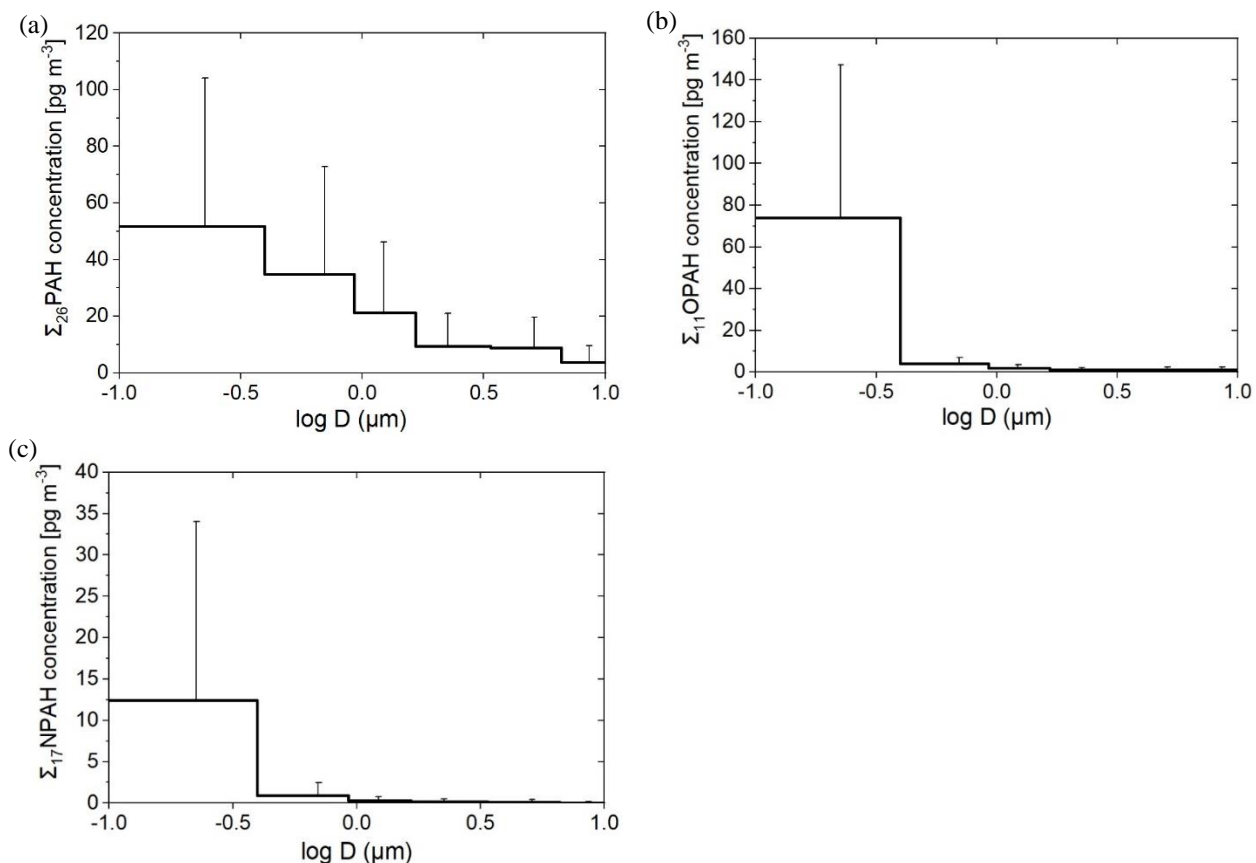
815 Figure 8: Campaign average mass size distributions (MSDs) of (a) \Sigma_{26}\text{PAHs} , (b) \Sigma_{11}\text{OPAHs} and (c) \Sigma_{17}\text{NPAHs} during the campaign; including standard deviation as error bars.
