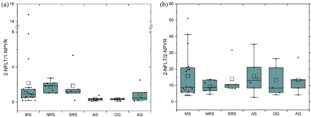
Figure 6: Box-Whisker plot of the ratios (a) 2-NFLT/1-NPYR and (b) 2-NFLT/2-NPYR across sea regions (MS: Mediterranean Sea; NRS: northern Red Sea; SRS: southern Red Sea; AS: Arabian Sea; OG: Gulf of Oman; AG: Arabian Gulf; Empty square: mean value; Filled, grey triangles: Measurement points; Box with additional borders: interquartile range (IQR) bound by the 75 th and 25 th percentile and range of 1.5 IQR; Horizontal line: Median).
