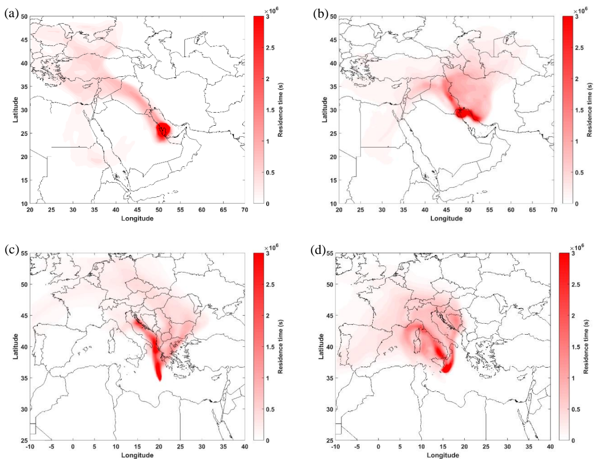
Figure 7: Distribution of residence times of air masses received in the Arabian Gulf: (a) D30 (29-30 July 2017), (b) D31 (3-4 August 2017) and the Mediterranean Sea: (c) D54-55 (27-28 August 2017), (d) D58 (29-30 August 2017) using FLEXPART Lagrangian particle dispersion model samples.
