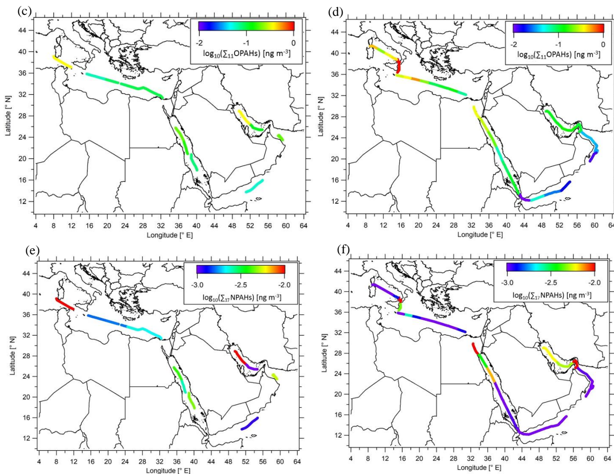
Figure 2: Total concentration (logarithmic scale) of \Sigma_{26} PAHs, in (a) and (b), \Sigma_{11} OPAHs in (c) and (d) and \Sigma_{17} NPAHs in (e) and (f) during the first leg in (a), (c), (e) and the second leg in (b), (d), (f). Spatial resolution of data limited to sampling stretches (see Fig. S1).
