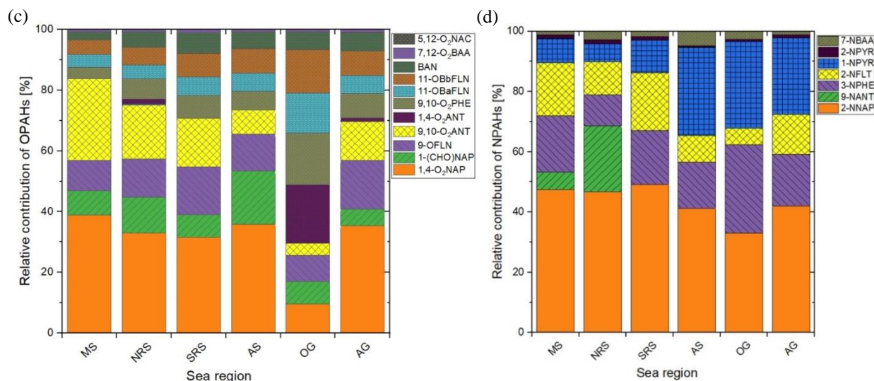
Figure 3: Relative amount of (a) 16 PAHs, (b) RPAHs, (c) OPAHs, (d) NPAHs across sea regions (MS: Mediterranean Sea; NRS: northern Red Sea; SRS: southern Red Sea; AS: Arabian Sea; OG: Gulf of Oman; AG: Arabian Gulf). Full names of the substances are given in Sects. 2.3.1, 2.3.2 and Tables 1 and S2. Only quantified species included in legends.
