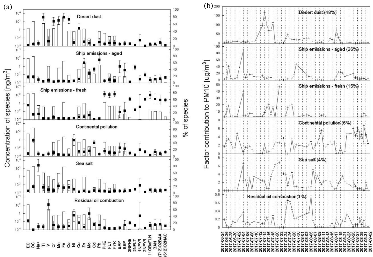
Figure 4: PMF group 2: (a) Factor profiles (Bars: Concentration of the species, black squares: Percentage of the species explained, box: Displacement (DISP) average, whiskers: DISP max and DISP min) and (b) time series of factor contributions to sample composition.
