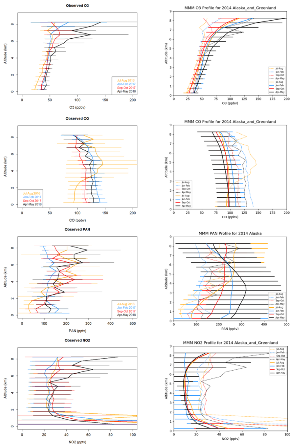
Figure 9: Mean vertical profiles of O_3 , CO , PAN and NO_2 (left) measured in Alaska and Greenland from the NASA ATom missions during summer 2016, winter 2017, autumn 2017 and spring 2018 (horizontal lines indicate 1 standard deviation spread around mean values at each altitude). (right) the MMM for the years 2014-15 (with the MMM standard deviation as horizontal lines). The observations appear as dashed lines in the right panels, for ease of comparing to the MMM.
