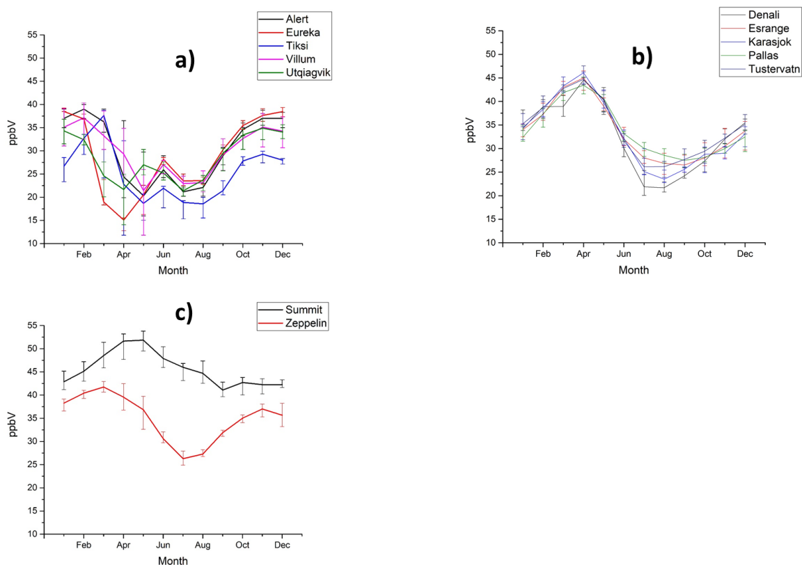
Figure 5: Seasonal behavior of surface O 3 at selected Arctic stations that are representative of a) coastal high Arctic b) near Arctic Circle and c) Greenland ice sheet and high Arctic, high-elevation sites. Monthly medians are calculated for the period 2003 to 2018. Data were not available from 2003 to 2006 for Villum and 2004 and 2013-
