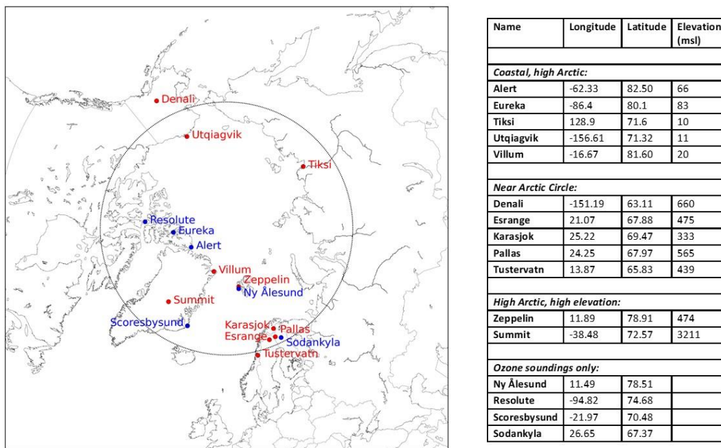
Figure 4. Map of the surface (red) and ozonesonde (blue) sites, cited in the present study, with coordinates and elevation. Eureka and Alert are both surface and soundings sites. ‘Utqiagvik’ was formerly called ‘Barrow’. The Arctic Circle at 66.55° N is also shown in the figure for reference.
