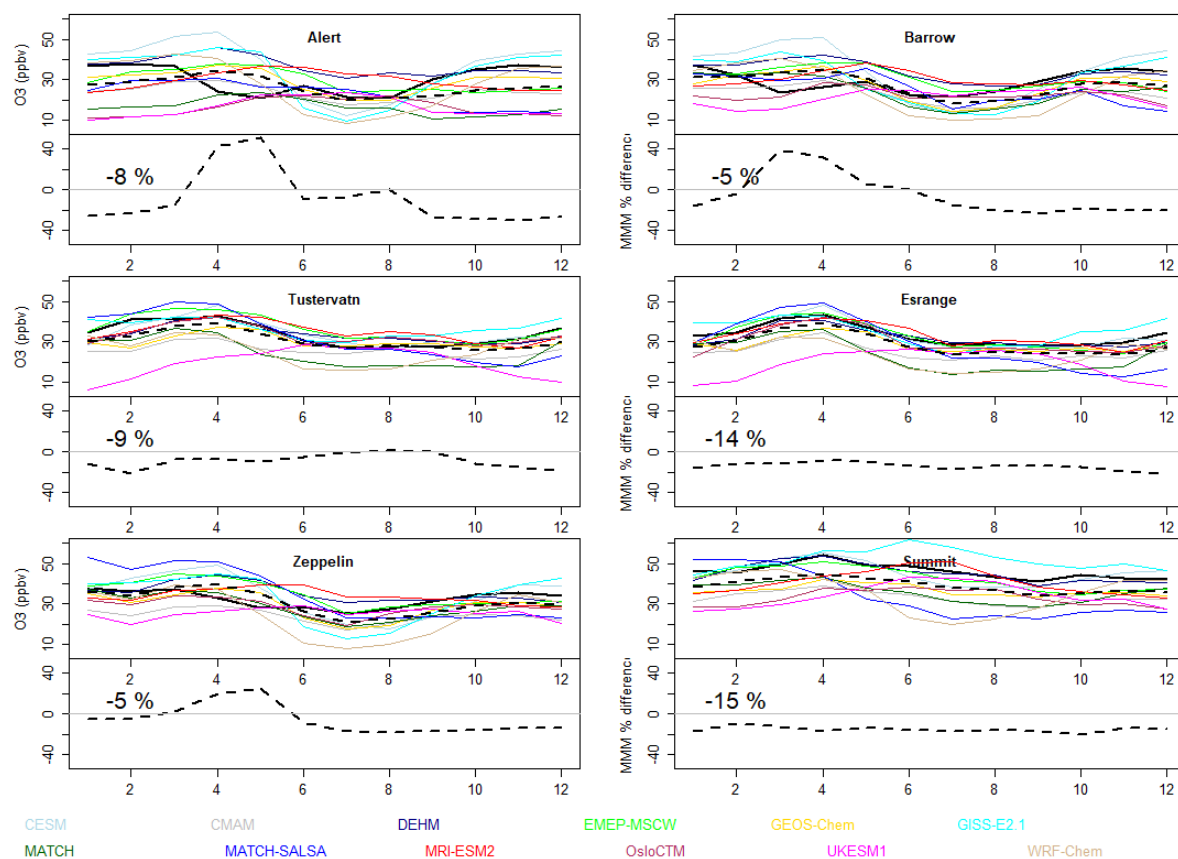
Figure 6: Arctic surface O 3 by month; seasonal cycle model comparisons. Top row: coastal high-Arctic sites; middle row: near-Arctic circle sites; bottom row: high elevation sites. The solid black line is the observed O 3 monthly means, and the dashed black line is the multi-model median. Bottom row: sub-panels show the MMM % difference [(MMM - measurements)/measurements*100].
