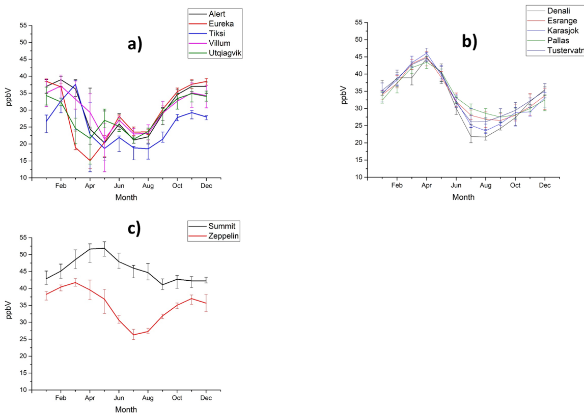
Figure 5: Seasonal behavior of surface O 3 at selected Arctic stations that are representative of a) coastal high Arctic b) near Arctic Circle and c) Greenland ice sheet-inland and high arctic, high-elevation sites. Monthly medians are calculated for the period 2003 to 2018. Data were not available from 2003 to 2006 for Villum and
