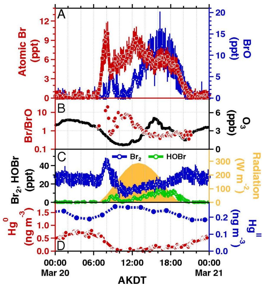
Figure 3: Time series at Uqiagvik on 20 March 2012 of measured (A) atomic bromine (Br) and bromine monoxide (BrO), (B) Br/BrO ratios and O 3 . Error bars represent propagated measurement uncertainties. Figure based on Wang et al. (2019, PNAS). (EPS figure provided for the report). From Figure 2 in Wang et al. (2019), PNAS, vol. 116, no. 29, pages 14479-14484, Copyright (2019) National Academy of Sciences.
