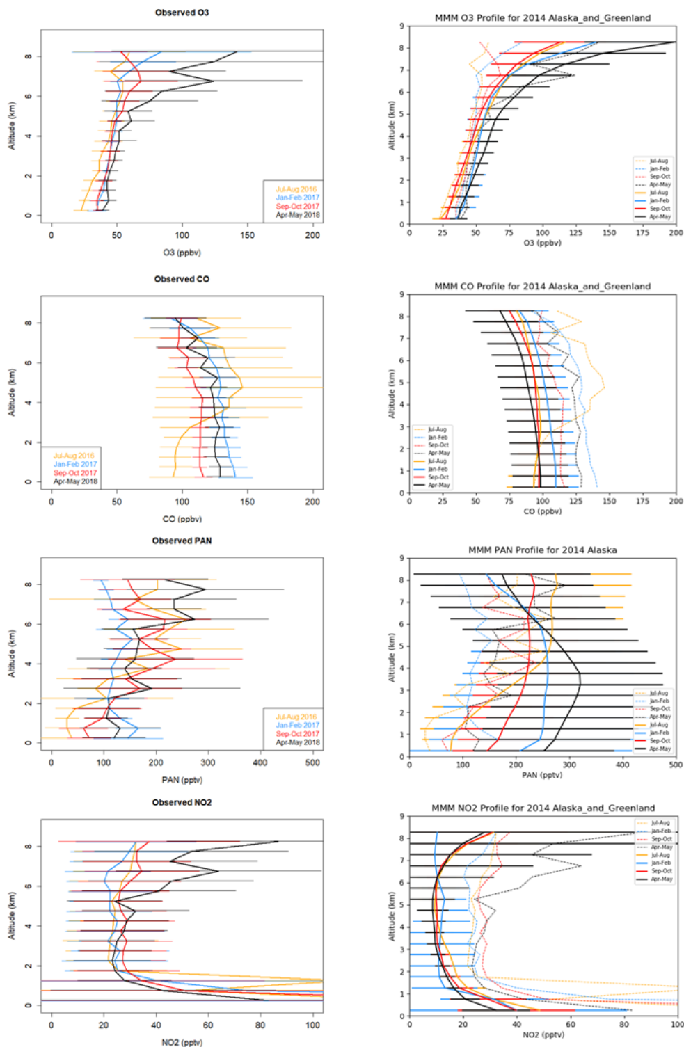
Figure 9: Mean vertical profiles of O_3 , CO , PAN and NO_2 ( left ) measured in Alaska and Greenland from the NASA ATom missions during summer 2016, winter 2017, autumn 2017 and spring 2018 (horizontal lines indicate 1 standard deviation spread around mean values at each altitude). ( right ) the MMM for the years 2014-15 (with the MMM standard deviation as horizontal lines). The observations appear as dashed lines in the right panels, for ease of comparing to the MMM.
