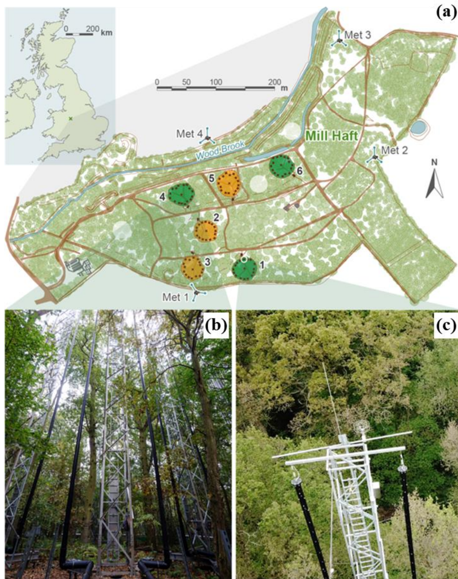
195 Figure 1: (a) schematic of the Birmingham Institute of Forest Research free-air carbon dioxide enrichment (BIFoR FACE) facility (see section 2.1 for site description). The coloured circles indicate the location of the FACE arrays, with green and orange denoting the fumigated and control arrays, respectively. The grey translucent circles mark the locations of the ghost arrays. The meteorological towers on the edge of the forest are labelled Met 1–4. (b) The perforated FACE vent pipes in array 4. (c) The two-dimensional sonic anemometer in array 1 (see section 2.2.2 for details of meteorological measurements). Figure 1a © Crown copyright and database rights 2021. Ordnance Survey (100025252).
