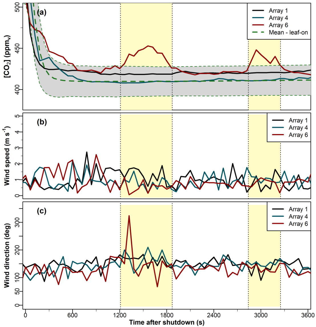
620 Figure 10: Timeseries of 1-minute averages in (a) the \text{CO}_2 mixing ratio, denoted [\text{CO}_2] (section 2.1), (b) wind speed, and (c) wind 625 direction after shutdown on 17 Aug 2020. In panel (a), the dashed green line shows the mean [\text{CO}_2] at each 1-minute time step after shutdown for the leaf-on period (section 2.2 for observational details). The grey shaded confidence interval in (a) shows one standard deviation either side of the mean. The standard deviation is presented here to emphasise that these venting events are not simply symptoms of the variability of the [\text{CO}_2] observations; on this dataset, it is larger than the other two measures of statistical variability used in this paper (the IQR and D_{med} ). The shaded yellow rectangles indicate the approximate duration of the venting events.
