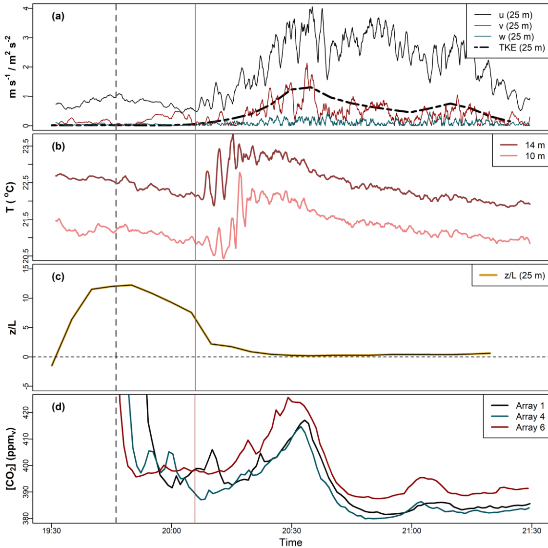
735 Figure A2: Timeseries after shutdown on 27 Aug 2019 of (a) the magnitude of the velocity vector components ( \text{m s}^{-1} ) and TKE ( \text{m}^2 \text{s}^{-2} ) at z = 25 \text{ m} , (b) T ( ^{\circ}\text{C} ), (c) z/L (where L is the Obukhov length, section 2.5), and (d) [\text{CO}_2] . The dashed grey vertical line indicates the shutdown time and the solid red line the approximate arrival time of the warm microfront described in the paragraph below. The high-resolution measurements in (a)–(c) are from on Met 1, at the southern edge of the BIFoR FACE facility (Figure 1 and section 2.1). (a) and (b) show 1-min rolling means.
