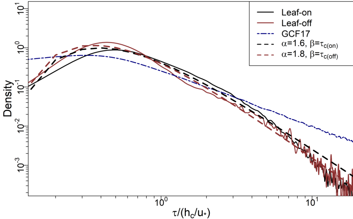
580 Figure 9: Solid black and red lines show PDFs of \tau (section 2.3) from BIFoR FACE (2.1 and Figure 1) during the leaf-on and leaf-off periods, respectively (section 2.2). Dashed lines show PDF estimates on the BIFoR FACE observations using Equation (7). Dot-
