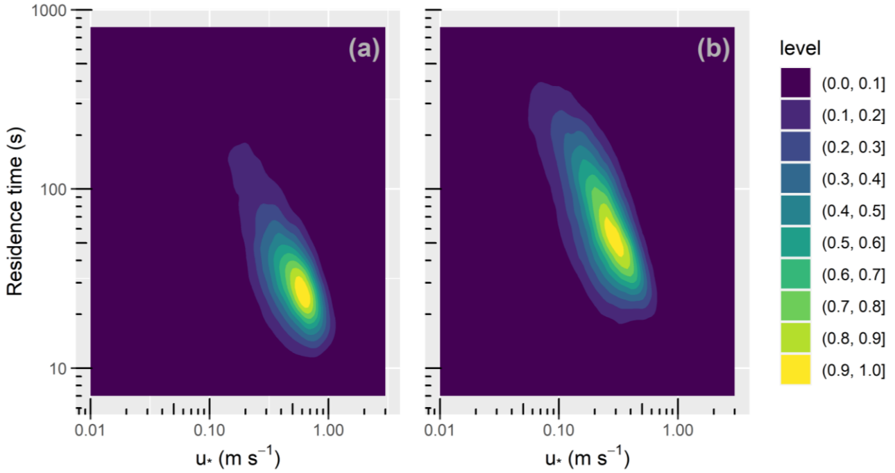
440 Figure 6: Two-dimensional density plots, showing the variation of the residence time \tau (section 2.3) with the friction velocity u_* (section 2.5) for the leaf-off (a) and leaf-on (b) periods (section 2.2 for observation details). The colour scale is normalised to account for the different sample sizes in the two periods. ‘Level’ in the colour scale refers to the density of each bin, normalised by the peak density for each observational period.
