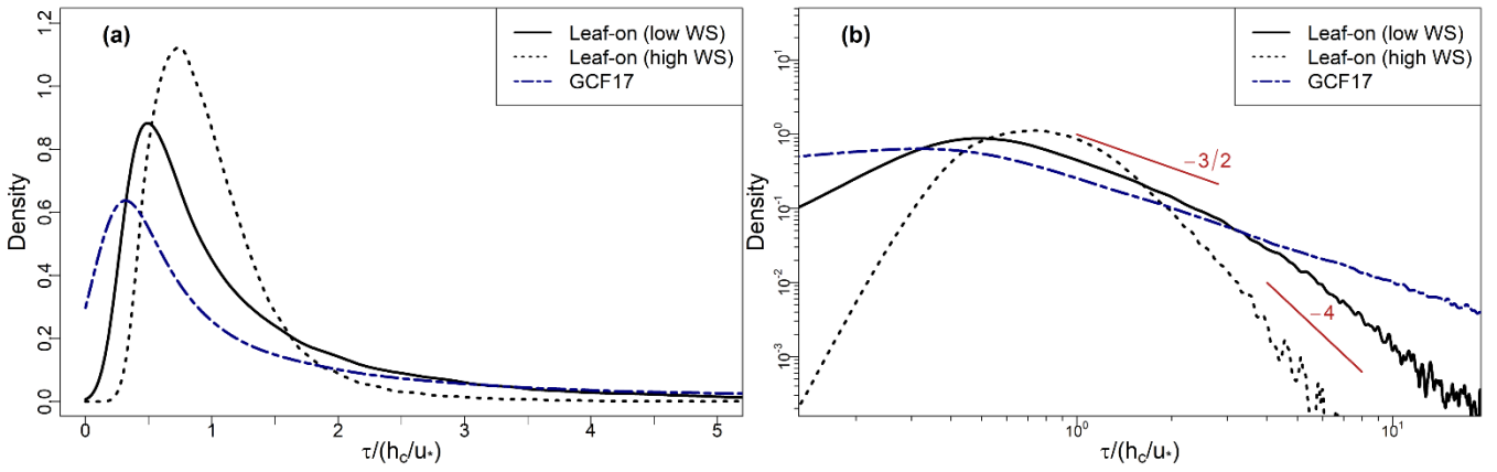
310 Figure 3: (a) Linear- and (b) logarithmic-scale PDFs of \tau , as defined in section 2.3, from BIFoR FACE during the lowest 50% (solid black) and highest 25% (black dashed) of wind speeds of the leaf-on period. GCF17's model in Eq. (1) is shown with the navy-blue dot-dash line. In (b), slopes of -3/2 and -4 are shown for reference. The slope of -3/2 is the power-law decay from GCF17, Eq. (1), and -4 is an arbitrary value to show the steeper decay of the right tail of the PDF of \tau in strong winds. Values of \tau normalised by the canopy turnover time h_c/u_* (section 2.4).
