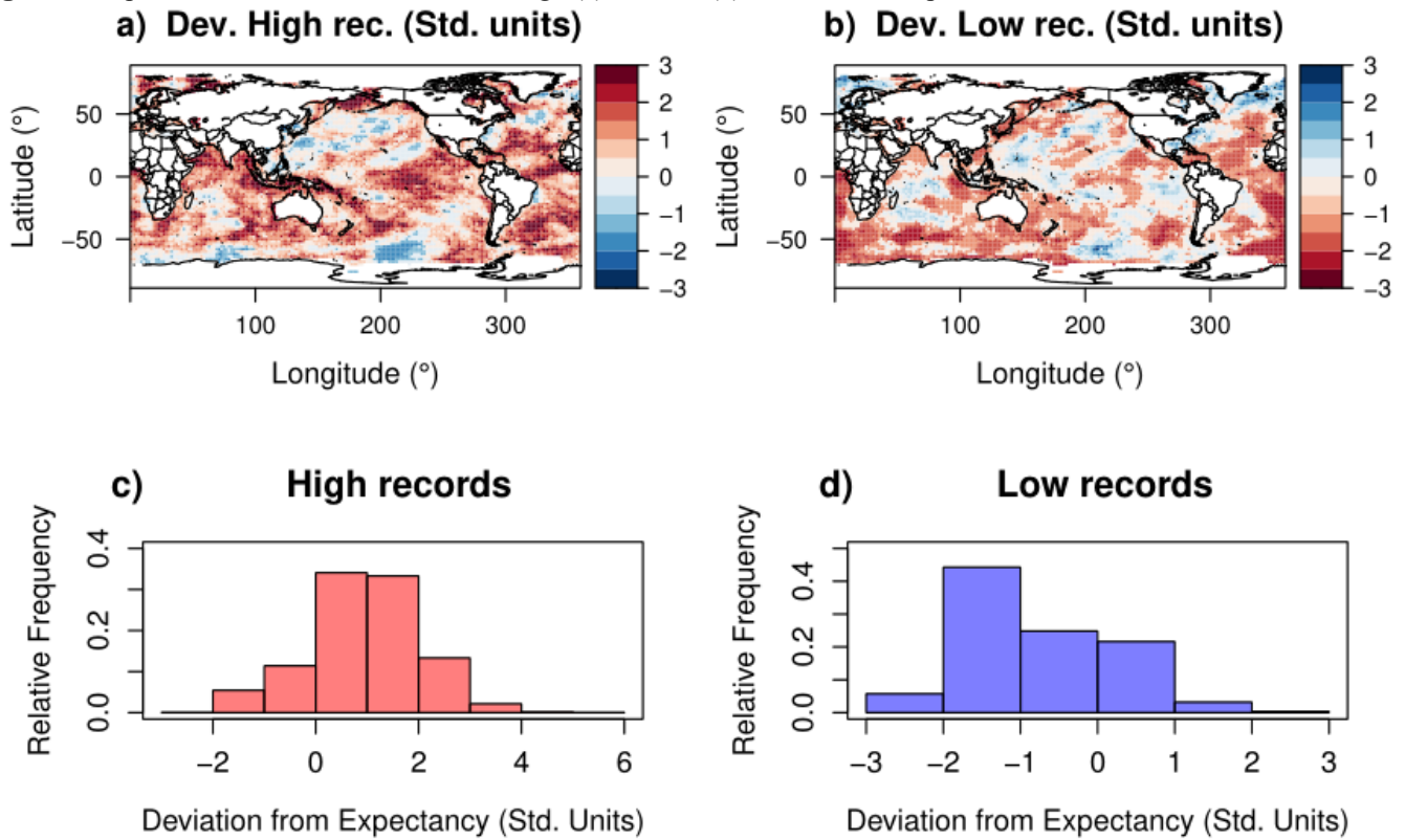
Figure 5: Departure of the observed number of high (a) and low (b) records from expectation, in units of standard deviation,
