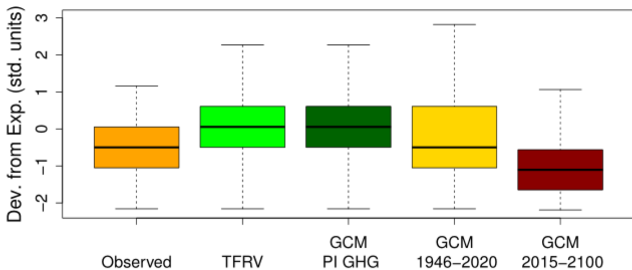
Figure 7: Boxplots of the high and low deviation from expected number for: observed SST between 1946-2020, TRFV, modelled SST of the PI control run samples, modelled SST between 1946-2020, projected SST between 2015-2100 (using the SSP2-4.5 scenario). The simulations were from the MRI-ESM2-0 CMIP6 global climate model.
