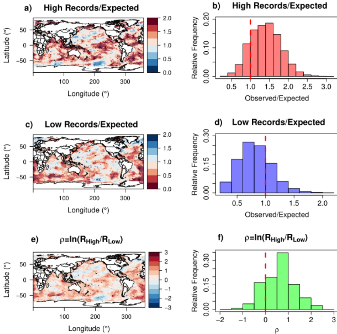
465 Figure 2: Number of observed high (a) and low (c) records of SST over the expected value for a TFRV in a 75-years time series. The trend indicator \rho , quantifies the asymmetry between the number of high and low records, \rho = \ln(R_{\text{High}}/R_{\text{Low}}) (e), and their respective distributions for the whole globe (b, d, f) are presented. The red dashed lines mark the thresholds where observed records exceeded the expected value in (b) and (d) or when the number of high records is larger than the low records in (f). These three different metrics combined can be used to simply and robustly detect trends in noisy time series. The 470 asymmetry between high and low records is evident, with a large number of high records and a small number of low records over most of the globe, particularly in the tropical and subtropical Atlantic, the Central Pacific, the eastern Indian Ocean, and the Southern sea. Note that, although the overwhelming majority of the ocean is warming, some islands of persistent cooling are observed in the maps.
