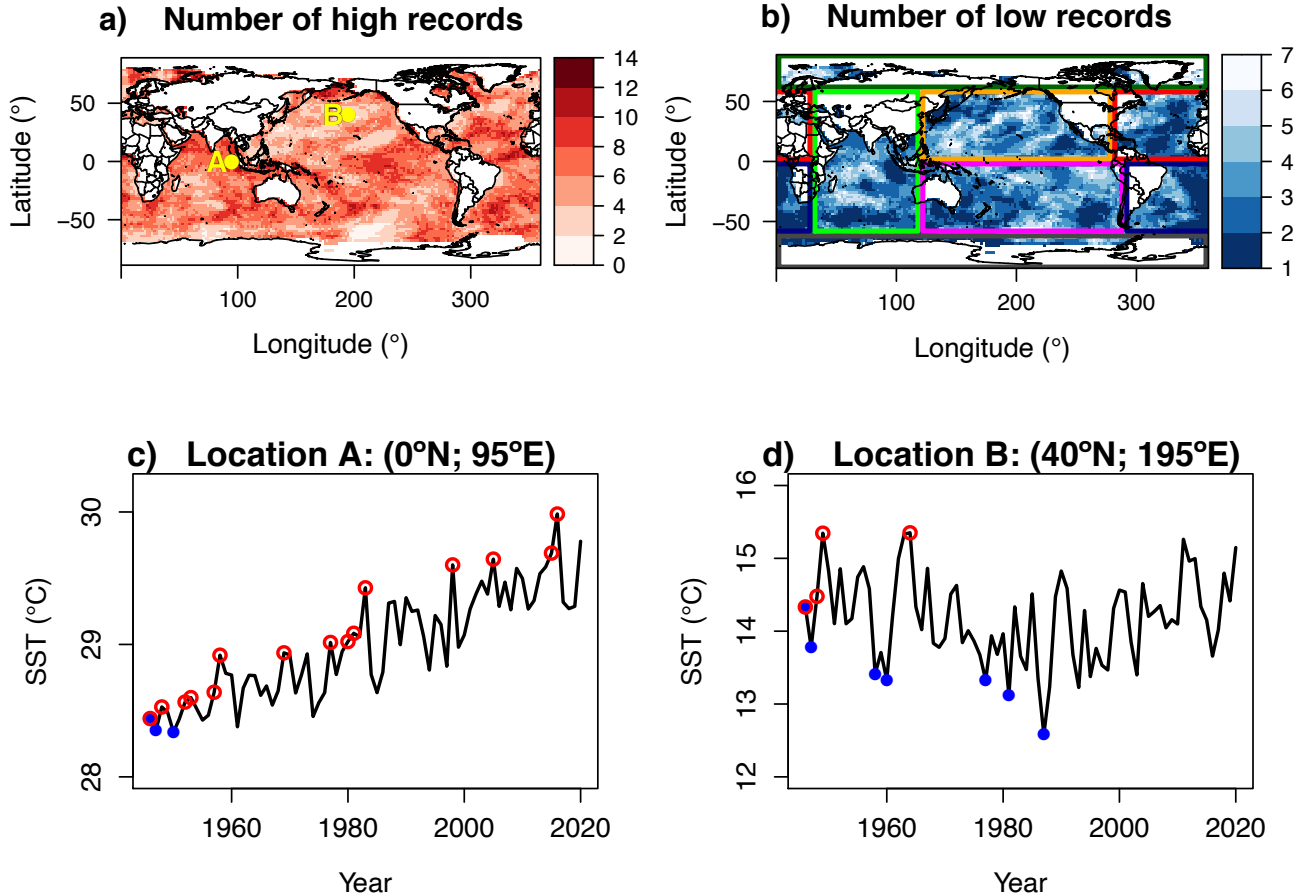
455 Figure 1: Number of observed high (a) and low (b) records of SST for the p 1946 to 2020 period. Panels (c) and (d) show samples of time series of annual SST for two pixels, marked by yellow dots on panel (a): points A (0°N; 95°E) and B (40°N; 195°E), high/low records are marked by red/blue dots on the time series. Location A shows a clear increasing trend, with high records exceeding the low ones, while at location B, the opposite holds. The asymmetry between the number of high and low records and their deviation from the expected value for a TFRV were used to quantify trends and their significance in each 460 pixel's time series. The boxes in (b) divide the global oceans for subsequent analysis: Antarctic (ANT - gray), Arctic (ARC - dark green), Indian (IND - green), North Pacific (NP - orange), South Pacific (SP - magenta), North Atlantic (NA - red), and South Atlantic (SA - navy blue).
