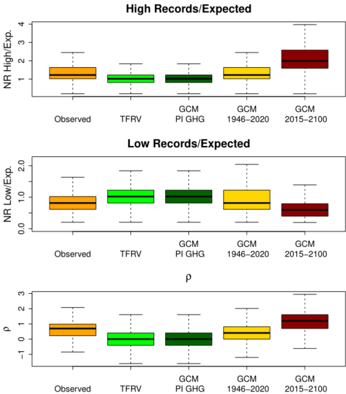
Figure 6: Boxplots of the ratio of the number of high and low records over the expected value and of \rho for the observed SST between 1946-2020, Monte Carlo simulation of a TRFV, modelled SST of the PI control run samples, modelled SST between 1946-2020, projected SST between 2015-2100 (using the SSP2-4.5 scenario). The simulations were from the MRI-ESM2-0 CMIP6 global climate model.
