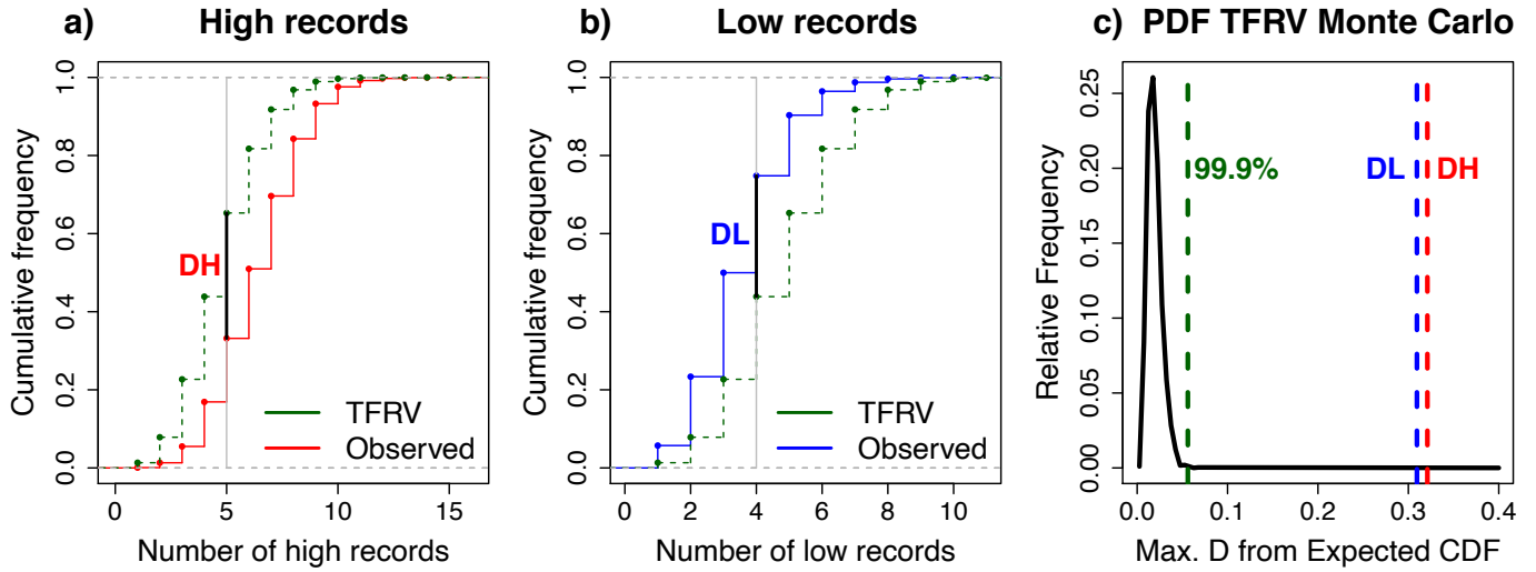
505 Figure 4: Cumulative distribution functions (CDFs) of the theoretical TFRV number of records from Eq. (34) (in green) and number of observed high (red) (a), and low (blue) (b) records. The Kolmogorov-Smirnov test was applied to the distributions, and the maximum distances, DH and DL, were obtained for the high and low records, respectively (black vertical lines). NoticeNote that the exact theoretical (discrete and integer-valued) distribution of the number of records of a TFRV time series of length 75, given by Eq. (43), was used, and it is a discrete distribution (since the number of records in a time series is an 510 integer > 0 ). The probability distribution function of the maximum distance D for Monte Carlo simulations of the number of records of TFRV (c) was used to assess the significance of the results. The 99.9% percentile and the maximum deviations, DH and DL, are shown in green, red, and blue dashed lines, respectively. Both DH and DL are far above the 99.9% percentile, demonstrating the high statistical significance of SST global trends in high and low records.
