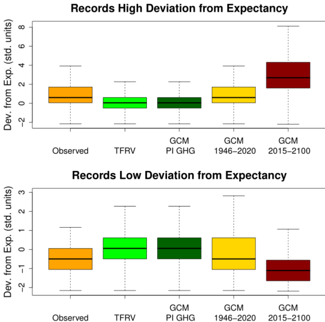
Figure 7: Boxplots of the high and low deviation from expected number for: observed SST between 1946-2020, TRFV, modelled SST of the PI control run samples, modelled SST between 1946-2020, projected SST between 2015-2100 (using the SSP2-4.5 scenario). The simulations were from the MRI-ESM2-0 CMIP6 global climate model.
