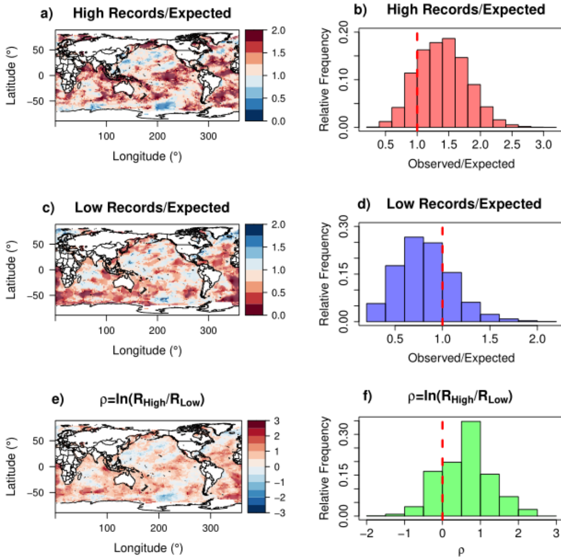
Figure 2: Number of observed high (a) and low (c) records of SST over the expected value for a TFRV in a 75-years time series. The trend indicator \rho , given by quantifies the asymmetry between the number of high and low records, \rho = \ln(R_{\text{High}}/R_{\text{Low}}) (e), and their respective distributions for the whole globe (b, d, f) are presented. The red dashed lines mark the thresholds where observed records exceed the expected value in (b) and (d) or when the number of high records is larger than the low records in (f). These three different indicators metrics combined can be used to efficiently simply and robustly detect trends in noisy time series. The asymmetry between high and low records is evident, with a large number of high records and a small number of low records over most of the globe, particularly in the tropical and subtropical Atlantic, the Central Pacific, the eastern Indian Ocean, and the Southern sea. Note that, although the overwhelming majority of the ocean is warming, some islands of consistent persistent cooling are observed in the maps.
