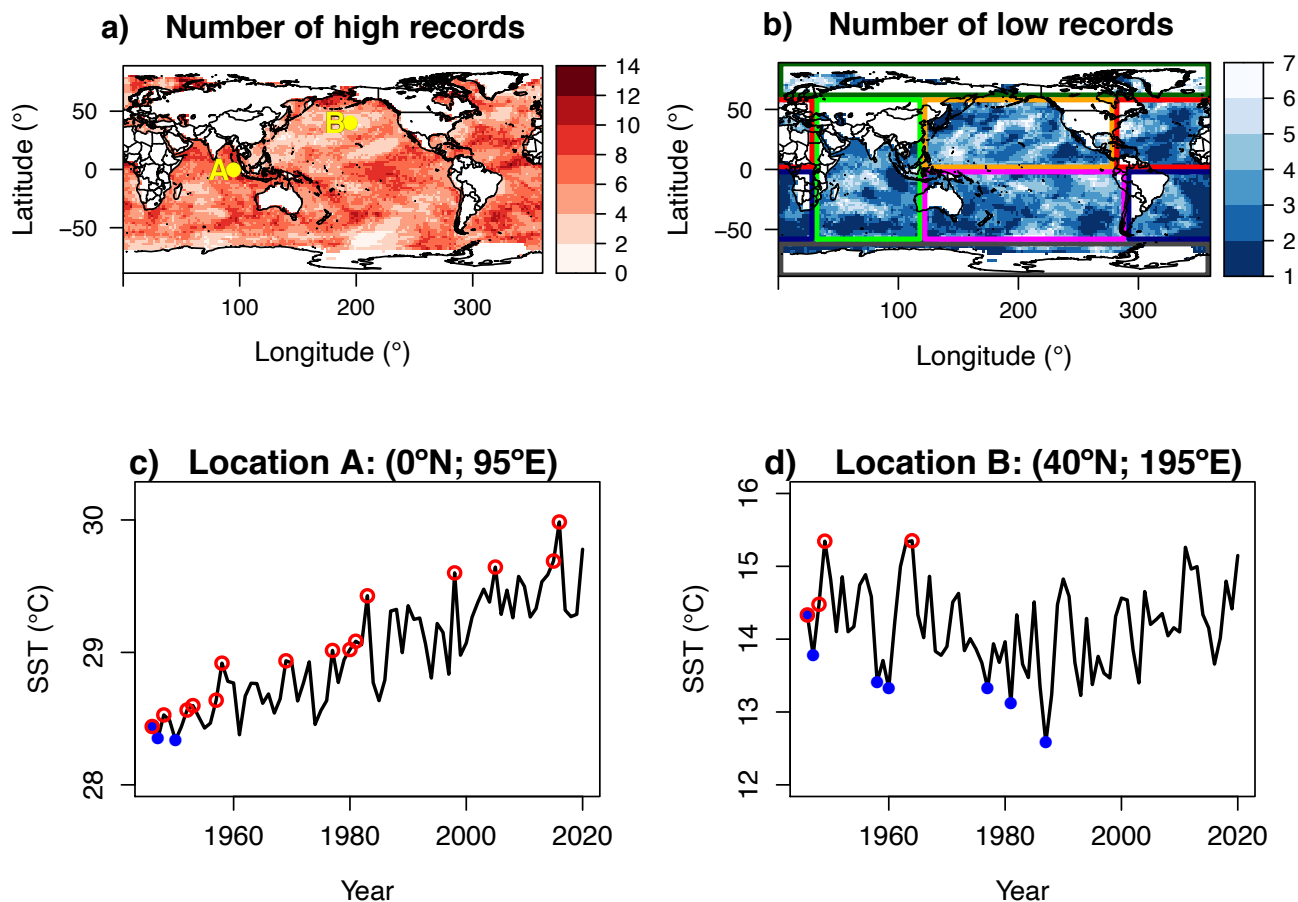
Figure 1: Number of observed high (a) and low (b) records of SST for the period-between 1946 to 2020 period . Panels (c) and (d) show examplesamples of time series of annual SST for two pixels, marked by yellow dots on panel (a): points A (0°N; 95°E) and B (40°N; 195°E), high/low records are marked by red/blue dots on the time series. Location A shows a clear increasing trend, with high records exceeding the low ones, while at location B, the opposite holds. The asymmetry between the number of high and low records and their deviation from the expected value for a TFRV were used to identifyquantify trends and their significance in each pixel's time series. The boxes in (b) divide the global oceans for subsequent analysis: Antarctic (ANT - gray), Arctic (ARC - dark green), Indian (IND - green), North Pacific (NP - orange), South Pacific (SP - magenta), North Atlantic (NA - red), and South Atlantic (SA - navy blue).
