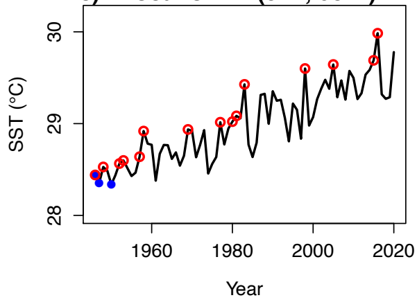
c) Location A: (0°N; 95°E)
