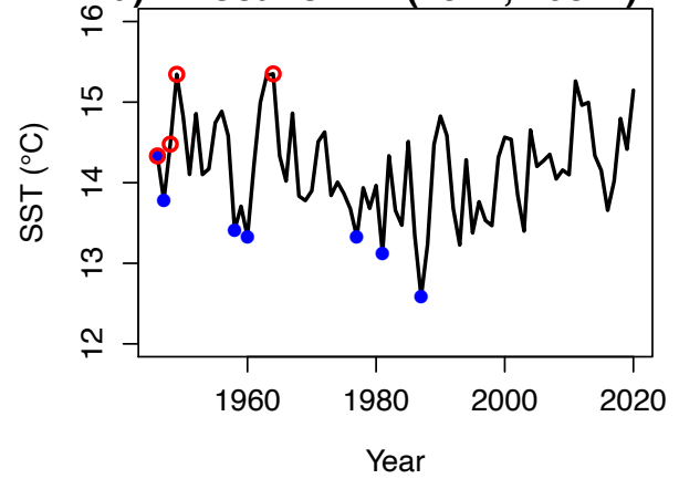
d) Location B: (40°N; 195°E)
