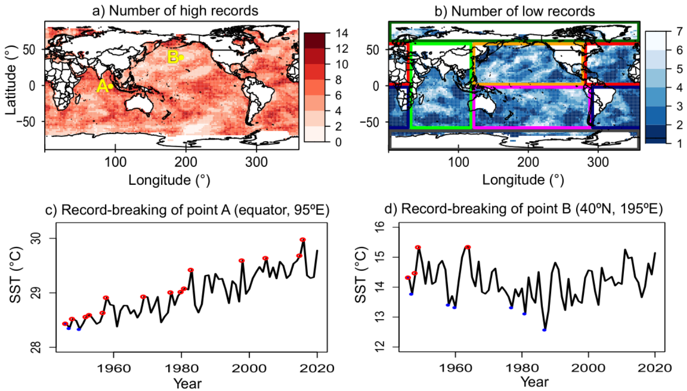
495 Figure 1: Number of observed high (a) and low (b) records of SST for the p 1946 to 2020 period. Panels (c) and (d) show 500 samples of time series of annual SST for two pixels, marked by yellow dots on panel (a): points A ( 0^{\circ}\text{N} ; 95^{\circ}\text{E} ) and B ( 40^{\circ}\text{N} ; 195^{\circ}\text{E} ), high/low records are marked by red/blue dots on the time series. Location A shows a clear increasing trend, with high records exceeding the low ones, while at location B, the opposite holds. The asymmetry between the number of high and low records and their deviation from the expected value for a TFRV were used to quantify trends and their significance in each pixel's time series. The boxes in (b) divide the global oceans for subsequent analysis: Antarctic (ANT - gray), Arctic (ARC - dark green), Indian (IND - green), North Pacific (NP - orange), South Pacific (SP - magenta), North Atlantic (NA - red), and South Atlantic (SA - navy blue).
