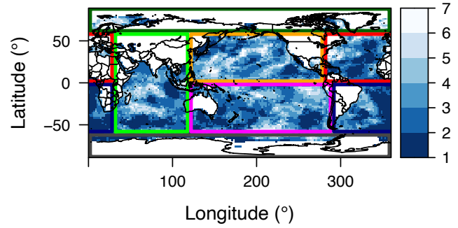
b) Number of low records
