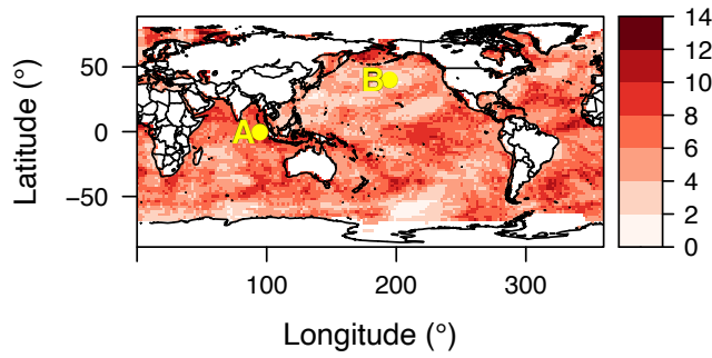
a) Number of high records
