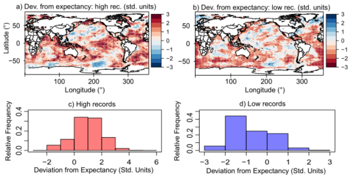
550 Figure 5: Departure of the observed number of high (a) and low (b) records from expectation, in units of standard deviation, and their frequency distributions (c and d). In 15.8% of the pixels, the number of high records exceeds 2 standard deviations above expectation. This value is ~12 times larger than TFRV. Large deviations are observed over all the oceans for high records and predominantly in the Arctic and Atlantic Oceans for low records.
