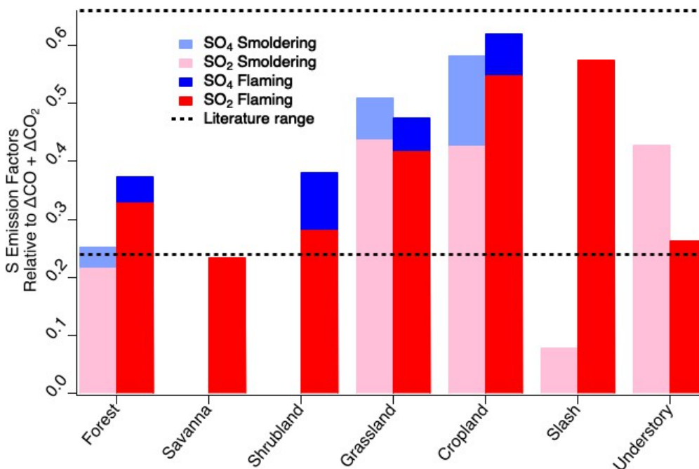
375 Figure 2. Elemental sulfur emission factors of SO 2 and sulfate by fuel type and combustion stage 380 within 1 hr downwind compared to literature values of total sulfur emission factors.
