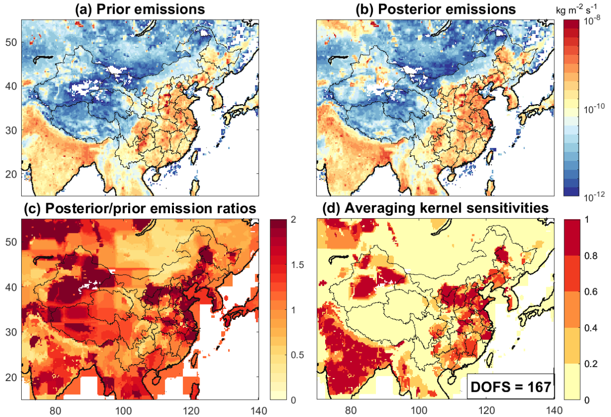
Figure 4. Optimization of methane emissions over East Asia in 2019 from inversion of TROPOMI observations. Results are from the base inversion and are shown on the 0.25^\circ \times 0.3125^\circ grid. (a) Prior estimates of methane emissions, summing the contributions from the sectors in Fig. 3 plus additional minor sectors as given in Table 1. (b) Posterior methane emissions from the TROPOMI inversion. (c) Posterior/prior emission ratios. (d) Averaging kernel sensitivities. The averaging kernel sensitivities are the diagonal elements of the averaging kernel matrix and display the ability of the observations to quantify emissions independently from the prior estimates (1 = fully, 0 = not at all). The degrees of freedom for signal (DOFS, defined as the trace of the averaging kernel matrix) is given inset.
