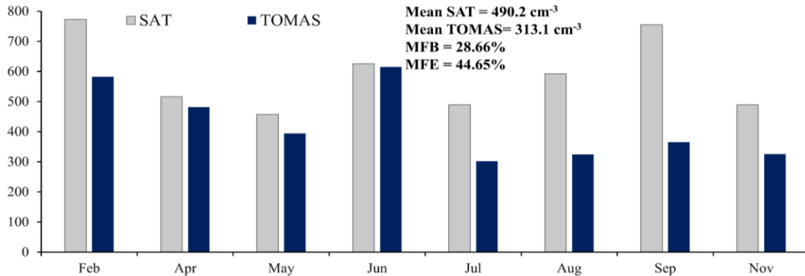
26 Figure S45. Monthly mean simulated CCN concentrations (TOMAS) from XG simulation and satellite-retrieved CCN 27 concentrations (SAT) from Liu et al., (2020). The mean satellite-retrieved (Mean SAT) CCN concentrations, mean 28 simulation (Mean TOMAS), mean fractional error (MFE), and mean fractional bias (MFB) displayed at upper centre 29 are the statistic result of averaged on the simulation grid for corresponding satellite-retrieved CCN geographical 30 location (in total 667 grids).
