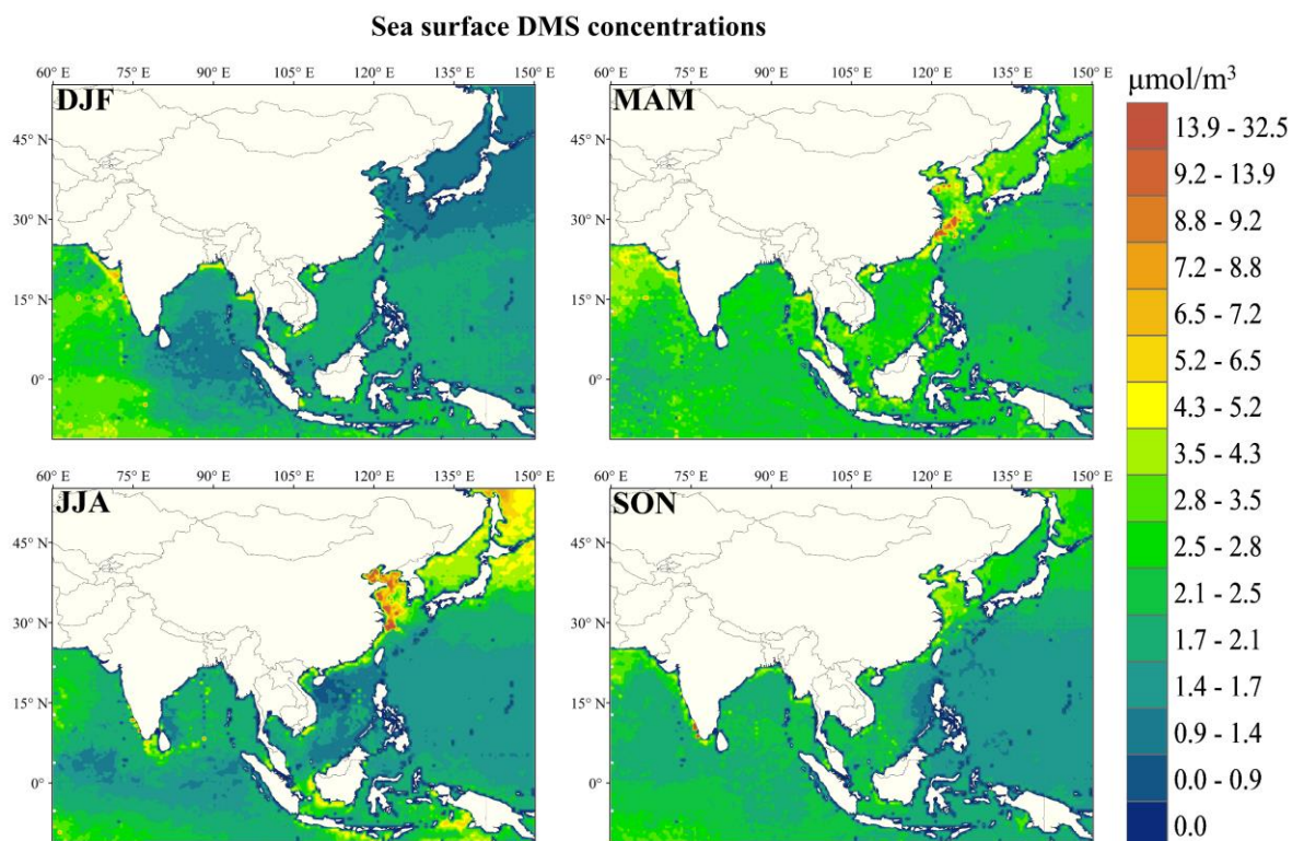
730 Figure 2. Sea-surface DMS concentrations predicted by XGBoost model by season.
