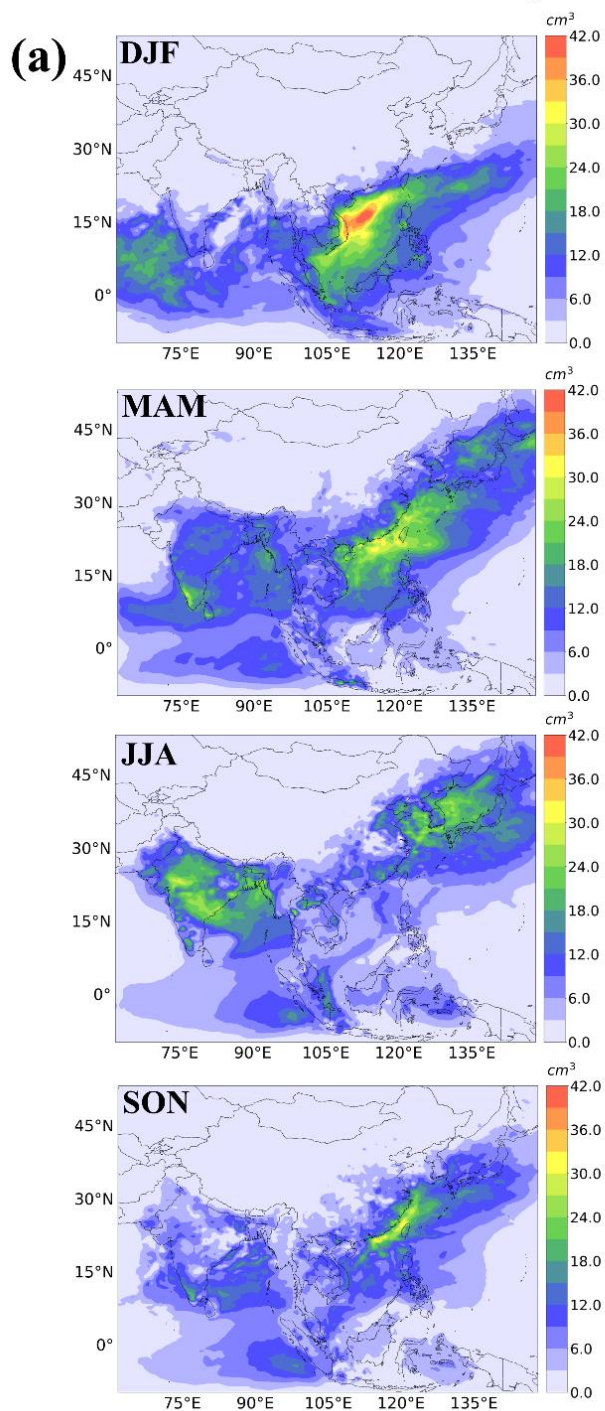
745 Figure 6. Spatial pattern of the seasonal mean absolute changes in surface \text{SO}_4^{2-} (first column) and all-sky DRF (second column) between the XG and ND (no DMS) simulations.
