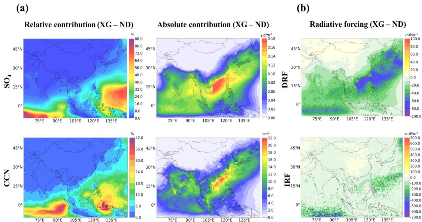
Figure 8. Panel (a) presents the spatial distributions of annual mean percent changes and absolute changes in surface SO 4 2- and CCN, and panel (b) presents the spatial distributions of annual mean all-sky DRF and cloud-albedo IRF between XG and ND (no DMS) simulations.
