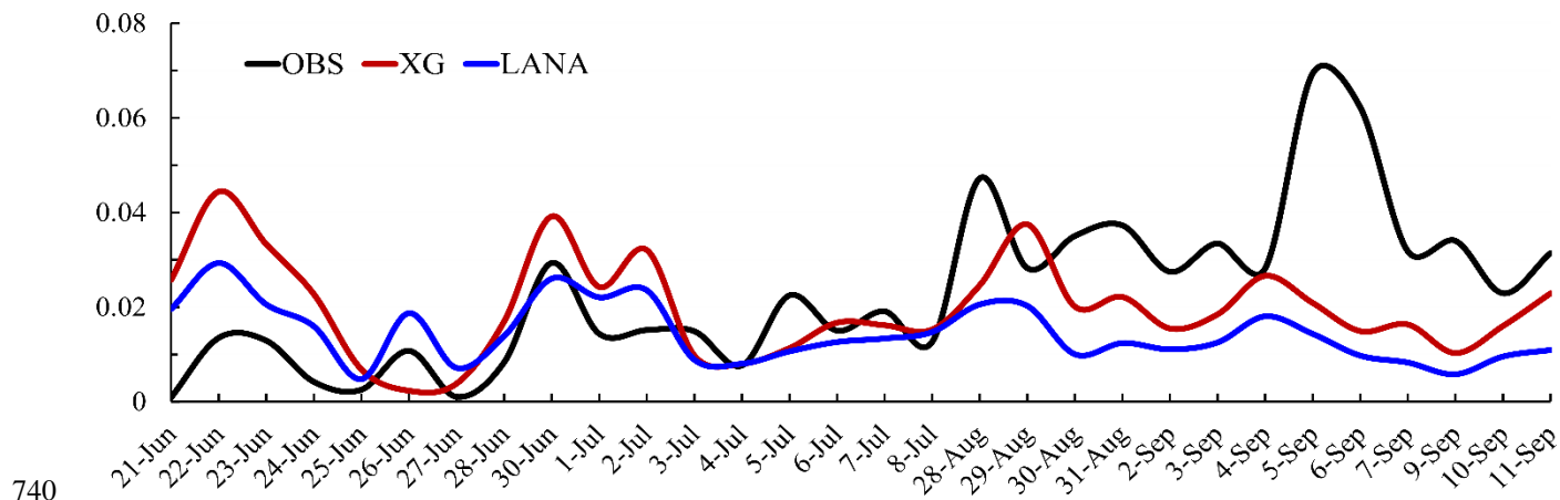
Figure 5. A comparison of simulated daily concentrations of MSA with observations at the Hua Niao Island site (Units: \mu\text{g m}^{-3} ).
