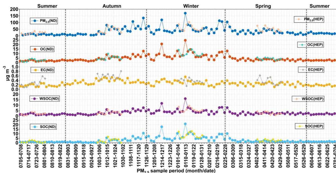
Figure 4. Temporal variations in concentration ( \mu\text{g m}^{-3} ) of PM 2.5 and its chemical components: OC, EC, WSOC and SOC, at ND (solid dots) and HEP (solid star shape) in Tianjin during 2018-2019. See text for abbreviations.
