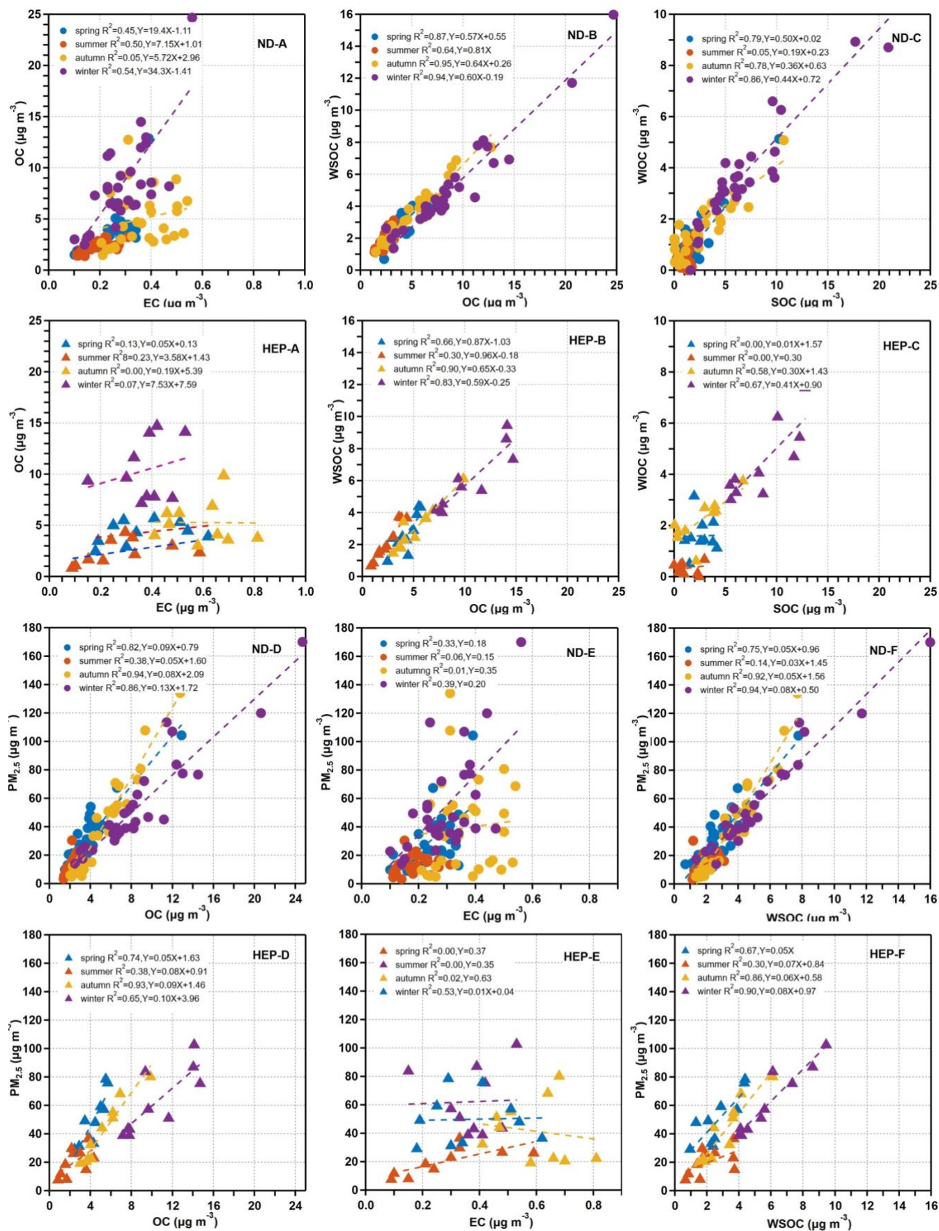
395 Figure 5. Scatter plots of selected carbonaceous components in PM_{2.5} in Tianjin at ND and HEP.
