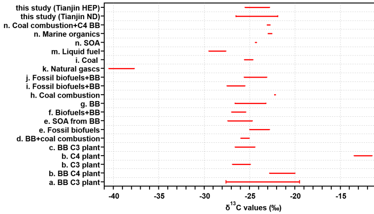
Figure 11. Range or mean \delta^{13}C_{TC} in the particles emitted from point sources, source substance, and atmospheric aerosols from different sites around the world. a Fang Cao et al. (2016); b Martinelli et al. (2002); c Junwei Song et al. (2018); d Garbaras et al. (2015); e Bikkina et al. (2016); f Aggarwal et al. (2013); g Pingqing Fu et al. (2012); h Kunwar et al. (2016); i Cachier et al. (1986); j Pavuluri et al. (2016); k; l; m Widory et al. (2006); n Kundu et al. (2014).
