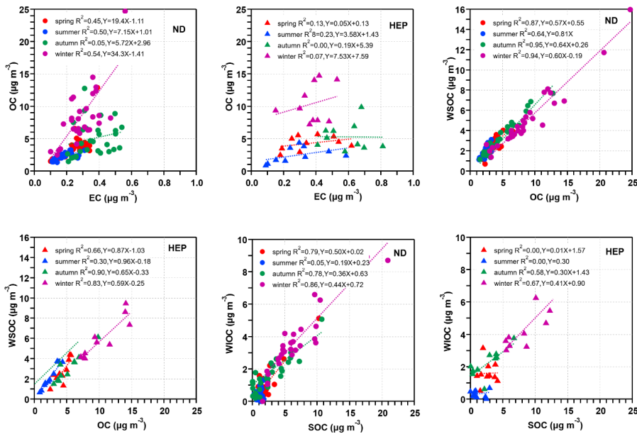
Figure 6. Scatter plots of selected carbonaceous components in PM 2.5 in Tianjin at ND and HEP.
