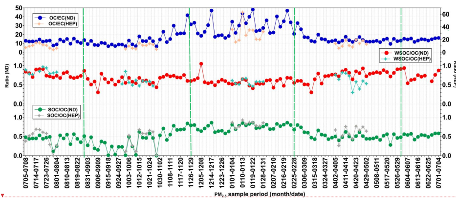
Figure 5. Temporal variations in the ratios of OC/EC, WSOC/OC, and SOC/OC in \text{PM}_{2.5} at ND (solid dots) and HEP (hollow small ball) in Tianjin during 2018-2019. See text for abbreviations.
