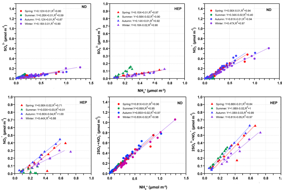
Figure 8. Linear relations between secondary ions in PM 2.5 at ND (solid dots) and HEP (solid triangles) in Tianjin during the campaign period.
