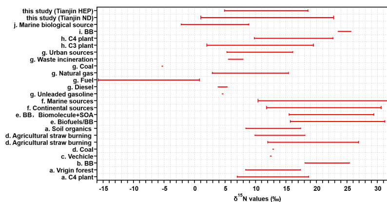
Figure J2. Range or mean \delta^{15}\text{N}_{\text{TN}} in the particles emitted from point sources, source substance, and atmospheric aerosols from different sites around the world. a Martinelli et al. (2002); b Aggarwal et al. (2013); c Kunwar et al. (2016); d Kundu et al. (2010); e Pavuluri et al. (2010); f Bikkina et al. (2016); g Widory et al. (2007); h Turekian et al. (1998); i Kundu et al. (2010); j Miyazaki et al. (2011).
