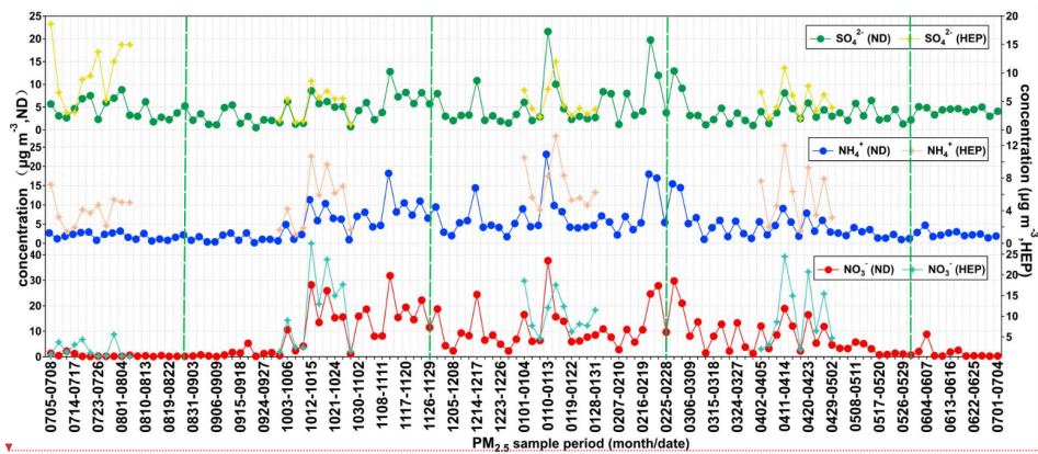
Figure 7. Temporal variations in concentrations ( \mu\text{g m}^{-3} ) of secondary ionic species in \text{PM}_{2.5} at ND and HEP in Tianjin during the campaign period (2018-2019).
