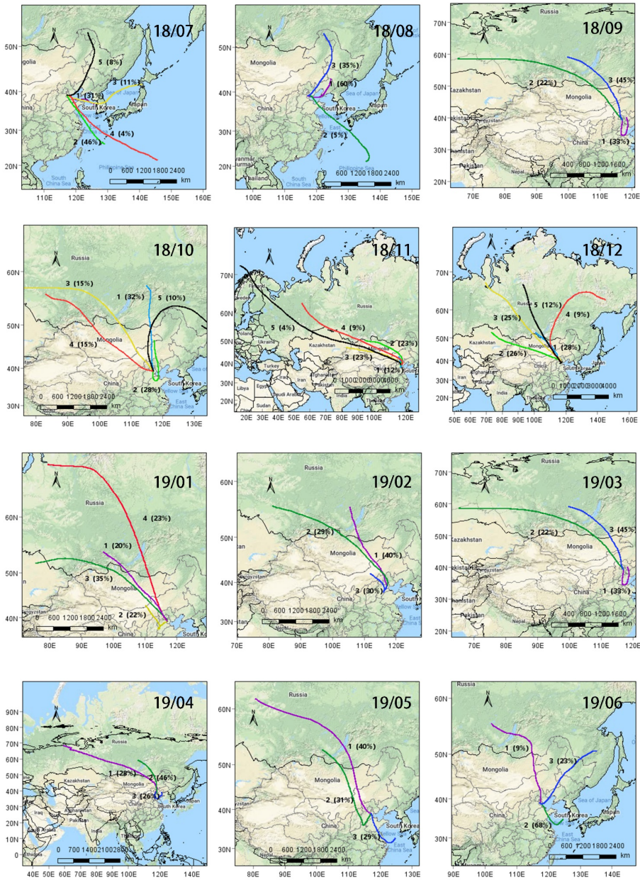
310 Figure 3. Monthly cluster analysis plots of 5-day backward air mass trajectories arriving over Tianjin at 500 m above the ground level during the campaign period. (The maps were generated by the MeteInfo software using the © Google Maps)
