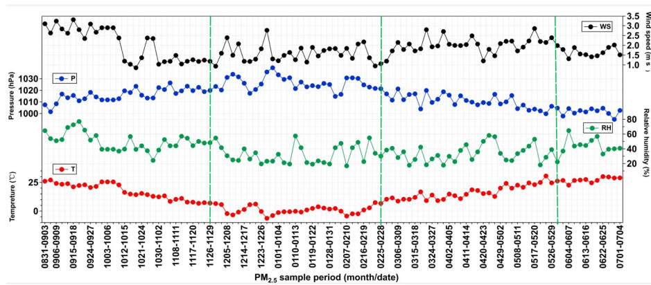
280 Figure 2. Temporal variations of ambient temperature (T), atmospheric pressure (P), wind speed (WS) and relative humidity (RH) at Tianjin from September 2018 to July 2019.
