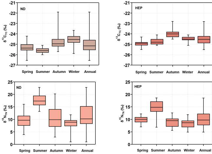
Figure 10. Box-and-whisker plot of seasonal variations in stable carbon isotope ratios of total carbon ( \delta^{13}C_{TC} ) and nitrogen ( \delta^{15}N_{TN} ) in PM_{2.5} at ND and HEP in Tianjin during the campaign. The cross bar in the box show the median and open circles show the outliers.
