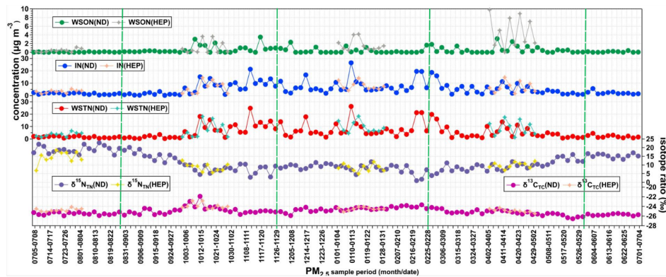
Figure 9. Temporal variations in WSTN, IN, WSON ( \mu\text{g m}^{-3} ) and \delta^{13}\text{C}_{\text{TC}} , \delta^{15}\text{N}_{\text{TN}} in \text{PM}_{2.5} at ND (solid dots) and HEP (solid stars) in Tianjin during the campaign period (2018-2019).
