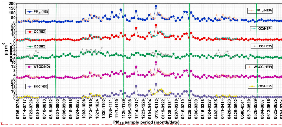
Figure 4. Temporal variations in concentration ( \mu\text{g m}^{-3} ) of \text{PM}_{2.5} and its chemical components: OC, EC, WSOC and SOC, at ND (solid dots) and HEP (solid star shape) in Tianjin during 2018-2019. See text for abbreviations.
