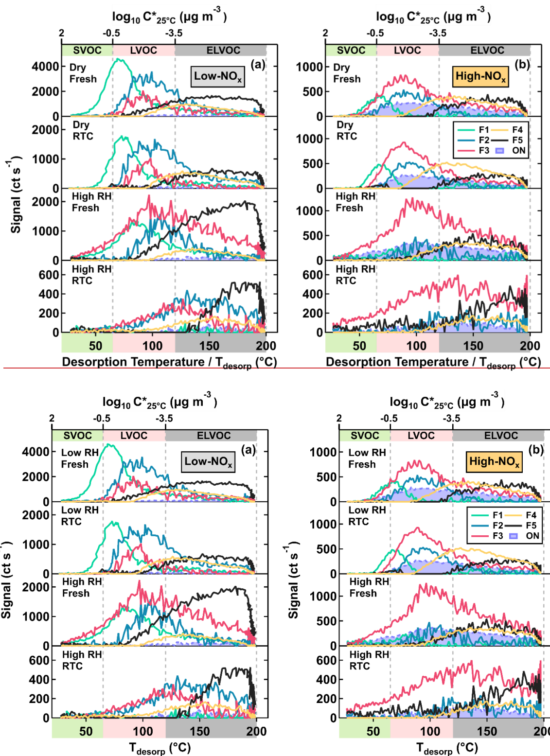
Figure 3. Factor thermograms of the five sample factors from the 12-factor PMF solution of non-nitrated organics CHO compounds in \alpha -pinene SOA particles that were formed under low- \text{NO}_x (a) and high- \text{NO}_x (b) conditions in the OFR . In addition, thermograms of organic nitrates the sum of ON (sum of NF1 – 3) are shown as purple areas in panel (b). In both panels, the ranges of different volatility classes are highlighted as color bands on the abscissa.
