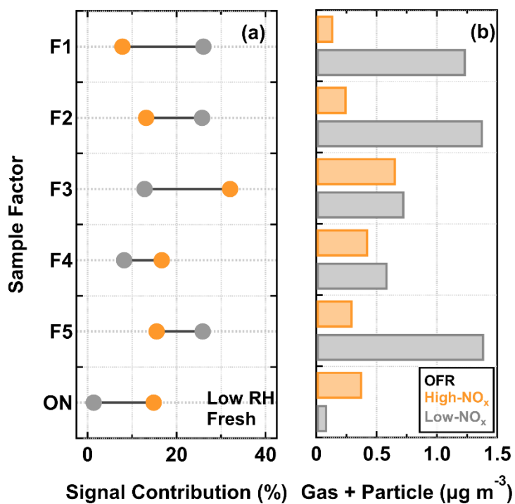
Figure 6. Signal contributions of sample factors to their total sum (a) and the corresponding estimated mass concentrations in gas and particle phase (b) for dry, fresh- \alpha -pinene SOA particles that were formed under low-NO x and high-NO x conditions in the OFR and evaporated under low-RH and fresh condition . Note that here ON indicates the sum of the organic nitrate -ON sample factors. The fraction is calculated by normalizing the measured sum from a PMF sample factor to the total sum of sample factors in the dry/low-RH , fresh samples under low-NO x and high-NO x conditions.
