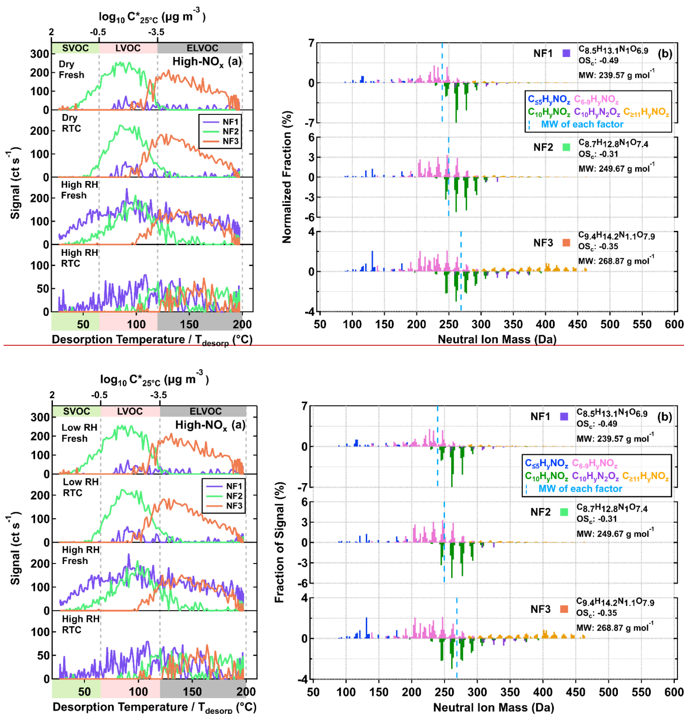
Figure 5. Factor thermograms (a) and normalized mass spectra (b) for the three sample factors from the eight-factor solution of organic nitrates-ON in the \alpha -pinene SOA particles that were formed under high-NO x conditions in the OFR . In panel (a), the ranges of different volatility classes are indicated in color bands on the abscissa. In panel (b), the bottom portion of each mass spectra represents C 10 H y NO z . The the signal-weighted molecular composition, molecular weight (MW), and oxidation state (OS c ) for each factor are shown on the right. Right next to each factor label in panel (b), the squares are shown in the same color scheme as the factor thermograms in panel (a) to identify different sample factors. The blue dashed line indicates the average MW of each factor.
