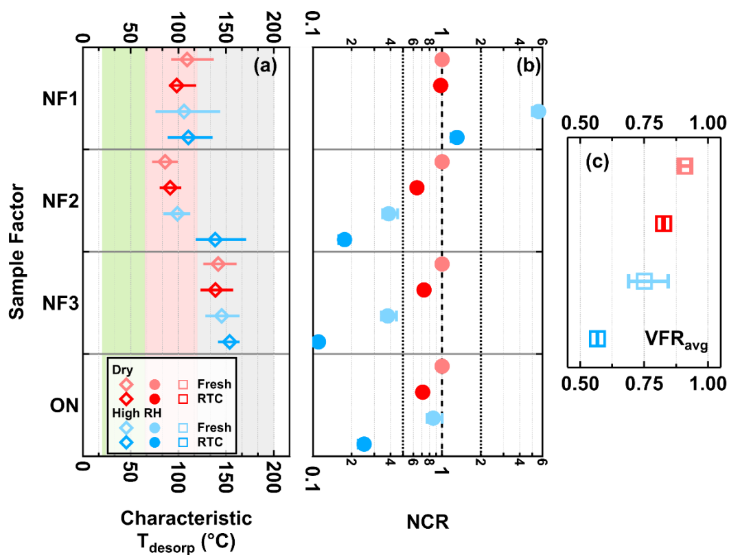
Figure 8. Volatility and changes in factor contribution for the three organic nitrate sample factors and total organic nitrates (ON, sum of organic nitrate sample factors). Panel (a): Characteristic desorption temperature (characteristic T_{desorp} ). The marker indicates the T_{50} values, and the horizontal lines mark the interquartile range of the factor thermograms. Panel (b): Net change ratio (NCR) with error bars indicating the uncertainty stemming from the estimated range in molecular weight and particle density. Panel (c): average volume fraction remaining during sample collection ( VFR_{avg} ) with error bars indicating the minimum and maximum values. The colors indicate the sample type. In panel (a), the range of volatility classes are highlighted with background colors (green—SVOCs; red—LVOCs; grey—ELVOCs). In panel (b), the dashed line at NCR equal to 1 indicates that any loss is counterbalanced by production, or no change occurs. The two dotted lines at NCR equal to 0.5 and 2 represent significant net loss and production.
