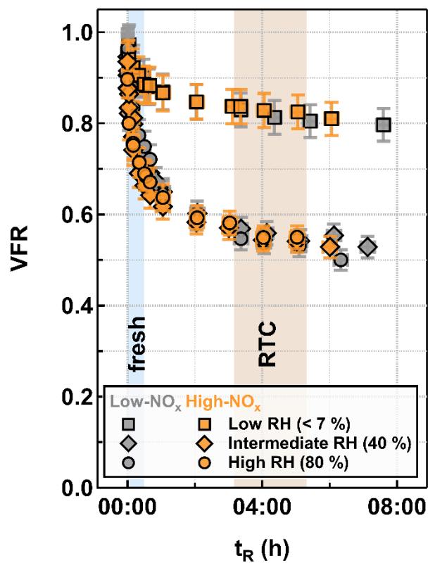
Figure 1. Evapograms-Volume Fraction Remaining (VFR) derived from particle size measurements for as function of residence time ( t_R ) in the RTC low \text{NO}_x (grey) and high \text{NO}_x (orange) cases for \alpha -pinene SOA particles which were formed under low- \text{NO}_x (grey) and high- \text{NO}_x (orange) conditions in the OFR and evaporated under dry-low-RH (< 7 %, squares), intermediate-intermediate-RH (40 % RH, diamonds) and high-high-RH (80 % RH, circles) conditions. The blue and brown areas indicate the collection periods of FIGAERO-CIMS corresponding to fresh and RTC samples.
