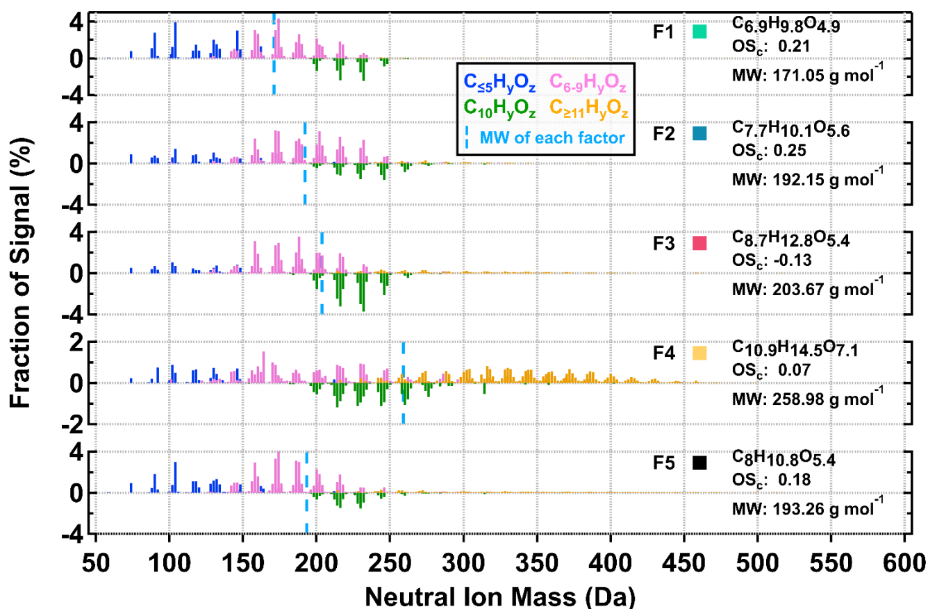
Figure 4. Normalized factor mass spectra of the five sample factors from the 12-factor PMF solution of non-nitrated organics CHO compounds in \alpha -pinene SOA particles that were formed under two NO x conditions in the OFR . For readability,
