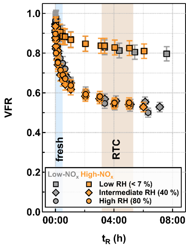
Figure 11. Evapograms—Volume Fraction Remaining (VFR) derived from particle size measurements for \alpha -pinene SOA particles which were formed under low- \text{NO}_x (grey) and high- \text{NO}_x (orange) conditions in the OFR and evaporated under dry-low-RH (< 7 %, squares), intermediate-intermediate-RH (40 % RH, diamonds) and high-high-RH (80 % RH, circles) conditions. The blue and brown areas indicate the collection periods of FIGAERO-CIMS corresponding to fresh and RTC samples.
