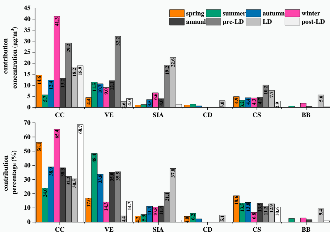
Figure 7. (a) Concentration and (b) percentage of source contribution to PM 2.5 in Hohhot in spring, summer, autumn, winter, and over the sampling year, pre-lockdown, lockdown, and post-lockdown periods . CC, VE, SIA, CD, CS, and BB represent coal combustion, vehicular emission, secondary inorganic aerosol, construction dust, crustal sources, and biomass burning, respectively.
