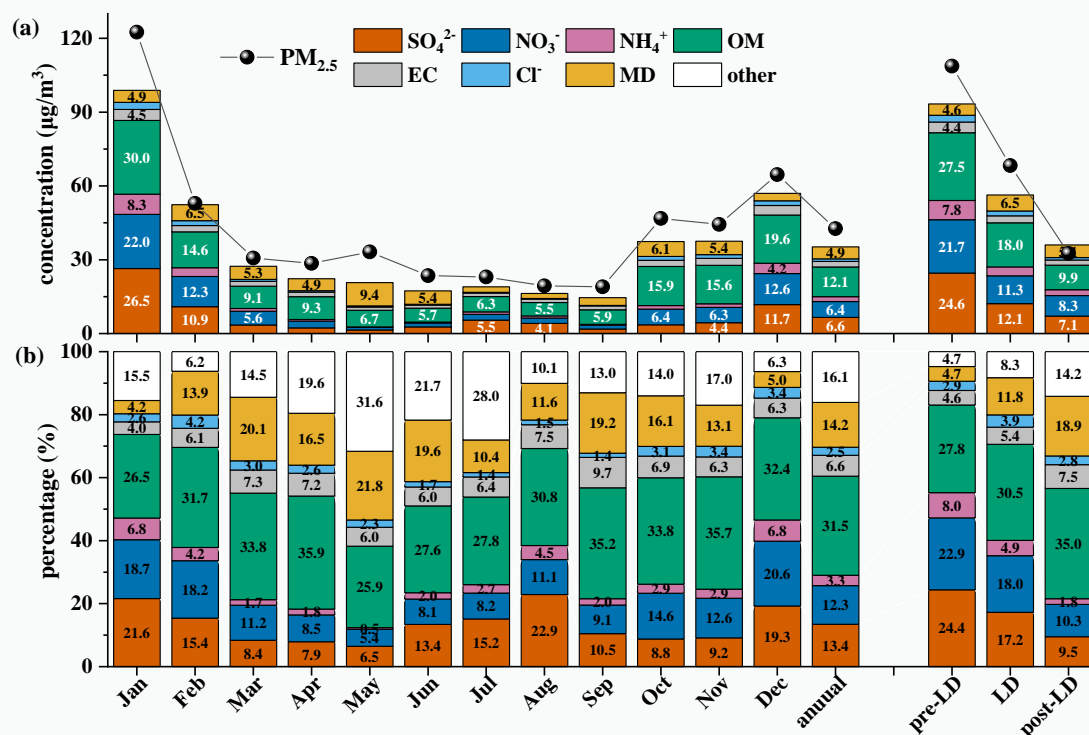
Figure 4. Monthly variation in (a) concentrations and (b) percentages of chemical components of \text{PM}_{2.5} in Hohhot during the sampling period. Pre-LD, LD, and post-LD represent the pre-lockdown, lockdown, and post-lockdown periods, respectively. OM and MD represent organic matter and mineral dust, respectively.
