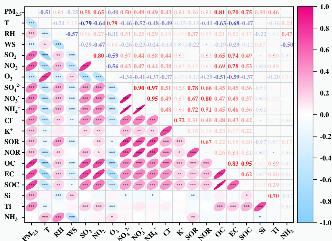
330 Figure 6. Correlation between chemical components of PM 2.5 , metrological-meteorological variables, SOR, NOR, and air pollutants in Hohhot during the sampling period (* p < 0.05 , ** p < 0.01 , *** p < 0.001 ).
