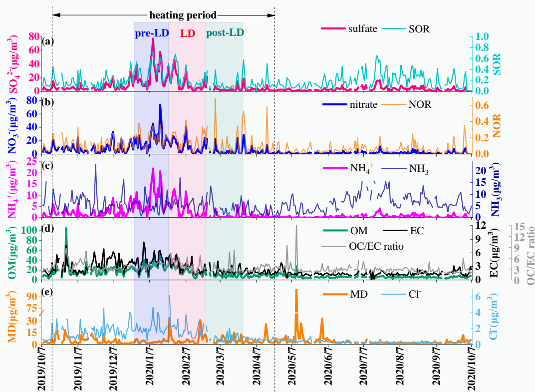
Figure 3. Daily variations in chemical composition of PM 2.5 , SOR, NOR, NH 3 , and OC/EC ratio in Hohhot during the sampling period. The blue, red, and green background represent the pre-lockdown, lockdown, and post-lockdown periods, respectively.
