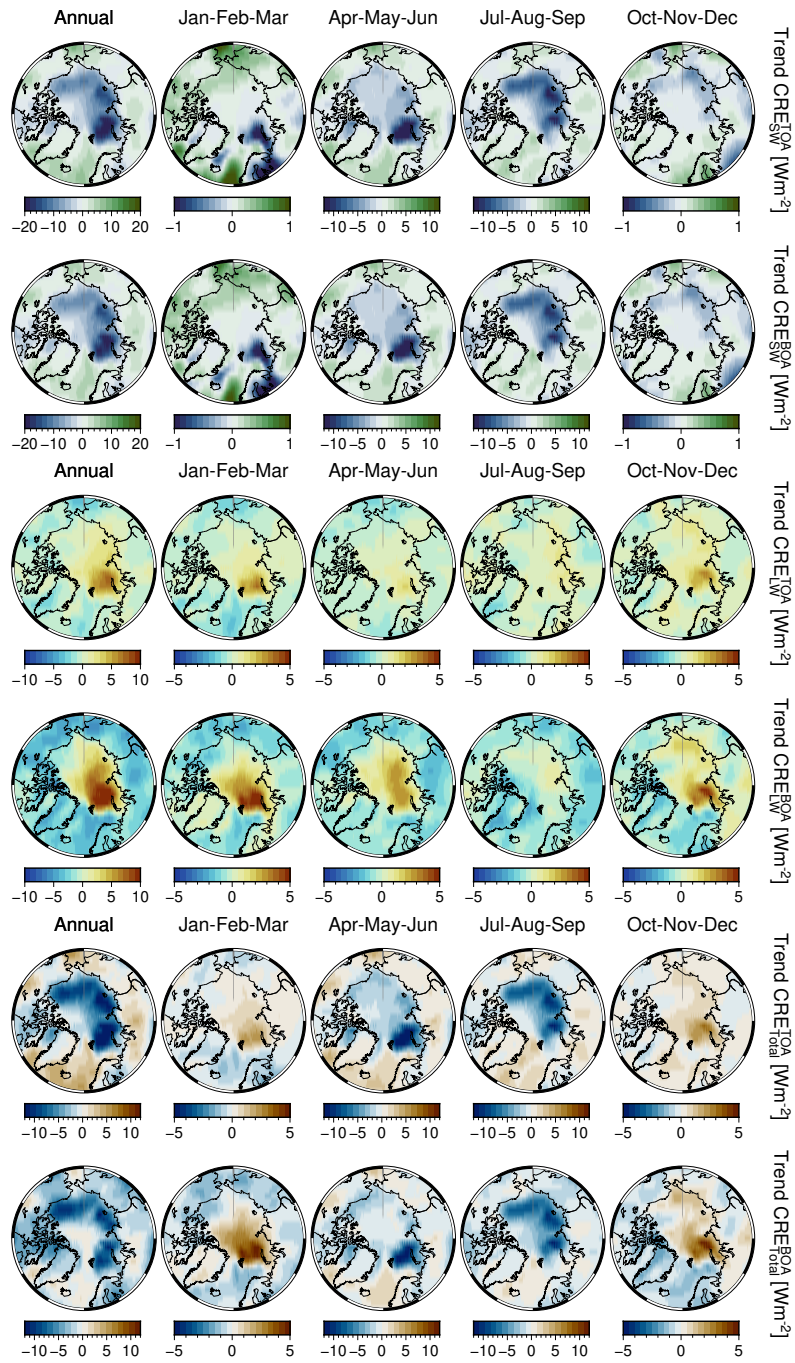
Figure C2. From left to right, annual and seasonal trends of SW (rows 1-2), LW (3-4), and total (5-6) cloud radiative forcing (CRF, \text{W m}^{-2} ) at TOA and BOA.
