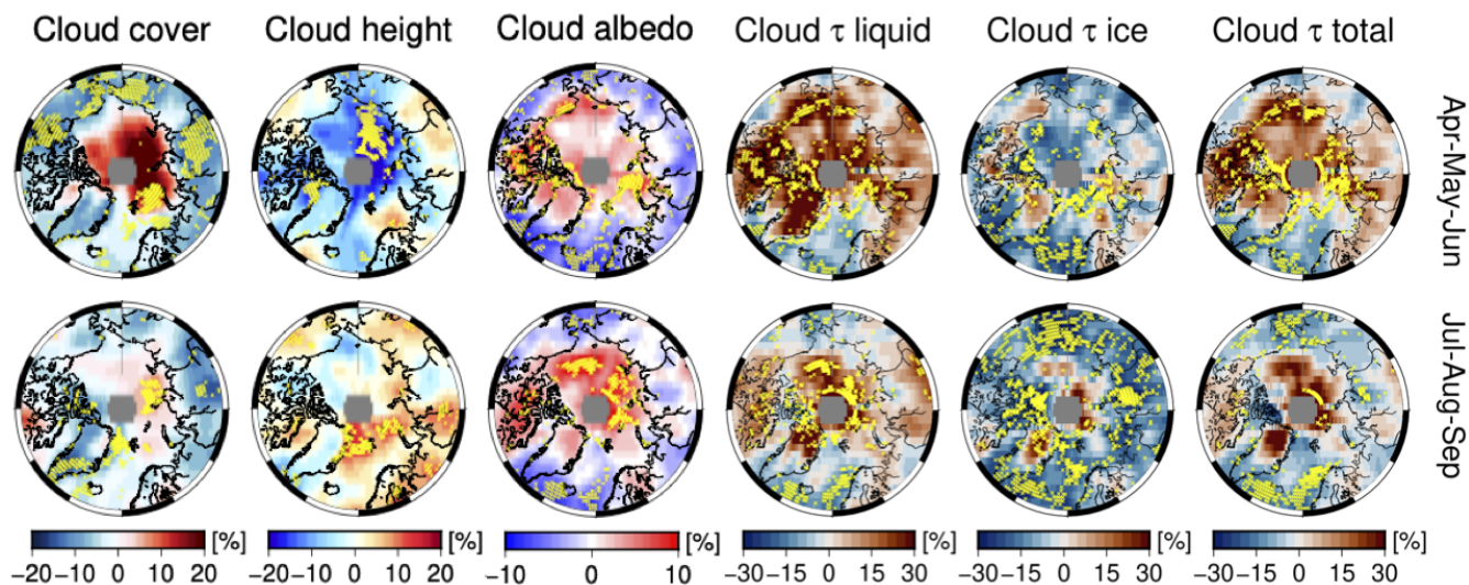
Figure 9. For cloud cover (CFC), height (CTH), cloud albedo (CA) at 600 nm, optical thickness (COT, \tau ) of all, liquid and ice clouds, the panels show their seasonal breakdown. The trend values in % are relative to the property value at the start year (1996) in the record. Stippling in yellow indicates statistical significance at 95% confidence.
