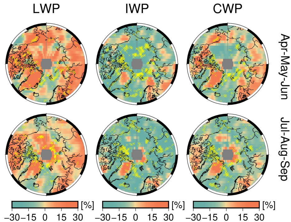
Fig. 11: Seasonal trends of LWP, IWP and CWP.
