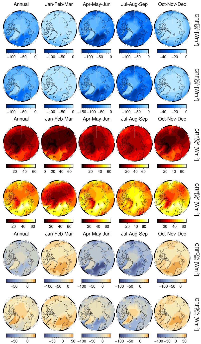
Fig. 10: From left to right, annual and seasonal average values of SW (rows 1-2), LW (3-4) and total (5-6) cloud radiative forcing (CRF, \text{W m}^{-2} ) at TOA and BOA, respectively. Note the different color scales to match the CRF ranges.
