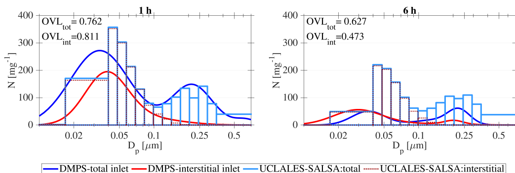
Figure 12. Comparison of aerosol size distributions calculated with UCLALES-SALSA at Puijo altitude of 225 m and measured by the Twin-inlet DMPS system during Case 2 31 October 2020
