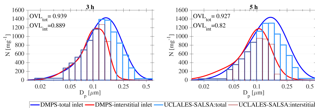
Figure 6. Comparison of aerosol size distributions calculated with UCLALES-SALSA at Puijo altitude of 225 m and measured the Twin-inlet DMPS system during Case 1 24 September 2020.
