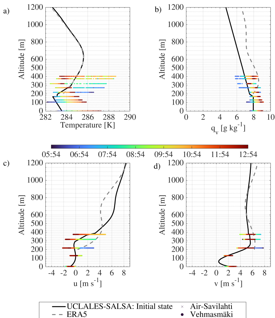
Figure 1. Vertical profiles used to initialize the simulation of Case 1, diurnal cloud event of 24 September 2020 starting at 07:54 (UTC+2:00). a) Potential temperature b) Specific humidity c) u-component d) v-component of the horizontal wind velocity. Each panel also shows local surface observational data from the Savilahti station, local vertical profiles observed at the Vehmasmäki station and re-analyzed data from ECMWF-ERA5
