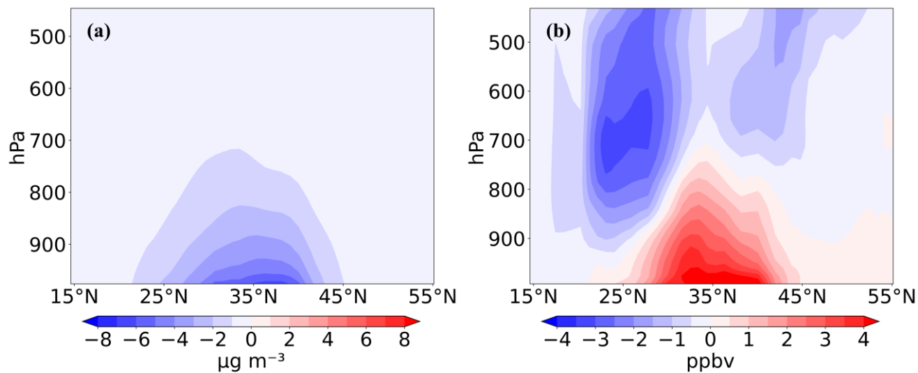
Figure 3. Pressure–latitude cross-section averaged over 110–125.5°E for differences in simulated annual mean (a) PM 2.5 (μg m -3 ) and (b) O 3 (ppbv) concentrations due to emission reductions of aerosol pollutants between 2013 and 2017 (2017 minus 2013). Modelled PM 2.5 data are from CESM2 simulations and modelled O 3 data are from GEOS-Chem simulations.
