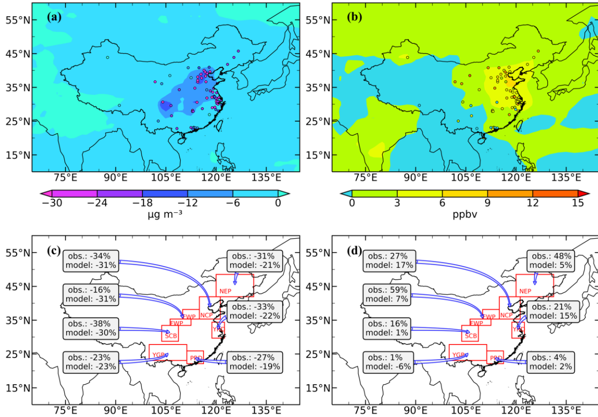
Figure 2. Spatial distributions of differences in observed (obs., circles) and simulated (model, shades) annual mean near-surface (a) PM 2.5 (μg m -3 ) and (b) O 3 (ppbv) concentrations over China between 2013 and 2017 (2017–2013) and (c, d) the percentage changes averaged over seven sub-regions of China, including the North China Plain (NCP, 35°N–41°N, 114°E–120°E), Sichuan Basin (SCB, 28°N–33°N, 103°E–108°E), Yangtze River Delta (YRD, 29°N–34°N, 118°E–121.5°E), Pearl River Delta (PRD, 21.5°N–25°N, 111°E–116°E), Northeast Plain (NEP, 41°N–48°N, 120°E–130°E), the Yunnan–Guizhou Plateau (YGP, 23°N–27°N, 100°E–110°E), and the Fenwei Plain (FWP, 33°N–35°N, 106°E–112°E and 35°N–38°N, 110°E–114°E). The modelled changes in PM 2.5 and O 3 are the differences between Base and AClean simulations (AClean–Base) and between AClean and AClean_O 3 (AClean_O 3 –AClean), respectively. Modelled PM 2.5 data are from CESM2 simulations in a/c and modelled O 3 data are from GEOS-Chem simulations in b/d.
