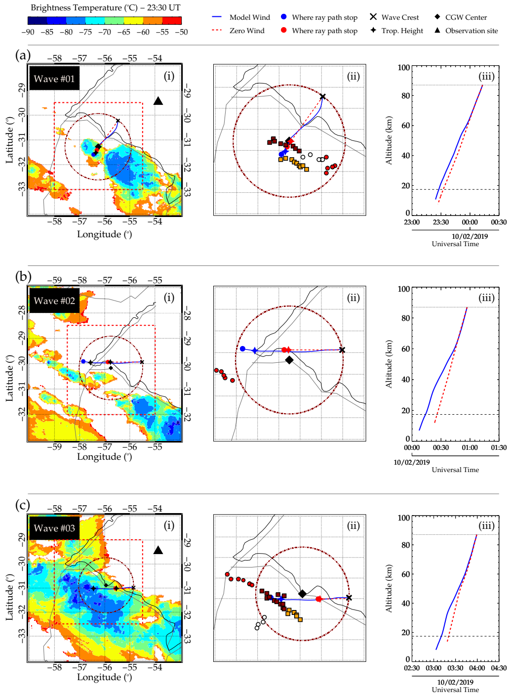
Figure 4. Ray tracing results of concentric gravity wave (CGW) events one (#01), two (#02), and three (#03) on October 01 - 02, 2019.
