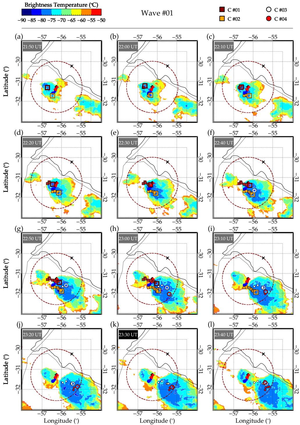
Figure 10. Tracking of the individual convective cores (Cs) #01, #02, #03 and #04 in space and time for Wave #01.
