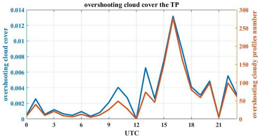
1105 Figure 7: The hourly cloud cover of cirrus shooting over tropopause based on CATS over the TP (blue line). The number of overshooting cloudy profiles every hour (red lines).
