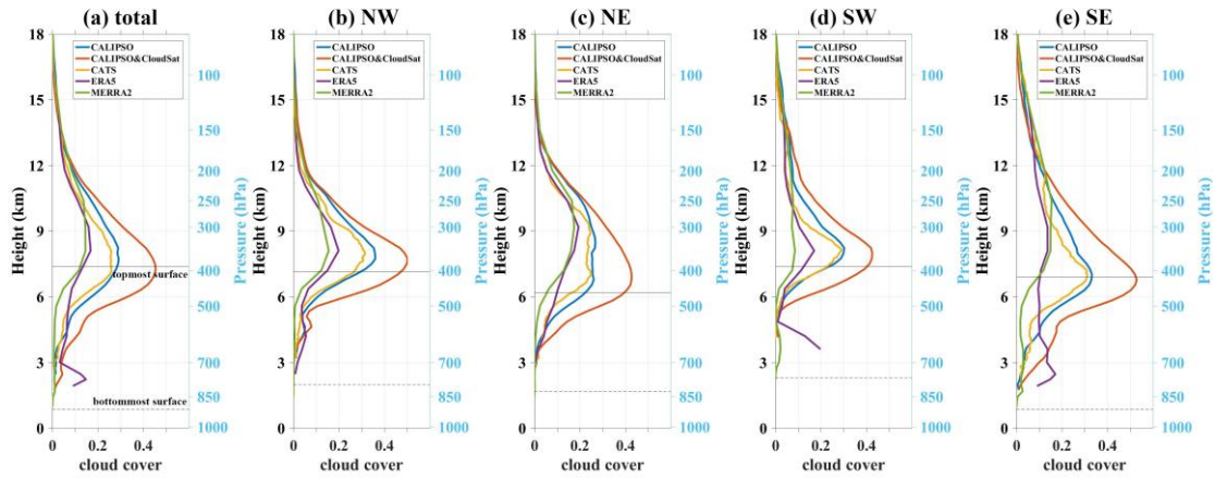
Figure 4: The cloud vertical distribution in different regions of the TP based on CALIPSO (blue lines), 2B-GEOPROF-lidar (CALIPSO&CloudSat, red lines), CATS (yellow lines), ERA5 (purple lines), MERRA-2 (green lines) at the hour closest to the CloudSat and CALIPSO daytime overpass time. (a) The whole TP (b) The northwestern TP (c) The northeastern TP (d) The southwestern TP (e) The southeastern TP. The regions are divided by latitude and longitude lines of 33° N and 89° E and the boundary of TP (shown in Fig. 1). The height here represents the height above the mean sea level. The horizontal solid black lines represent the topmost surface altitude and the dashed black lines represents the bottommost surface altitude obtained in CATS DEM elevation.
