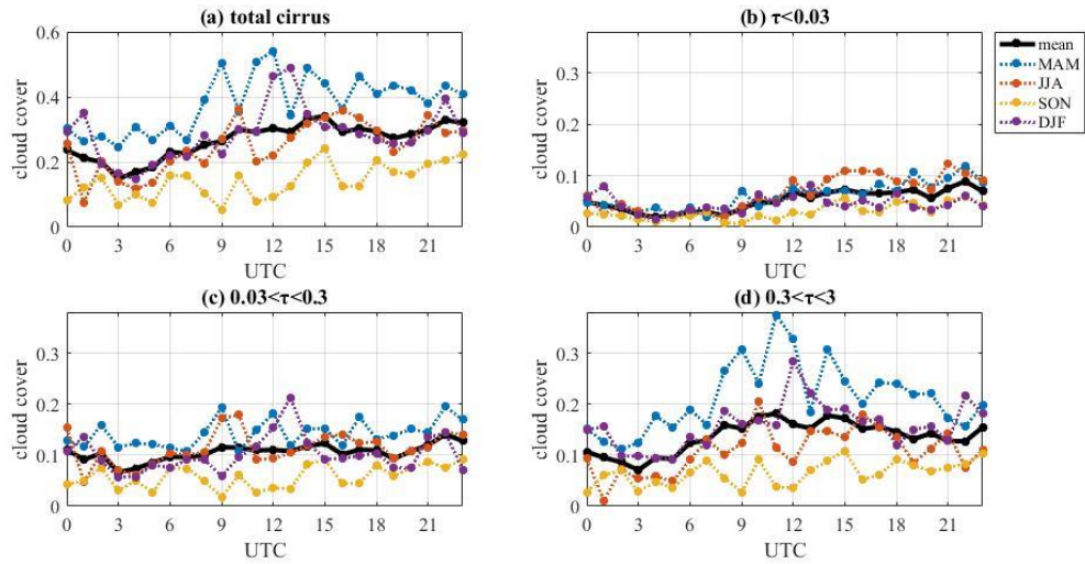
1100 Figure 6: The hourly cloud cover of different types of cirrus of different seasons. The black lines represent the results of annual average, the blue lines represent the results of spring, the red lines represent the results of summer, the yellow lines represent the results of autumn, the purple lines represent the results of winter. All seasons here are northern hemisphere seasons. (a) represents the cloud cover of all cirrus. (b) represents the subvisible cirrus (optical thickness less than 0.03). (c) represents the thin cirrus (optical thickness between 0.03 and 0.3). (d) represents the opaque cirrus (optical thickness between 0.3 and 3).
