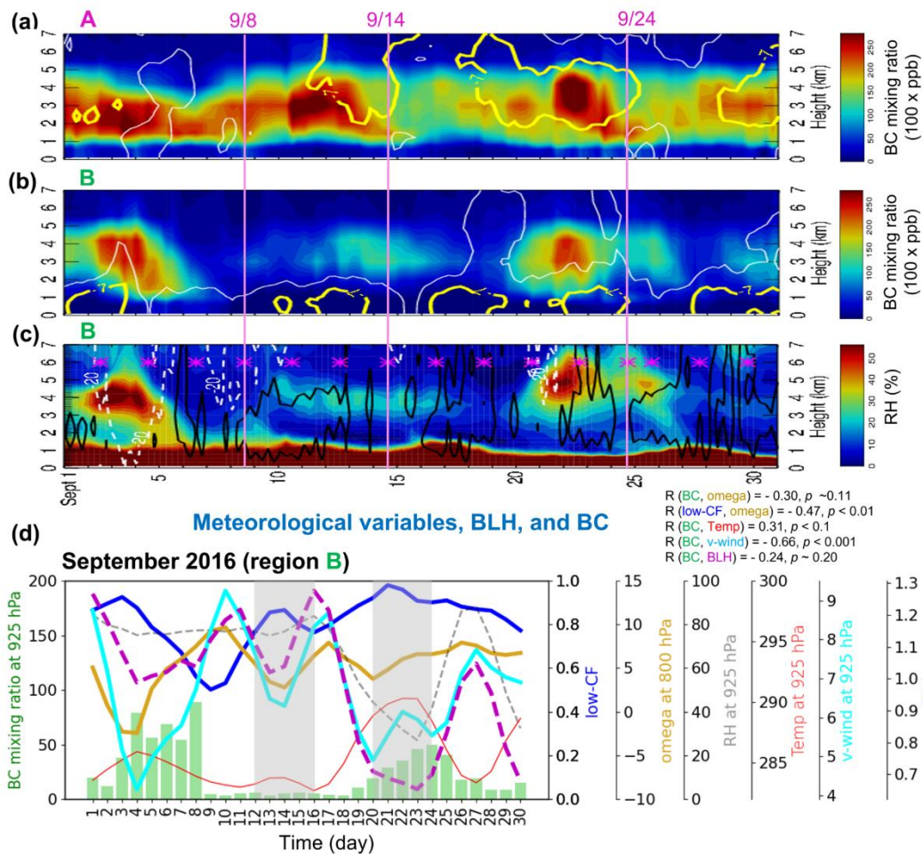
265 Figure 4. (a–b) Time-altitude cross section of 6-hourly BC (shading, ppb x 100) overlaid by 6-hourly zonal wind isotachs at -7 and 0 m s -1 (thick yellow and thin white lines respectively) averaged over (a) region A (0–10° E, 5–15° S) and (b) region B (0–10° E, 15–25° S) in September 2016. (c) The same as (b) but for 6-hourly RH (shading, %) overlaid by 6-hourly vertical velocities of -20 and 50 hPa day -1 (dashed white and solid black lines respectively; positive values represent subsidence) averaged over region B. (d) Time 270 series of daily-mean 925 hPa BC (green bar, ppb x 100), 800 hPa vertical velocity (omega, ω) (gold line, hPa day -1 ), 925 hPa RH (dashed gray line, %), 925hPa temperature (solid red line, K), 925 hPa meridional wind (solid cyan line, m s -1 ), BLH (dashed magenta line, km), and low-CF (blue line) over region B. Each color line represents the 3-day running mean. The asterisk in (c) represents the September 2016 flight days. The pink solid lines in (a–c) refer to the three flight days. The light gray shadings in (d) represent the two periods having different BC-RH conditions. R in (d) refers to Pearson correlation coefficient between two variables in a parenthesis with its statistical significance ( p-value ).
