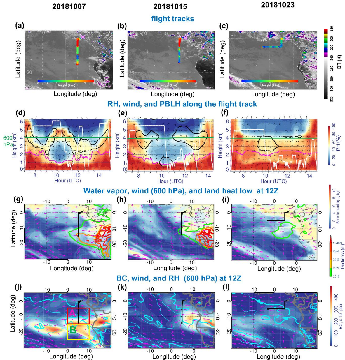
525 Figure 13. (a–c) The horizontal flight tracks during October 2018 ORACLES deployment plotted on Meteosat IR 10.8 \mu\text{m} imagery at 13:45 UTC (shading is Brightness Temperature (BT), K). The color of the flight track represents the altitude of the flight along
