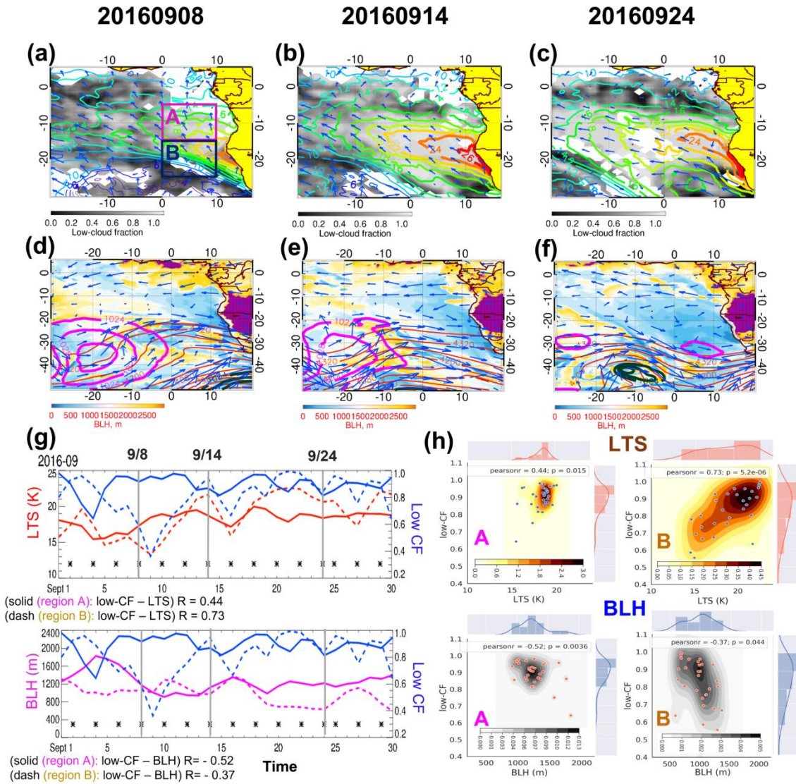
Figure 6. Map of (a–c) daily mean low-CF (shading) overlaid by LTS (contour, K) and 925 hPa horizontal winds (vectors, \text{m s}^{-1} ), (d–f) BLH (shading, m) overlaid by 600 hPa horizontal winds (vectors, \text{m s}^{-1} ), 600 hPa geopotential height (red lines, m), and sea level pressure (SLP; dark green (low-pressure: 996, 1000, 1004), and magenta (high-pressure: 1024, 1028, 1032) lines, hPa) at 12:00 UTC 8, 14, and 24 September 2016. (g) (Top) time series of daily mean low-CF (blue lines) and daily mean LTS (red lines, K), and (bottom) daily mean low-CF (blue line) and daily mean BLH (magenta lines, m) averaged over region A ( 0\text{--}10^\circ \text{ E} , 5\text{--}15^\circ \text{ S} ; solid lines) and region B ( 0\text{--}10^\circ \text{ E} , 15\text{--}25^\circ \text{ S} ; dashed lines) during September 2016. All flight days (8, 14, and 24 September 2016) are marked by asterisk (gray vertical lines). The purple shading over the land in (d–f) refers to BLH higher than 3250 m. (h) The 2-D joint pdf (shading) with scatter plot are shown with 1-D histogram (pdf in line) of (top) daily mean low-CF and LTS and (bottom) daily mean low-CF and BLH over region A (left) and B (right) during September 2016. The solid line in (a) indicates region A (magenta box)
