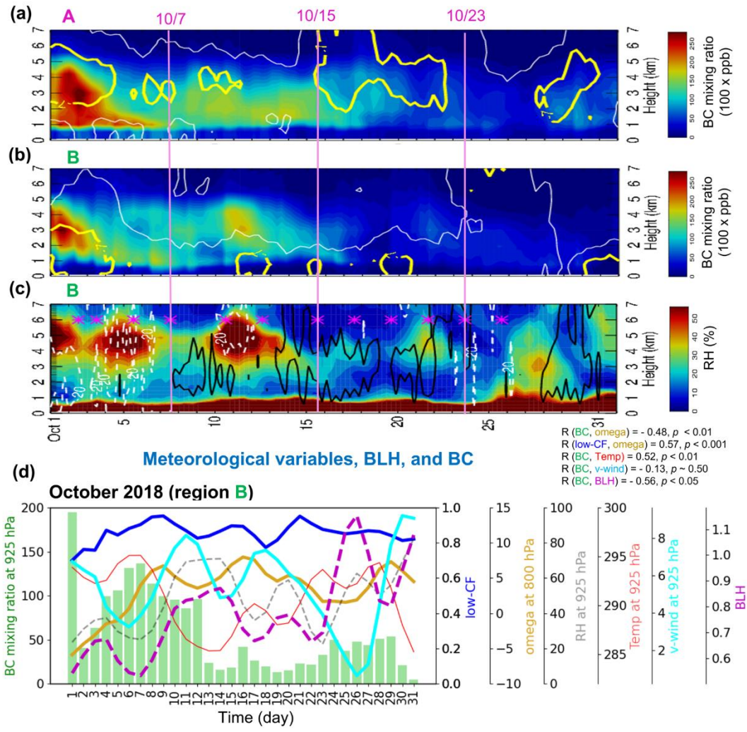
555 Figure 14. (a-b) Time-altitude cross section of 6-hourly BC (shading, ppb x 100) overlaid by 6-hourly zonal wind isotachs at -7 and 0 m s -1 (thick yellow and thin white lines respectively) averaged over (a) region A (0–10° E, 5–15° S) and (b) region B (0–10° E, 15–25° S) in October 2018. (c) The same as (b) but for 6-hourly RH (shading, %) overlaid by 6-hourly vertical velocities of -20 and 50 hPa day -1 (dashed white and solid black lines respectively; positive values represent subsidence) averaged over region B. (d) Time series of daily-mean 925 hPa BC (green bar, ppb x 100), 800 hPa vertical velocity (omega, ω) (gold line, hPa day -1 ), 925 hPa RH (dashed gray line, %), 925hPa temperature (solid red line, K), 925 hPa meridional wind (solid cyan line, m s -1 ), BLH (dashed magenta line, km), and low-CF (blue line) over region B. Each color line represents 3-day running mean. The asterisk in (c) represents the October 2018 flight days. The pink solid lines in (a-c) refer to the three flight days. R in (d) refers to Pearson correlation coefficient between two variables in a parenthesis with its statistical significance ( p -value). 560
