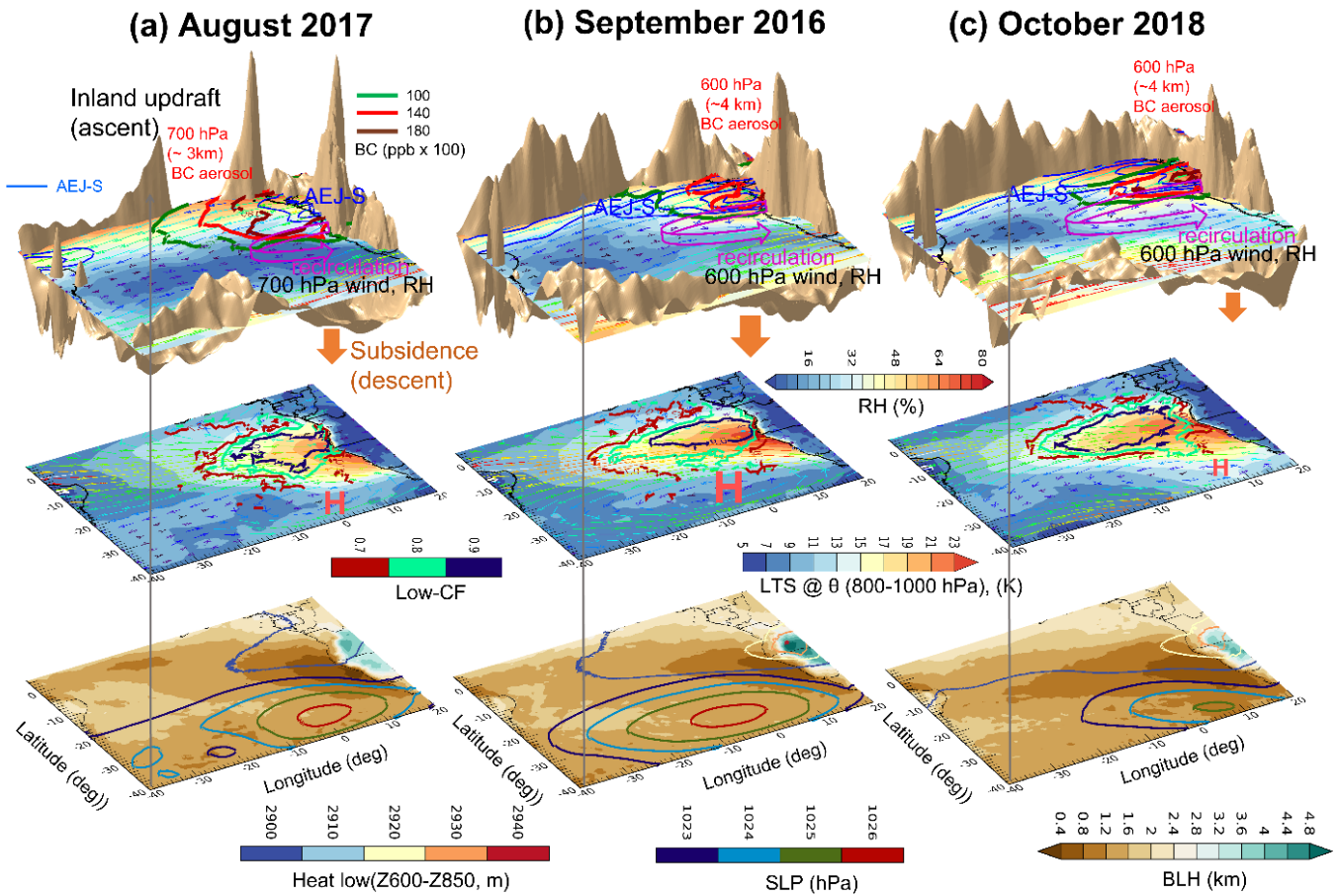
675 Figure 18. Visualization of ( top panels ) map of 700 hPa RH (shading, %), 700 hPa horizontal wind (vector, \text{m s}^{-1} ), and 700 hPa BC aerosols (color lines, \text{ppb} \times 100 ) for August 2017 and the same variables except for 600 hPa in September 2016 and October 2018. The 800 hPa vertical velocity for all months (gold bumpy surface, \omega multiplied by -1 (i.e. -\omega ), \text{hPa day}^{-1} ; above the RH contour plane is updraft and below the RH contour plane is subsidence). ( Middle panels ) map of LTS (shading, K) overlaid by 925 hPa horizontal wind (vector, \text{m s}^{-1} ) and low-CF (color contours, 0.7–0.9 %). ( Bottom panels ) map of BLH (color shading, km) overlaid by thickness between 600 hPa and 850 hPa (color contours, m) and sea level pressure (SLP; color contours, hPa) during (a) August 2017, (b) September 2016, and (c) October 2018. The magenta arrow in the top panels represents the recirculating flow to the African continent. The red “H” mark in mid panels refers to the anticyclones associated with St. Helena High.
