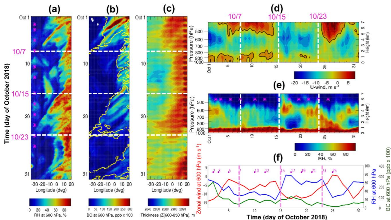
Figure 12. Longitude-time cross-section of 6-hourly (a) 600 hPa RH (%), (b) 600 hPa BC aerosol (shading, ppb x 100) overlaid by 600 hPa zonal wind (yellow line, -7 \text{ m s}^{-1} ), (c) thickness (geopotential height difference (600-850 hPa); high values over a South African plateau represents the heat low, m) averaged over 8\text{--}10^\circ \text{ S} during October 2018. (d–e) Altitude-time cross-section of zonal wind and RH at 10^\circ \text{ S} , averaged over 0\text{--}10^\circ \text{ E} during October 2018. The black contour in (d) represents the 0 value. (f) Daily time series of the 600 hPa zonal-wind (red line, \text{m s}^{-1} ), 600 hPa RH (blue line, %), 600 hPa BC (green line, ppb x 100) averaged over 8\text{--}10^\circ \text{ S} and 0\text{--}10^\circ \text{ E} . The white dashed lines indicate the flight days investigated further in this study, and the magenta asterisks (and numbers in f) represent the flight days during October 2018 deployment.
