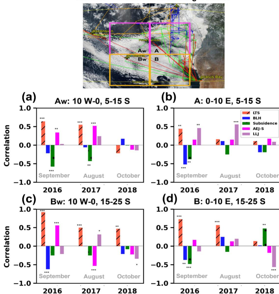
Figure 17. Bar plots of the linear correlation between daily mean low-CF and daily mean of the meteorological variables (LTS, BLH, subsidence, AEJ-S, and LLJ) averaged over four subregions in the ORACLES flight regions over the SE Atlantic Ocean ((a) Aw: 10° W–0, 5–15° S, (b) A: 0–10° E, 5–15° S, (c) Bw: 10° W–0, 15–25° S, and (d) B: 0–10° E, 15–25° S) during the deployment months (marked in the boxed regions over the top image with flight tracks). A and B correspond to the regions A and B shown in the previous figures (e.g., Figs. 3, 4, 6; Figs. 8, 9, 11; Figs. 13, 14, 16), while Aw and Bw correspond to the west of the regions A and B, respectively. *** (**, *) denotes when the correlation is statistically significant within 99% (95, 90 %) confidence interval ( p -value < 0.01 ( < 0.05 ),
