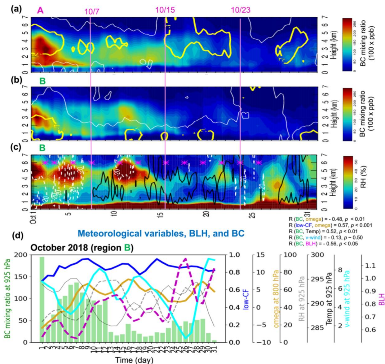
Figure 14. (a-b) Time-altitude cross section of 6-hourly BC (shading, ppb x 100) overlaid by 6-hourly zonal wind isotachs at -7 and 0 m s -1 (thick-yellow and thin-white lines respectively) averaged over (a) region A (0–10° E, 5–15° S) and (b) region B (0–10° E, 15–25° S) in October 2018. (c) The same as (b) but for 6-hourly RH (shading, %) overlaid by 6-hourly vertical velocities of -20 and 50 hPa day -1 (white dashed and black solid lines respectively) averaged over region B. (d) Time series of daily-mean 925 hPa BC (green bar, ppb x 100), 800 hPa vertical velocity (omega, ω) (gold line, hPa day -1 ), 925 hPa RH (gray dashed line, %), 925 hPa temperature (black solid line, K), 925 hPa meridional wind (cyan solid, m s -1 ), BLH (magenta dashed line, km), and low-CF (blue line) over region B. Each color line represents 3-day running mean. The asterisk in (c) represents the October 2018 flight days. The pink solid lines in (a-c) refer to the three flight days.
