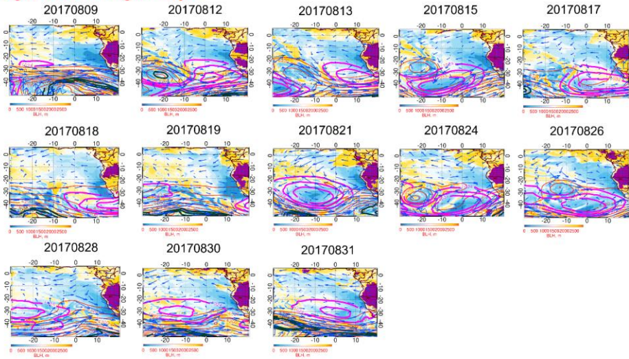
Figure S14. Map of BLH (shading, m) overlaid by 600 hPa horizontal winds (vectors, m s^{-1} ), 600 hPa geopotential height (red lines, m), and sea level pressure (SLP; dark green (low-pressure: 996, 1000, 1004), and magenta (high-pressure: 1024, 1028, 1032), hPa) at 12:00 UTC on flight days in August 2017. The purple shading over the land refers to BLH higher than 3250 m.
