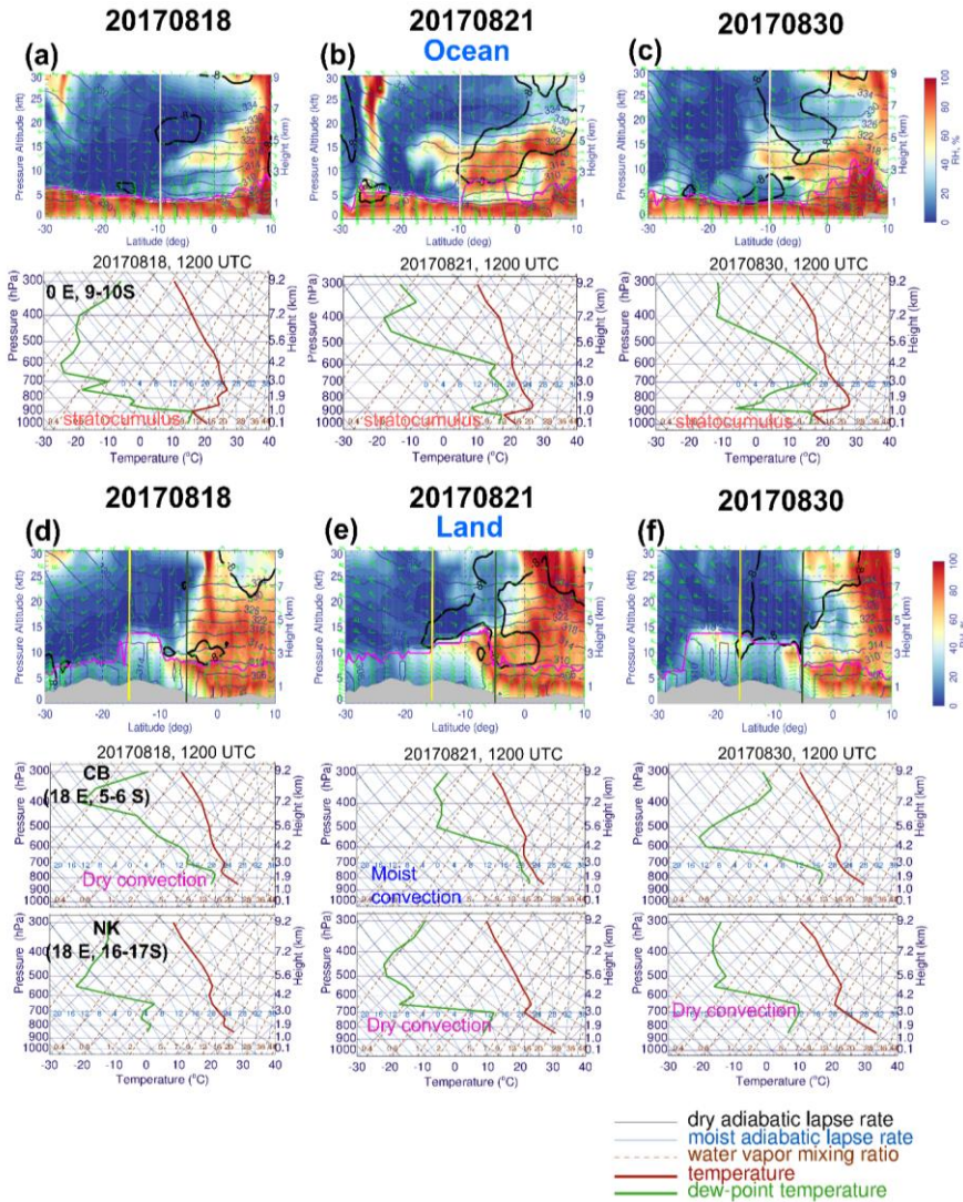
Figure 10. (a–c) Ocean : latitudinal cross-section of RH (shading, %), horizontal winds (wind barbs, green, \text{m s}^{-1} ), \theta (navy, K), and BLH (magenta, m) at 0^\circ \text{ E} (top) and Skew-T log-P diagram averaged over 0^\circ \text{ E} and 9\text{--}10^\circ \text{ S} (bottom: from the left) at 12:00 UTC
