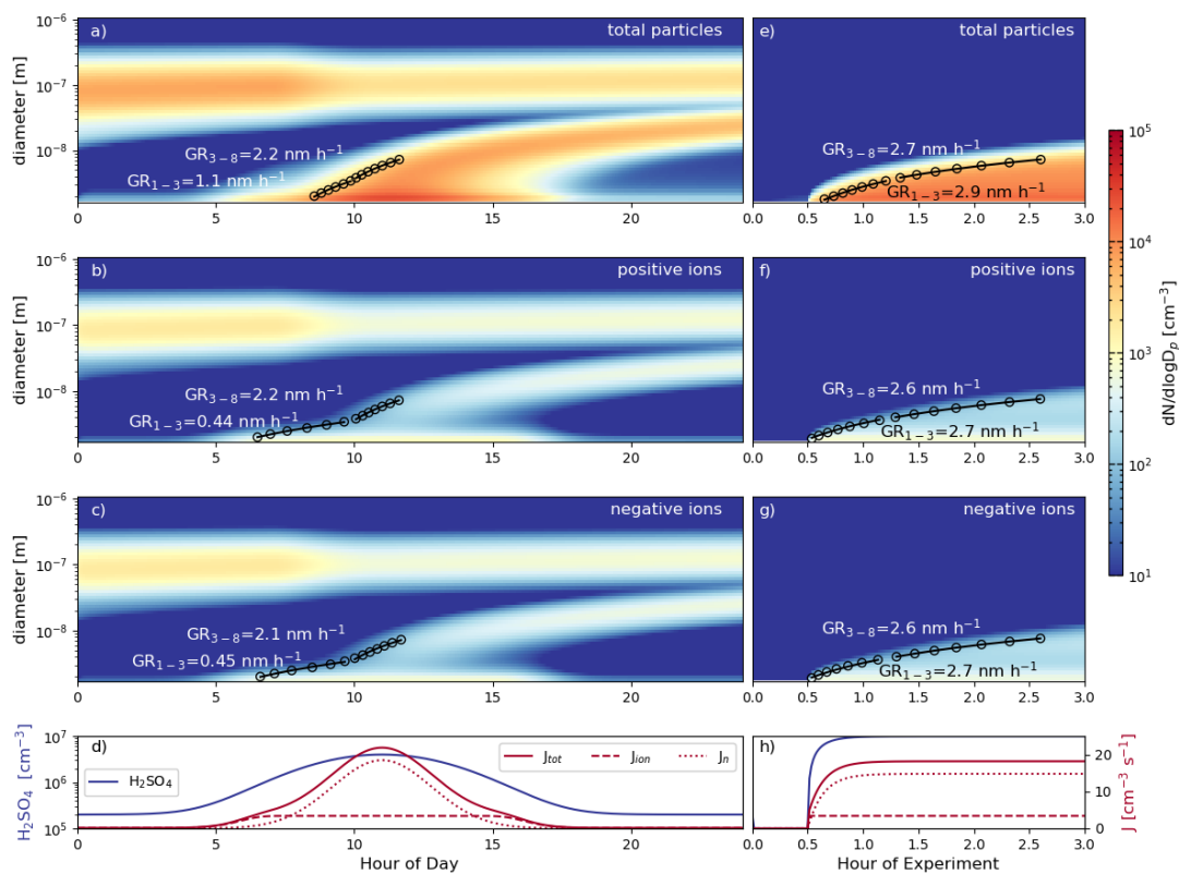
Figure 6: Ion-UHMA model results with the J rates parametrized according to Lehtipalo et al. (2018) for both Hyttiälä (Panels a-d) and CLOUD (Panels e-h) conditions. The upper panels show the total particle size-distribution, the second and third row panels the positive and negative ion size distribution, respectively. The last row panels show the sulfuric acid concentration for vapor growth (blue) and the parametrized nucleation rate according to Lehtipalo et al. (2018) assuming typical profiles of [\text{H}_2\text{SO}_4]^2 [\text{NH}_3] [\text{HOM}_{\text{dim}}] for Hyttiälä and CLOUD.
