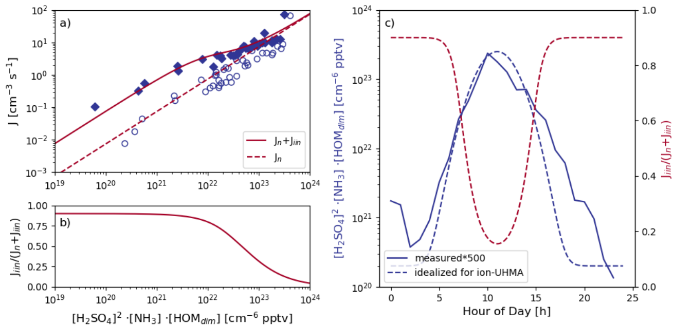
335 Figure 5: The importance of ion-induced nucleation in the boreal forest. a) shows the measured nucleation rates (diamonds under galactic cosmic ray conditions and circles under neutral conditions) and the parametrizations (Eq. (2) and Eq. (4)). b) shows the fraction of ion-induced nucleation from total nucleation rate against the parametrizations from Eq. (2) and Eq. (4). c) shows the diurnal pattern of the calculated nucleation rates and ion-induced fraction in Hyytiälä.
