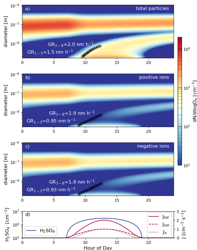
305 Figure 4: Model results based on Leppä et al. (2009) with the ion-induced nucleation starting 1 hour earlier than the neutral pathway as suggested by the conceptual approach of Gonser et al. (2014). The first panel corresponds to the total particle size distribution, the second and third panel are the ion (positive and negative) size distributions. The calculated apparent growth rate
