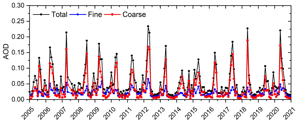
Figure S1. Series of monthly mean values of total (black), fine (blue) and coarse-mode AOD (red) at IZO between 2005 and 2021.
