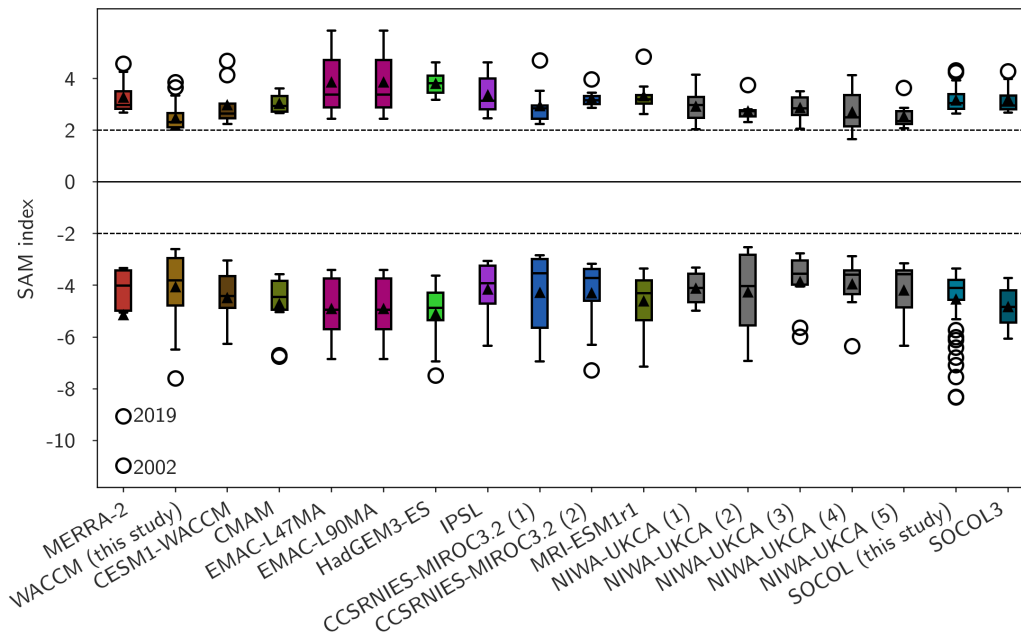
Figure A6. The 10 hPa SAM index values of the 25 % lowest and highest springtime SAM indices in MERRA-2 and the CCMI models (10 events per weak/strong category), and in the time-slice simulations of WACCM and SOCOL (50 events per weak/strong category).
