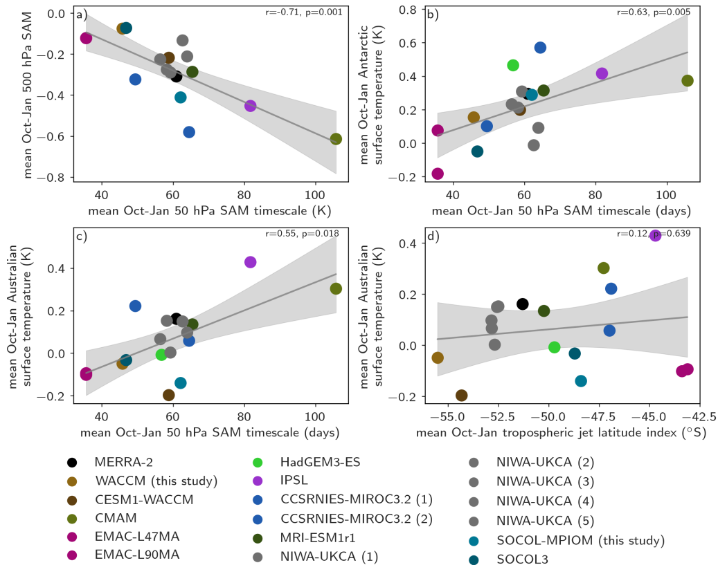
Figure A7. The mean October-January 50 hPa SAM timescale in each model and the reanalysis data versus the mean Oct-Jan 500 hPa SAM response (a), Antarctic temperature anomalies (b), Australian temperature anomalies (c) following weak polar vortex events, and the Oct-Jan mean tropospheric jet latitude index versus Australian temperature anomalies following weak polar vortex events (d). The Spearman correlation coefficients and p-values are annotated in the upper right corner for each relationship.
