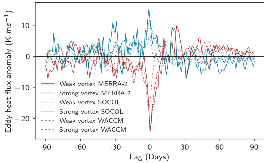
Figure A3. Composites of eddy heat flux anomalies (K m/s) averaged over 45-75°S at 100hPa for strong and weak polar vortex events for MERRA-2 and the CCMs SOCOL and WACCM. The central date (lag 0) refers to the onset day of the polar vortex anomaly.
