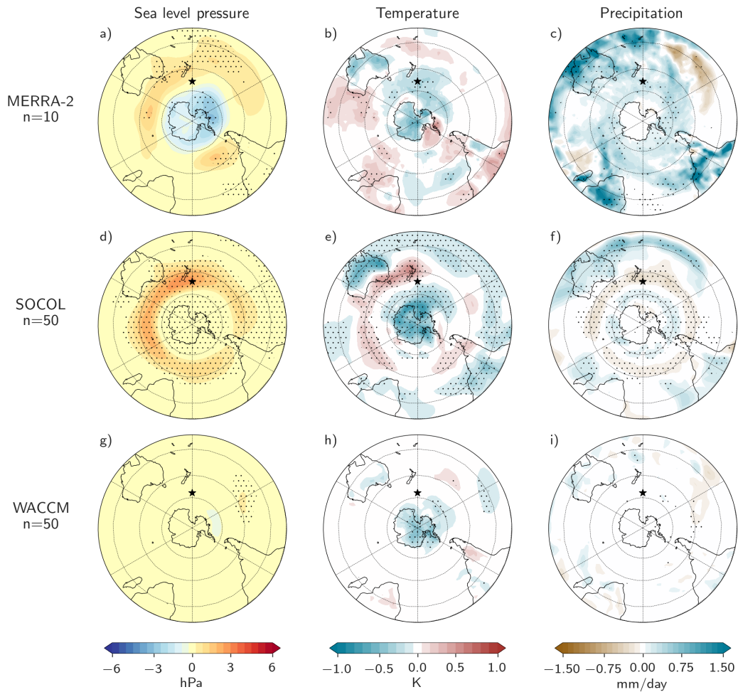
Figure A4. Surface climate composites for strong polar vortex regimes for October-January SLP anomalies (a,d,g), 2-meter temperature anomalies (b,e,h) and precipitation anomalies (c,f,i). The reanalysis data MERRA-2 (first row) includes 10 weak vortex regimes, and the CCMs SOCOL (second row), and WACCM (third row) each include 50 weak vortex regimes. Stippling refers to significance at the 4.5% level assessed with a bootstrapping test.
