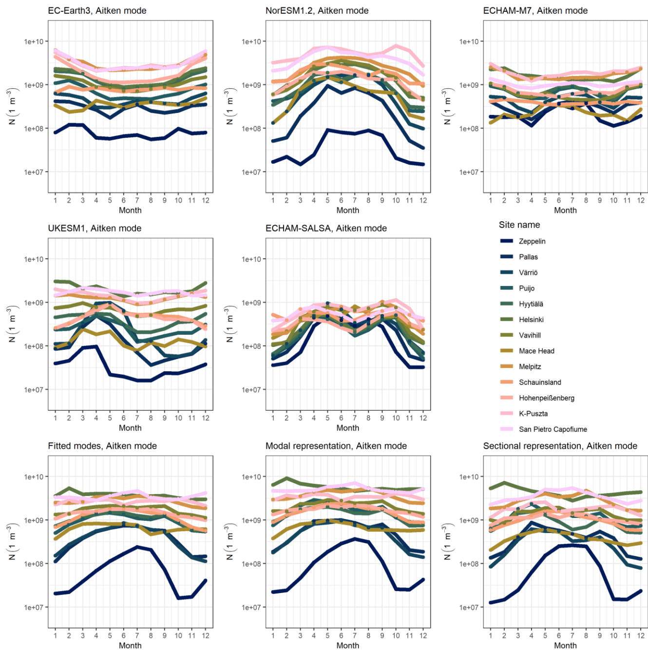
775 Figure 11. Seasonal cycle of Aitken mode number concentration in measurements and climate models for measurement sites. A subplot represents the seasonal cycle in one model or measurement. Coloured lines represent the median of the monthly means for Aitken mode number concentrations. Sites are ordered from most northerly to most southerly.
