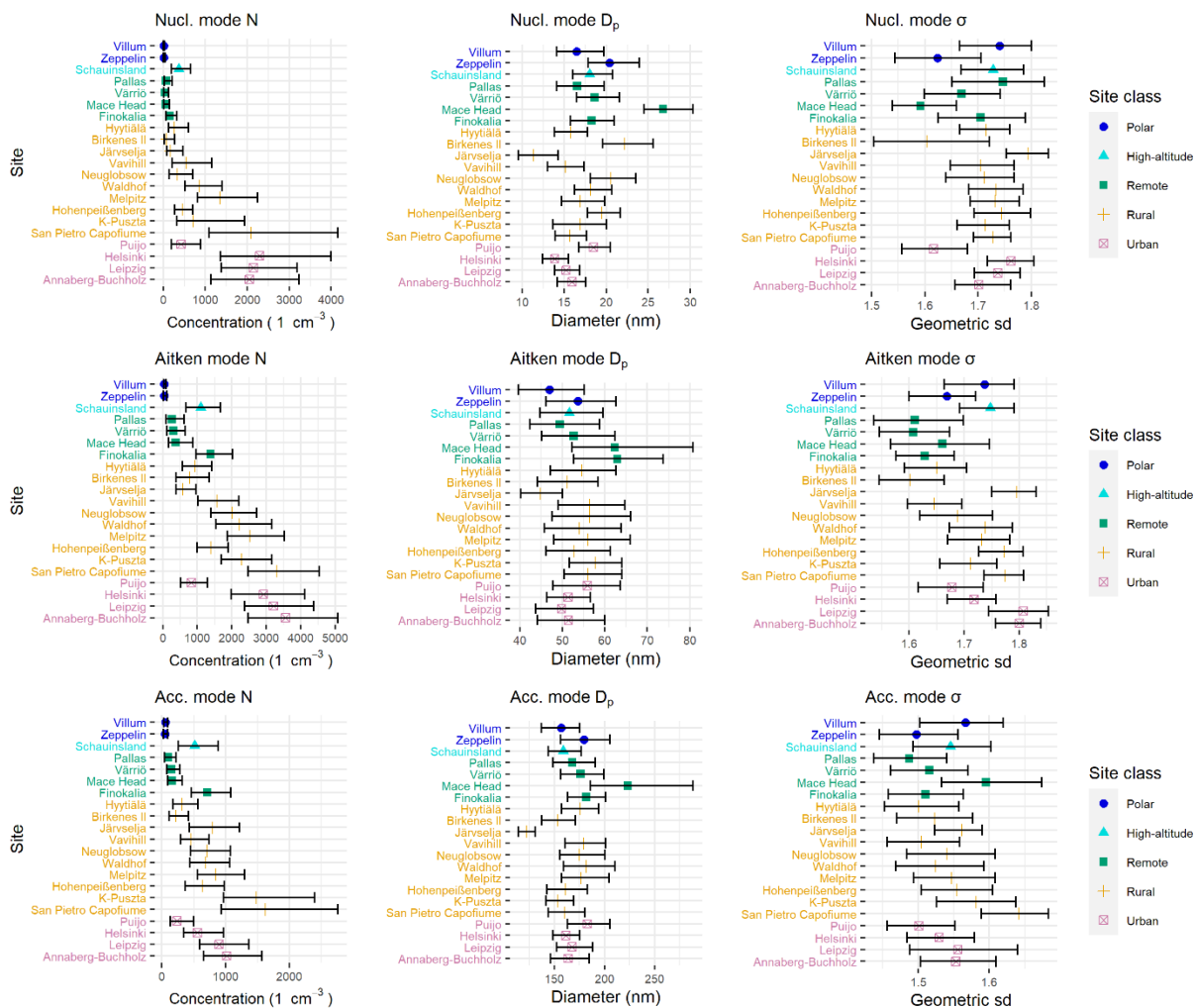
500 Figure 1. Summary of mode parameters (number concentration N , geometric mean diameter D_p , and geometric standard deviation \sigma ) for the measurement sites. The median values are marked with dots and interquartile ranges (25% and 75%) with whiskers for different mode parameters in fitted modes.
