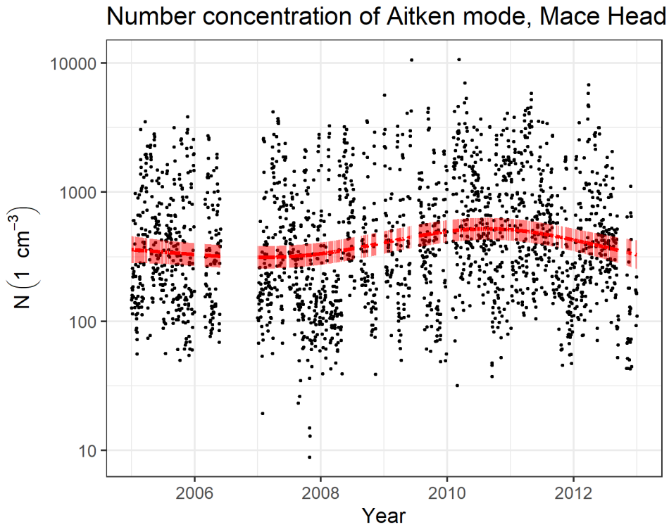
Figure 2. DLM fit for Mace Head Aitken mode number concentration. Black dots represent daily averages of Aitken mode number concentrations in Mace Head. The red solid line represents the estimated level, and the red ribbon represents the 95% confidence interval for the level.
