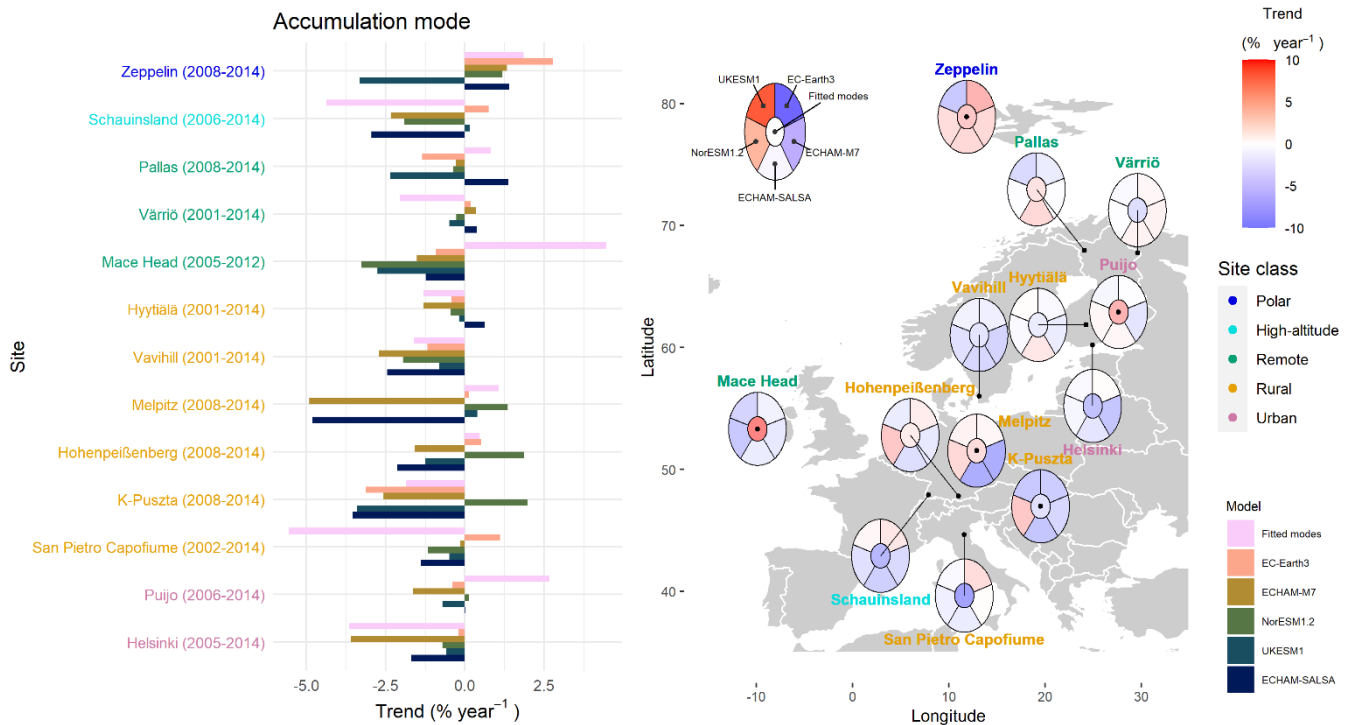
Figure 8. Long-term trend estimates for measured and modelled accumulation mode number concentration. Left panel: Bar plot of trends in different sites. Sites (y axis) are arranged by site class and within each site class from north to south. Right panel: Estimated trends presented in the map. The colour of the central part follows the trend of the fitted modes. Trends have been calculated using Sen-Theil estimator and complemented with bootstrap confidence intervals (see section 2.3.2).
