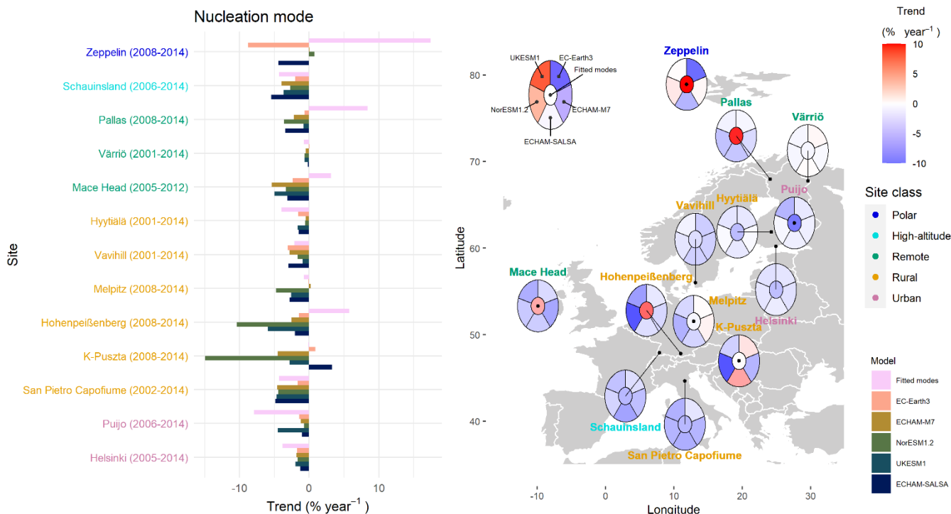
640 Figure 6. Long-term trend estimates for measured and modelled nucleation mode number concentration. Left panel: Bar plot of trends for different sites. The sites (y axis) are arranged by site class and within site class most northerly to most southerly. Right panel: Estimated trends presented in the map. The colour of the central part follows the trend of the fitted modes. Trends have been calculated using Sen-Theil estimator and complemented with bootstrap confidence intervals (see section 2.3.2).
