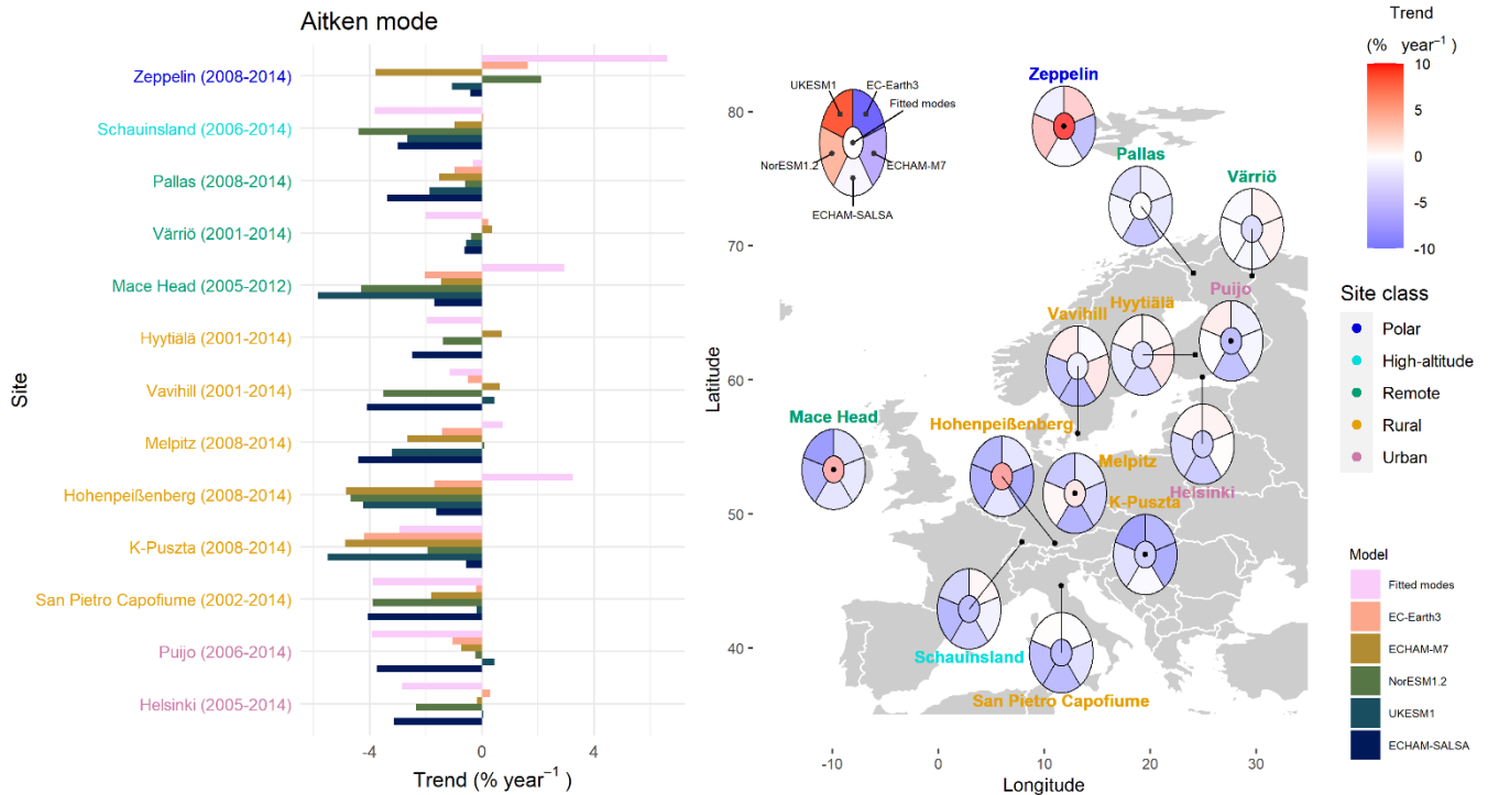
665 Figure 7. Long-term trend estimates for measured and modelled Aitken mode number concentration. Left panel: Bar plot of trends in different sites. Sites (y axis) are arranged by site class and within site class most northerly to most southerly. Right panel: Estimated trends presented in the map. The colour of the central part follows the trend of the fitted modes. Trends have been calculated using Sen-Theil estimator and complemented with bootstrap confidence intervals (see section 2.3.2).
