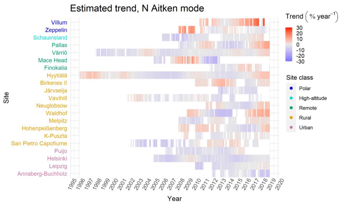
Figure 3. Estimated trends for Aitken mode D_p and N at measurement sites. Trend has been calculated by DLM, see section 2.3.1 for details. The overall trend presented in the figure is comparable with the long-term trend estimates given in section 3.1. To get a DLM trend for one year, the one-day trend given by the model was multiplied by the number of days in a year (365 used for all years) and divided by the mean of the variable over the first observed year. For example, if the trend is showing an increase of 10% / year it means that if the short-term increase would continue for a year, the concentration would be increased by 10% during the year compared to the first year mean.
