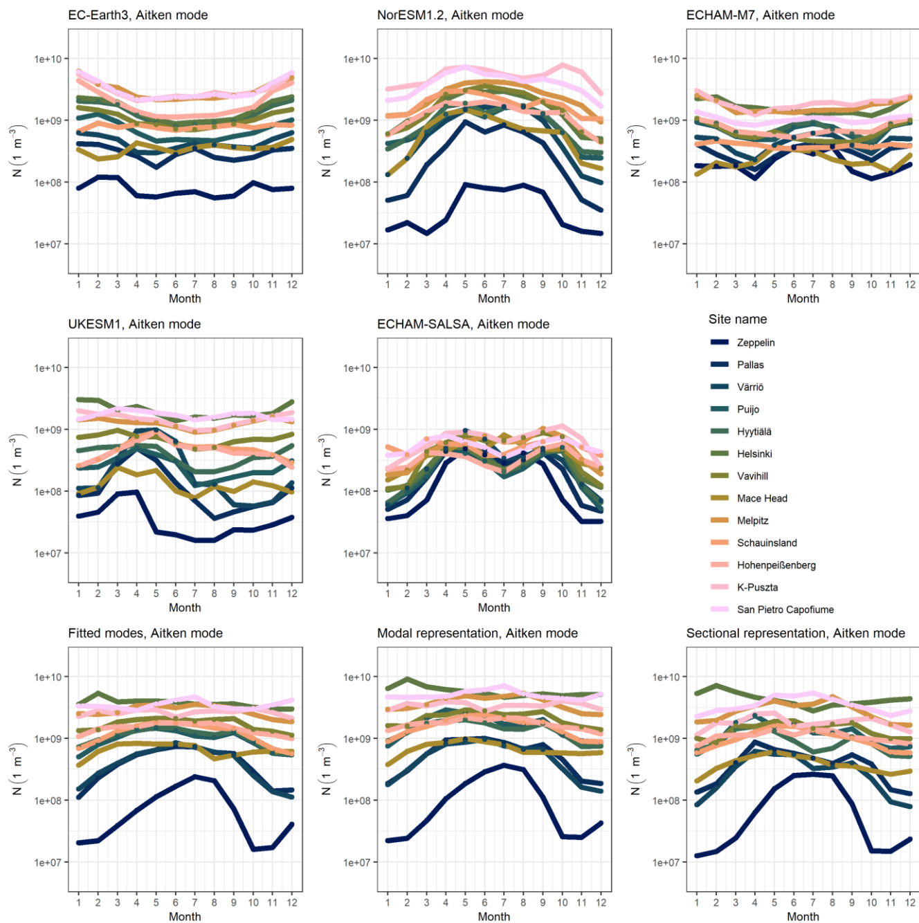
810 Figure 11.4 Seasonal cycle of Aitken mode number concentration in measurements and climate models for measurement sites. A subplot represents the seasonal cycle in one model or measurement. Coloured lines represent the median of the monthly means for Aitken mode number concentrations. Sites are ordered from most northerly to most southerly.
