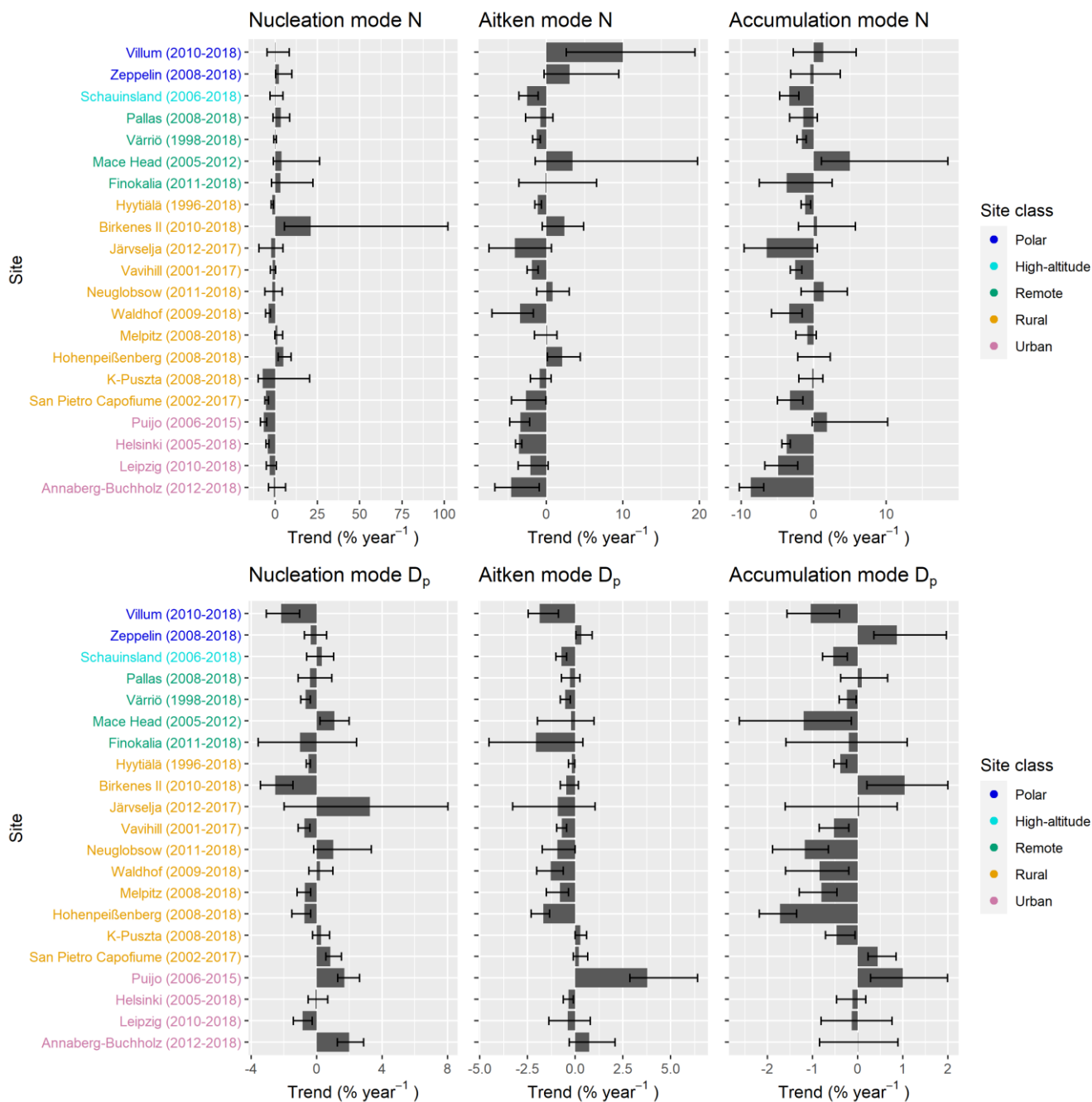
600 Figure 4. Long-term trend estimators for measured trends of all mode parameters (mean geometric diameter D_p , geometric standard deviation \sigma , and number concentration N ) in nucleation (NuclM), Aitken (AitM), and accumulation mode (AccM). Confidence intervals (95% confidence level) are shown with whiskers. Statistically significant (95% confidence level) trends are bolded, marked with an asterisk, and highlighted with border lines. Trends have been calculated using Sen-Theil estimator and complemented with bootstrap confidence intervals (see section 2.3.2).
