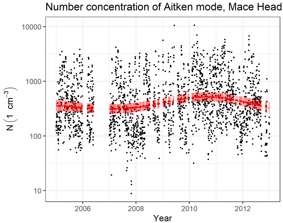
535 Figure 2. DLM fit for Mace Head Aitken mode number concentration. Black dots represent daily averages of Aitken mode number concentrations in Mace Head. The red solid line represents the estimated level, and the red ribbon represents the 95% confidence interval for the level.
