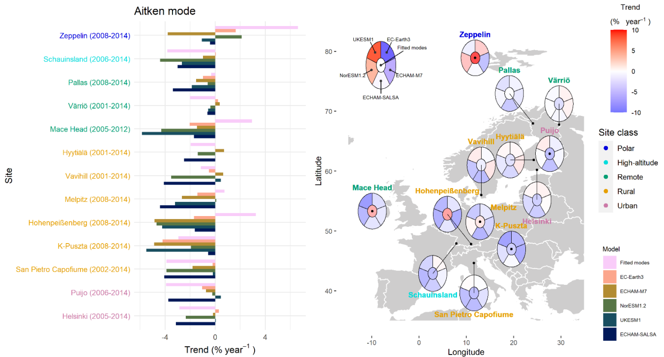
690 Figure 7. Long-term trend estimates for measured and modelled Aitken mode number concentration. Left panel: Table- Bar plot of trends in different sites. Sites (y axis) are arranged by site class and within site class most northerly to most southerly from north to south. Statistically significant (95% confidence level) trends are bolded, marked with an asterisk, and surrounded by a black border. Right panel: Estimated trends presented in the map. The colour of the central part follows the trend of the fitted modes. Trends have been calculated using Sen-Theil estimator and complemented with bootstrap confidence intervals (see section 2.3.2).
