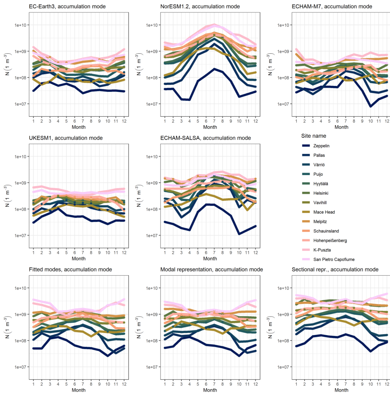
815 Figure 12. The seasonal cycle of accumulation mode number concentration in measurements and climate models for measurement sites. A subplot represents the seasonal cycle in one model or measurement. Coloured lines represent the median of the monthly means for accumulation mode number concentrations. Sites are ordered from most northerly to most southerly.
