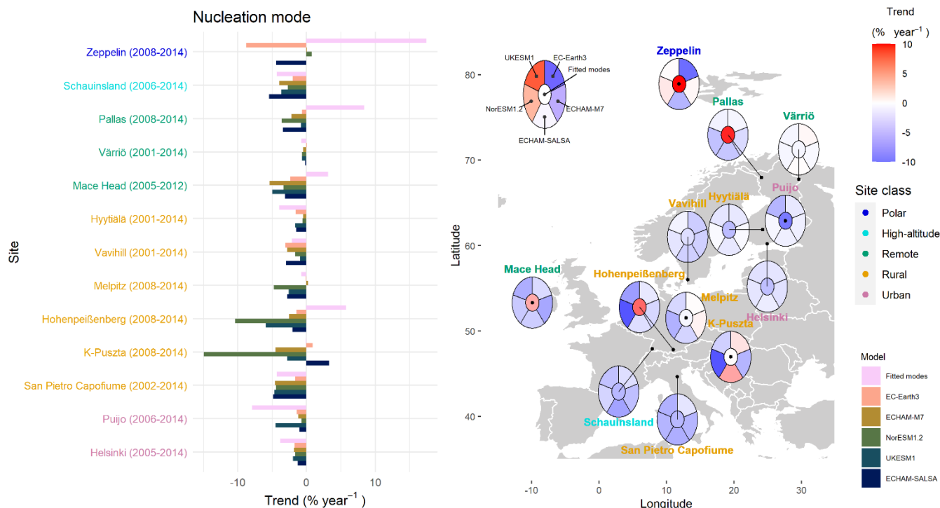
665 Figure 6. Long-term trend estimates for measured and modelled nucleation mode number concentration. Left panel: Table Bar plot of trends for different sites. The sites (y axis) are arranged by site class and within site class most northerly to most southerly from north to south. Statistically significant (95% confidence level) trends are bolded, marked with an asterisk, and surrounded by a black border. Right panel: Estimated trends presented in the map. The colour of the central part follows the trend of the fitted modes. Trends have been calculated using Sen-Theil estimator and complemented with bootstrap confidence intervals (see section 2.3.2).
