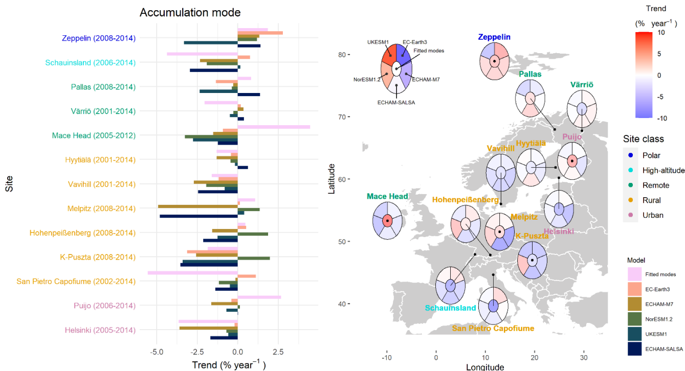
715 Figure 8. Long-term trend estimates for measured and modelled accumulation mode number concentration. Left panel: Table Bar plot of trends in different sites. Sites (y axis) are arranged by site class and within each site class from north to south most northerly to most southerly from north to south . Statistically significant (95% confidence level) trends are bolded, marked with an asterisk, and surrounded by a black border. Right panel: Estimated trends presented in the map. The colour of the central part follows the trend of the fitted modes. Trends have been calculated using Sen-Theil estimator and complemented with bootstrap confidence intervals (see section 2.3.2).
