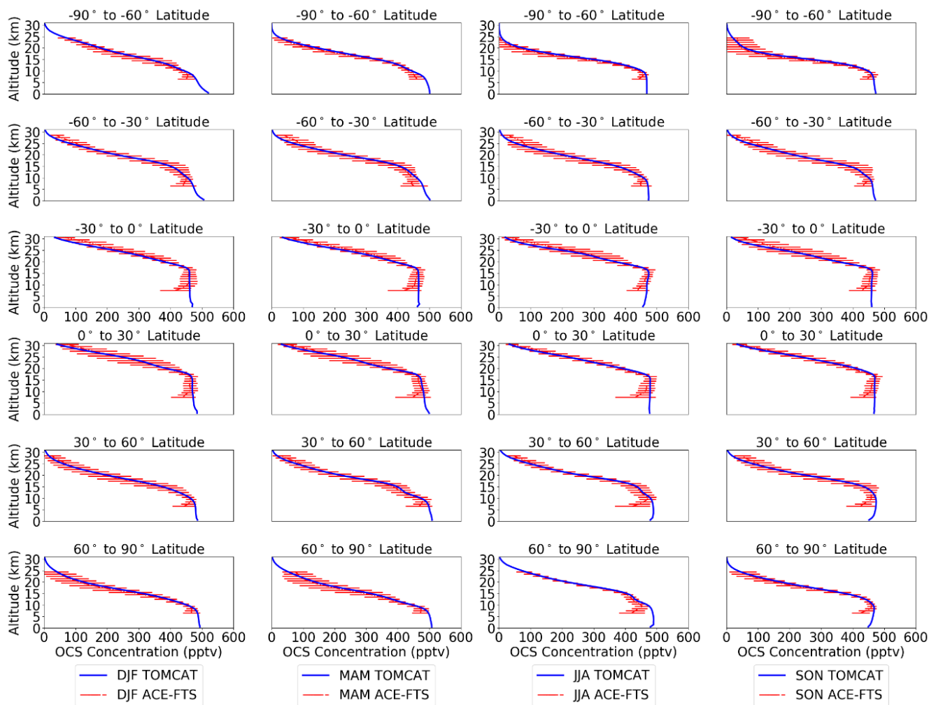
545 Figure 4. Seasonal mean vertical profiles of OCS concentration (mixing ratio, ppt) from TOMCAT model output (blue) and ACE (red) for six different latitude regions. The error bars are standard deviation of ACE at each altitude level. All profiles are seasonal averages between the years 2004 to 2018.
