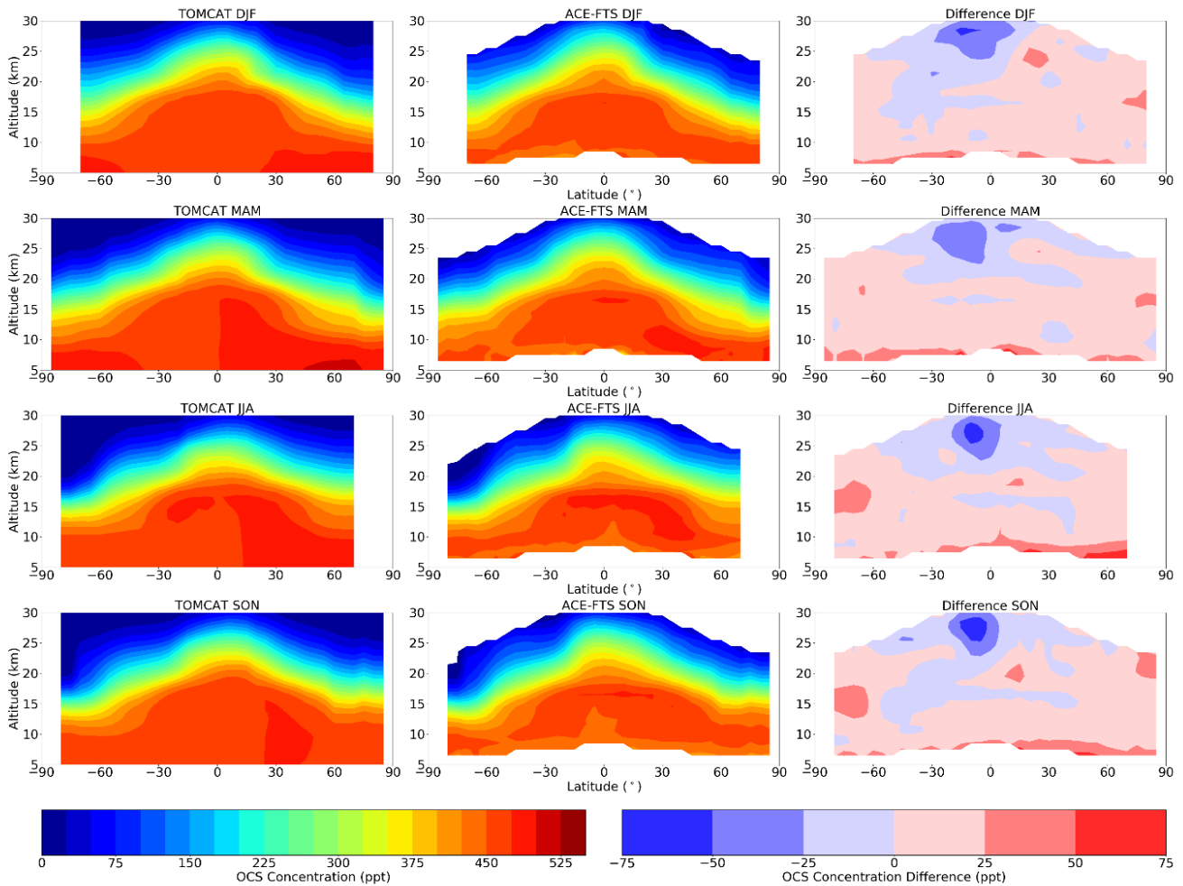
525 Figure 3. Seasonal zonal mean concentration (mixing ratio) of OCS (ppt) from TOMCAT OCS (left), ACE (centre) and the difference between the two (TOMCAT OCS minus ACE, right) for the period of 2004 to 2018. TOMCAT OCS and ACE data averaged in 5-degree latitude bins and over all longitudes.
