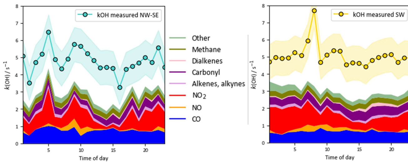
15 Figure 13. Median diel profiles of the OH reactivity calculated from measured reactants and comparison to measured OH reactivity, split according to wind direction. Average daytime contributions are given in Table 3. For interpretation of colours, please see the figure legend. Reactants in the “Other” class are listed in Table 3. The shaded area on measured k'_{\text{OH}} corresponds to the 1\sigma precision of \sim 1 \text{ s}^{-1} . Model intermediates are not included here but their contributions are discussed in the text.
