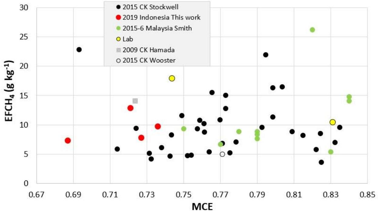
Figure 2. The emission factor for CH 4 (g kg -1 ) versus MCE for field studies sampling pure peat fires in the tropics and lab studies of pure tropical peat smoke that also included extensive NMOG data. “CK” indicates the Indonesian province Central Kalimantan. Black Stockwell et al. (2016a), red this work (provincial averages), green Smith et al. (2018), gray Hamada et al. (2013), unfilled circle Huijnen-Wooster et al. (20152018) . Lab data (yellow) shown are from Fire #55 in FIREX (MCE = 0.831) and Fire #114 in FLAME-4 (MCE = 0.744). See text for additional details.
