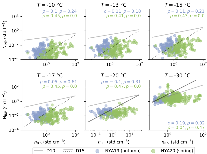
Figure 4. Observed INP concentration at selected temperatures as a function of the particle larger than 0.5\text{ }\mu\text{m} (volume equivalent diameter) number concentration ( n_{0.5} ) during sampling in the autumn (violet) and spring (green) campaign. The Spearman's rank coefficient ( \rho ) and p value are given for for each plot. Predicted INP concentration by DeMott et al. (2010) (D10) and DeMott et al. (2015) (D15) are presented in solid gray and black, respectively. Predictions of the D15 parameterization outside of the applicable temperature range ( T > -20\text{ }^{\circ}\text{C} ) are indicated in dashed lines.
