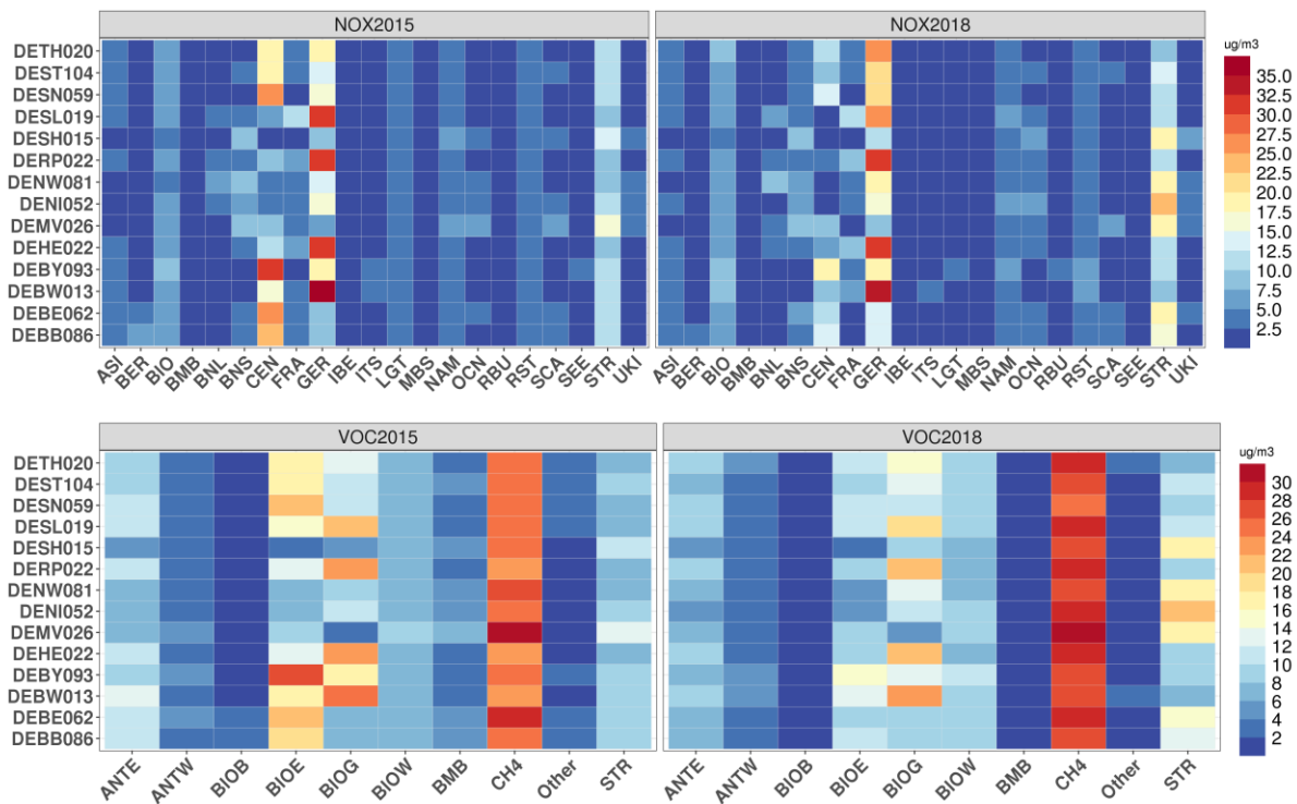
1085 Figure 5. Contribution to mean surface O 3 at 14 receptor stations from local and other European sources, HTAP2 sources, and other global sources. The upper panels denote the mean contribution of NO x precursor to total O 3 during 6 – 13 August 2015 (left) and 1 – 8 August 2018 (right). The bottom panels denote the mean contribution of VOC precursors to total O 3 during 6 – 13 August 2015 (left) and 1 – 8 August 2018 (right).
