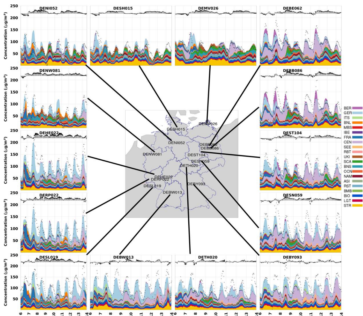
1090 Figure 6. Contribution of regional NO x sources to hourly O 3 concentrations of local and other European sources, HTAP2 source regions, and other global source types at each station during the 6 – 13 August 2015 period. In addition, the vectors along the top of each panel represent the calculated wind speed and direction at 10 m above ground level. The black dots represent the observed O 3 concentrations.
