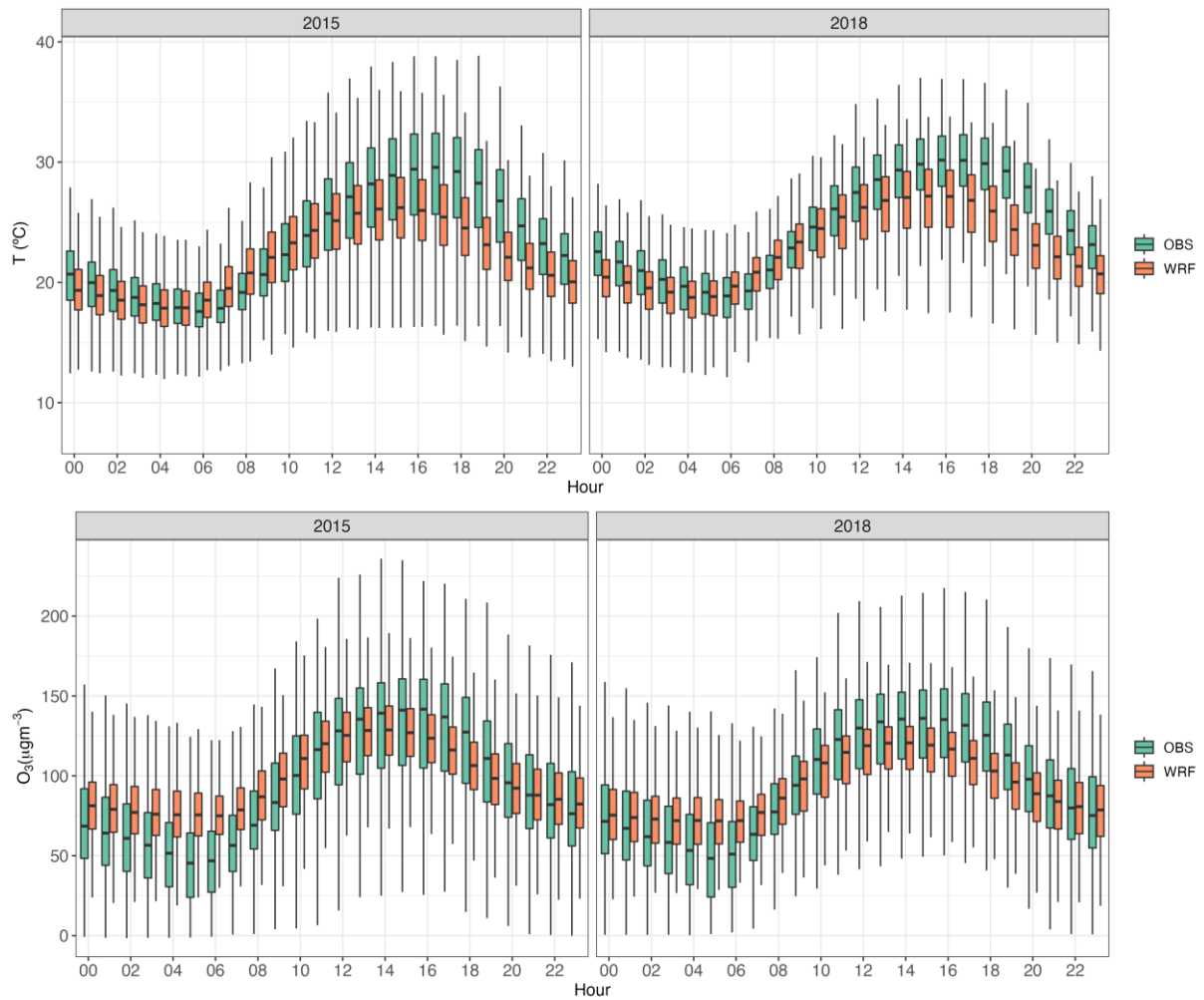
1070 Figure 1 Observed and simulated diel percentile for temperature and O 3 over the analyzed periods at the German “background” stations. Note that the “OBS” temperature is given by ERA5 temperature extracted at the German background station locations. Vertical lines denote 5 th and 95 th percentiles, boxes denote 25 th and 75 th percentiles, and the black line denotes the 50 th percentiles.
