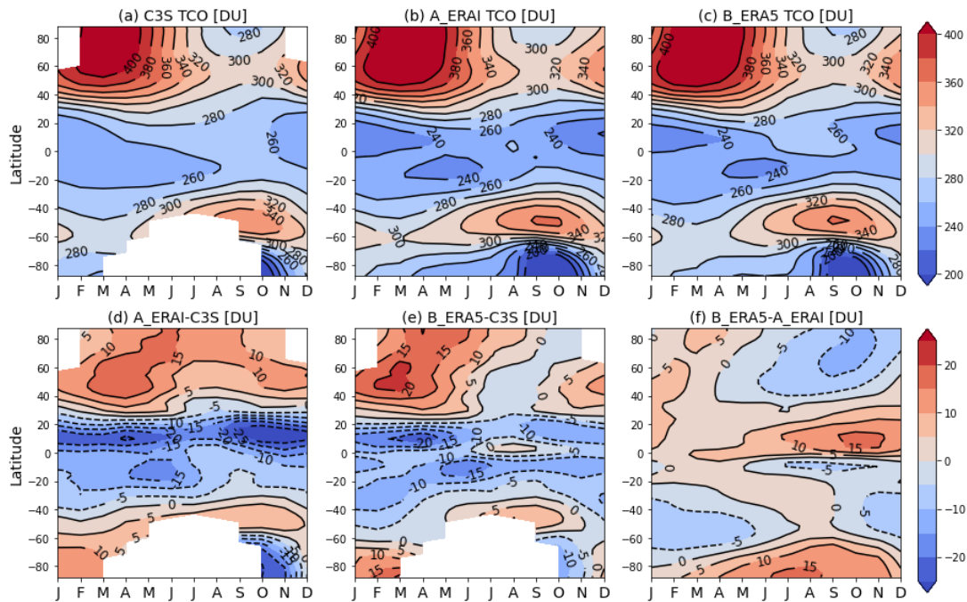
Figure 2: Zonal and monthly mean TCO (DU) climatology over the period 1979-2018 based on (a) C3S and two model simulations (b) A_ERAI and (c) B_ERAS. The absolute differences between each simulation and C3S, as well as between the two simulations, are shown in (d) A_ERAI - C3S, (e) B_ERAS - C3S and (f) B_ERAS - A_ERAI, respectively.
