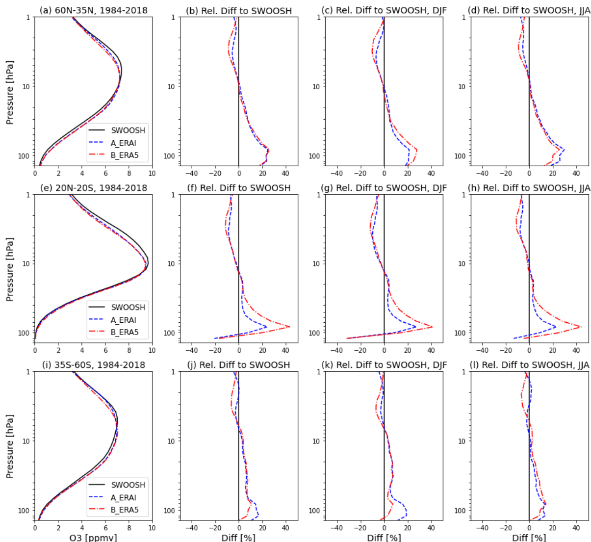
365 Figure 5: Averaged vertical ozone profiles from SWOOSH (black solid line), A_ERAI (blue dashed line) and B_ERAI5 (red dash-dot line) for (a-d) 60°N-35°N, (e-h) 20°N-20°S, and (i-l) 35°S-60°S (1984-2018). Relative differences (%) referencing each simulation to SWOOSH averaged in the whole time period as well as DJF and JJA seasons are shown in the three right-hand columns for comparison.
