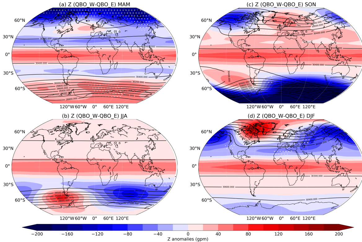
Figure 11. Influences of QBO (QBO W-QBO E) on global geopotential height (Z at 10 hPa) based on ERA5 data for the period 1979-2020. The climatological values of geopotential height in each season are also shown (contour lines). (a) MAM. (b) JJA. (c) SON. (d) DJF. Stippled areas indicate results that are statistically significant over the 99.95% level, using the two-tailed Student's t-test.
