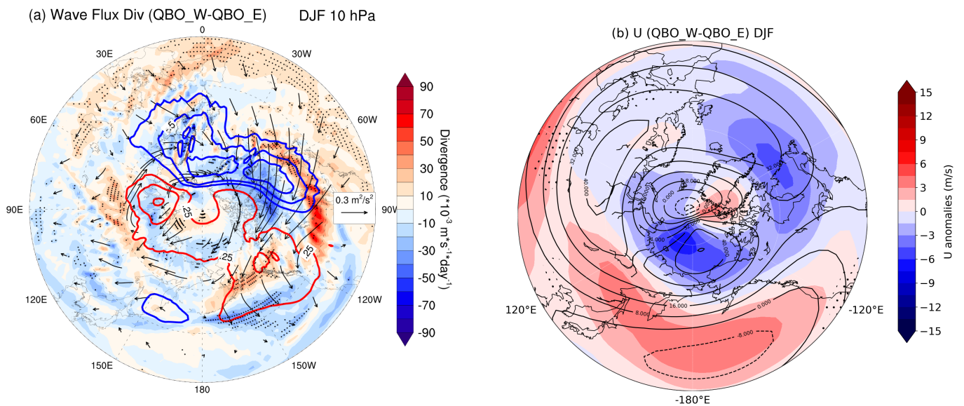
Figure 13. Influences of QBO (QBO_W-QBO_E) on T-N wave flux (a) and zonal winds (b) at 10 hPa north of 30°N during winter (DJF) based on ERA5 data for the period 1979-2020. In (a), the meridional and zonal components of the wave flux are shown as vectors, the vertical component is shown as contour lines (positive in red) and the divergence of the wave flux is shaded. In (b), the climatological values of zonal wind are shown in contour lines (solid lines for westerly) and the anomalies are shaded. Stippled areas indicate results that are statistically significant over the 95% level, using the two-tailed Student's t -test.
