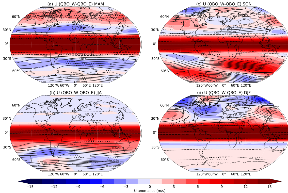
Figure 9. Influences of QBO (QBOW-QBOE) on the global zonal wind (U at 10 hPa) based on ERA5 data for the period 1979-2020. The climatological values of zonal winds in each season are also shown (contour lines). (a) MAM. (b) JJA. (c) SON. (d) DJF. Stippled areas indicate results that are statistically significant over the 99.5% level, using the two-tailed Student's t-test.
