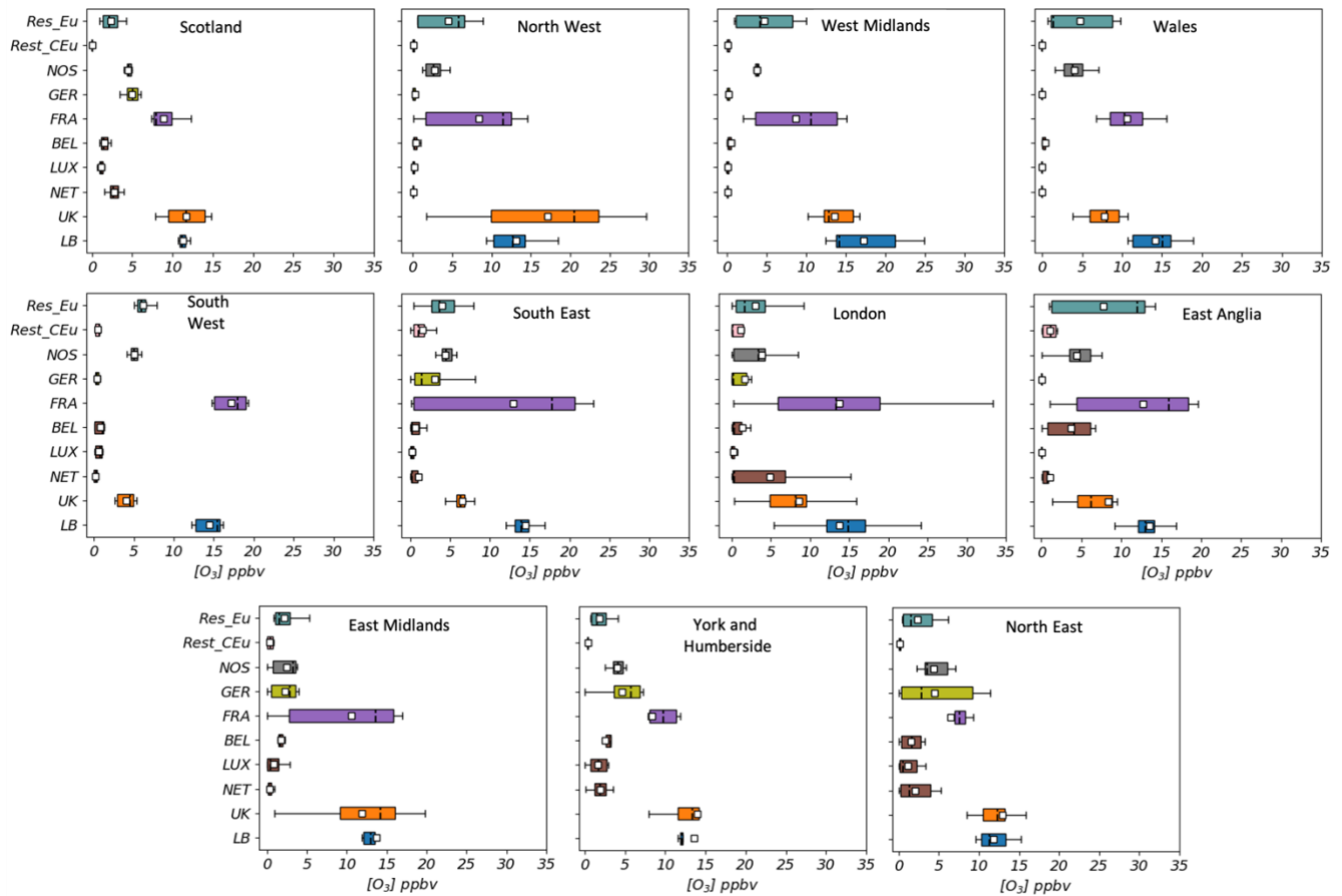
860 Figure 10. Hourly contributions, in ppbv, to surface O 3 at 11 UK receptor regions from 10 source regions (UK, background (LB), the 865 Netherlands, Luxembourg, Belgium, France, Germany, rest of Central Europe (Rest_CEu), North Sea and English Channel (NOS) and rest 870 of Eu) during days when the MDA8 is above 50 ppbv between May and August. The lower and upper ends of the boxes indicate the 25 th 875 and 75 th percentiles, the black dashed line the median, the white boxes the mean and the whiskers the minima and maxima.
