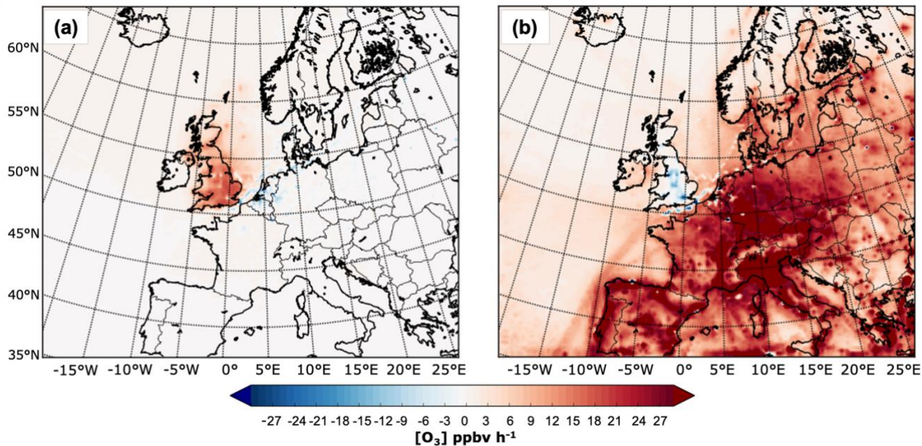
Figure 8. Net midday (11:00–14:00 UTC) surface chemical production rate in ppb h -1 on July 2015 for O 3 from UK (a) and European anthropogenic NO x emissions (b).
