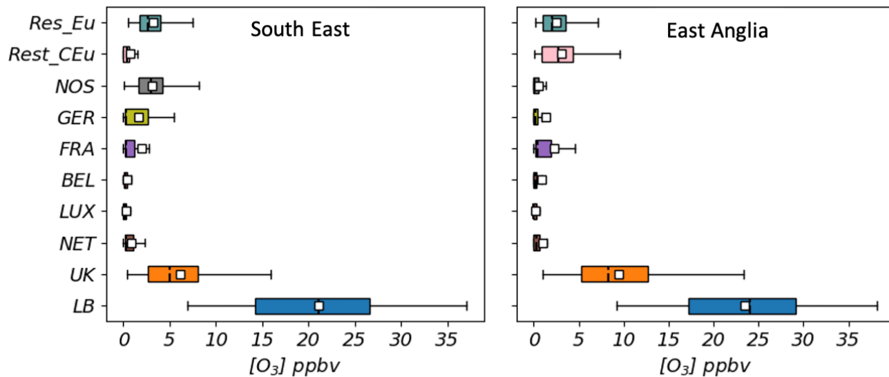
910 Figure 12. Hourly contributions, in ppbv, to surface O 3 at 2 UK receptor regions from 10 source regions (UK, background (LB), the Netherlands, Luxembourg, Belgium, France, Germany, rest of Central Europe, North Sea and English Channel (NOS) and rest of Eu) for AOT40 between May and August. The lower and upper ends of the boxes indicate the 25 th and 75 th percentiles the black dashed line the median, the white boxes the mean and the whiskers the minima and maxima.
