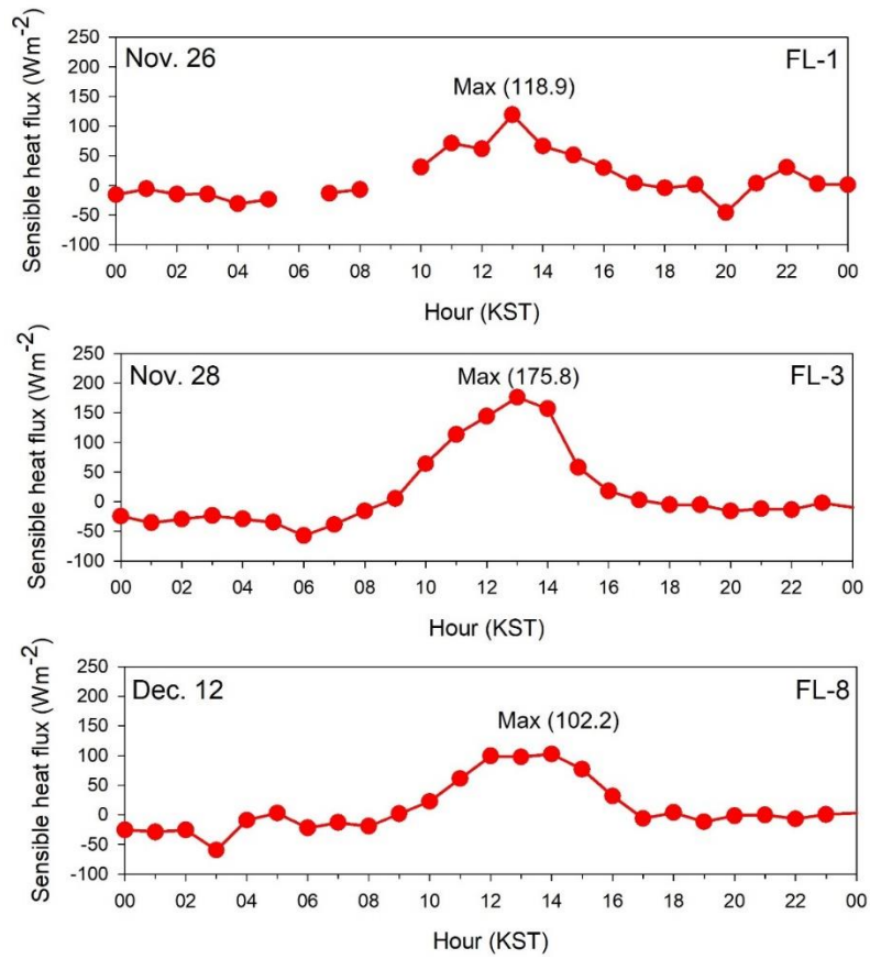
Figure S1. Diurnal variations of sensible heat fluxes on Nov. 26 (FL-1), Nov. 28 (FL-3), and Dec. 12(FL-8), observed at Seosan during GMAP-2020 campaign.
