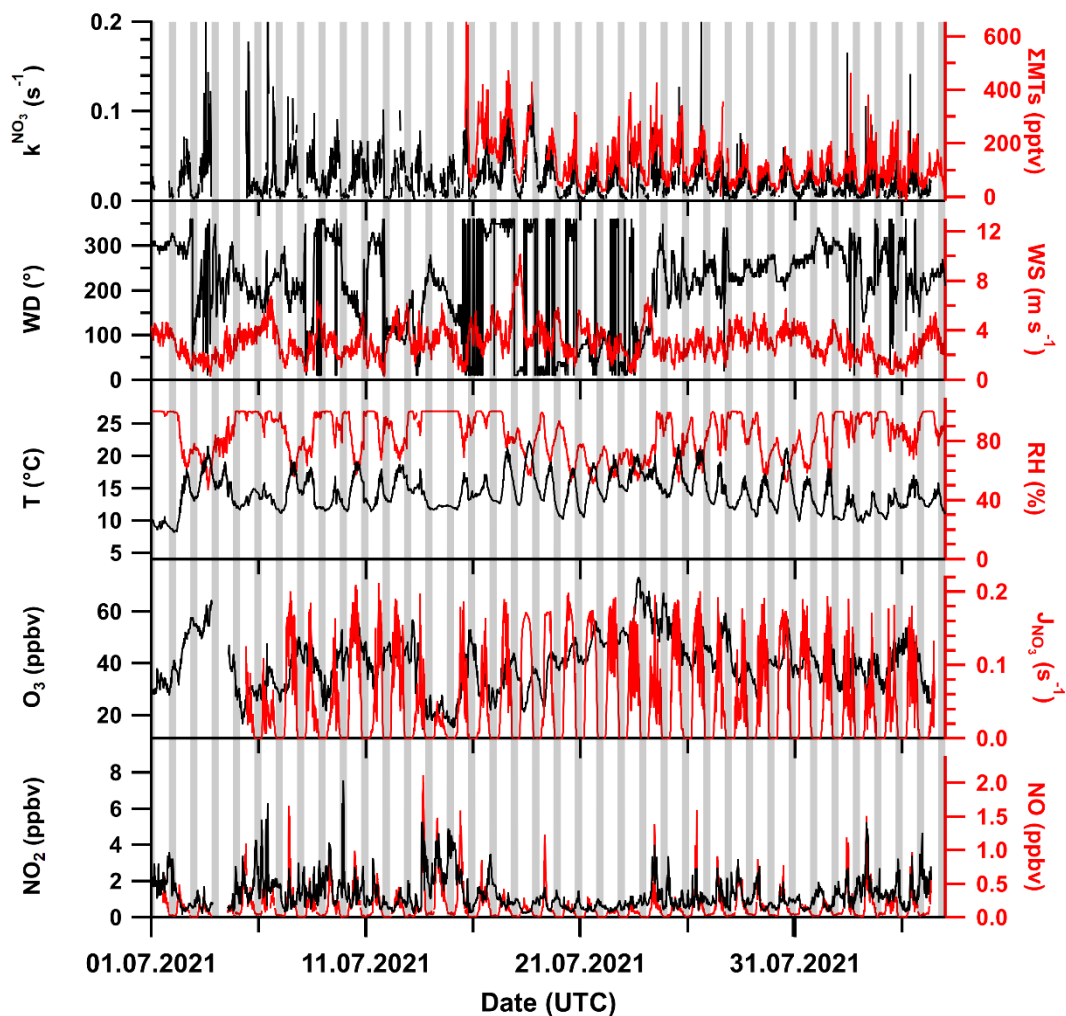
Figure 1: Overview of key measurements during the TO2021 campaign with wind direction (WD), temperature (T), sum of monoterpenes ( \Sigma MT, PTR8000 and scaled VOCUS), wind speed (WS), relative humidity (RH), \text{NO}_3 photolysis rate coefficient ( J_{\text{NO}_3} ). Meteorological data was provided by the German Meteorological Service (DWD). Nighttime periods are shaded grey. The x-axis ticks are at 00:00 UTC.
