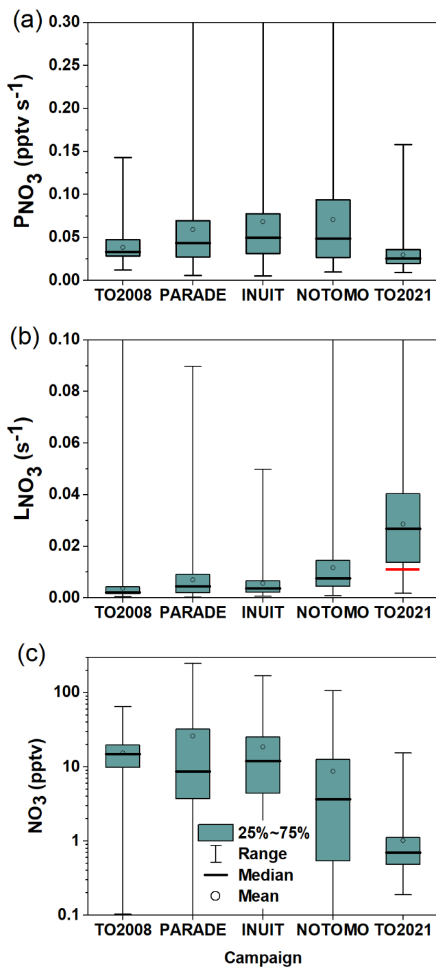
890 Figure 13: NO 3 production rates (a), loss rates (b) and mixing ratios (c) measured during 5 campaigns on the summit of Kleiner Feldberg between 2008 and 2021. Boxes represent the range between the first and third quartiles, whiskers denote the full range of values. The red line represents the median of directly measured k^{NO_3} during TO2021 at nighttime.
