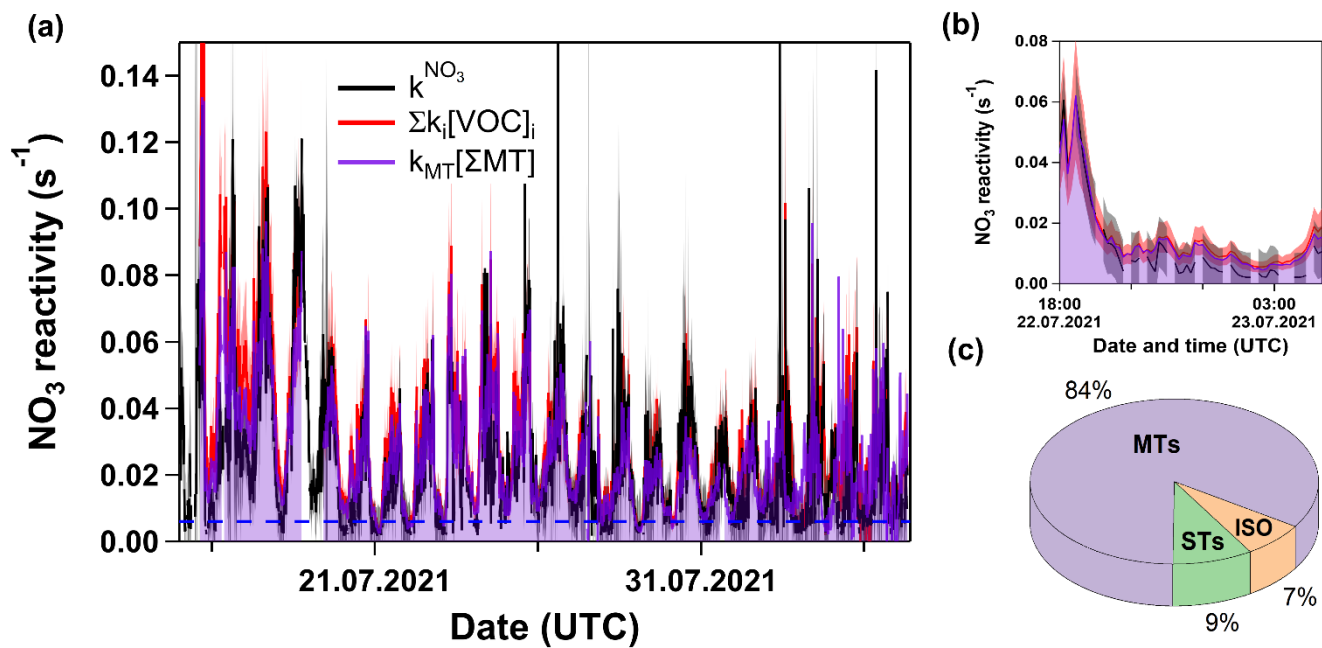
815 Figure 5: (a) Time-series of k^{NO_3} and \Sigma k_i[VOC]_i . Dashed blue line marks the LOD of the k^{NO_3} measurement. The purple line together with the same-coloured shade represents the contribution of monoterpenes. The red- and grey-shaded areas represent the uncertainty associated with k^{NO_3} and \Sigma k_i[VOC]_i , respectively. (b) Same as (a) but with a detailed view of the night between the 22 nd and 23 rd July presented in Fig.2b. (c) Pie-chart of fractional contributions of isoprene, monoterpenes and sesquiterpenes to \Sigma k_i[VOC]_i over this time period.
