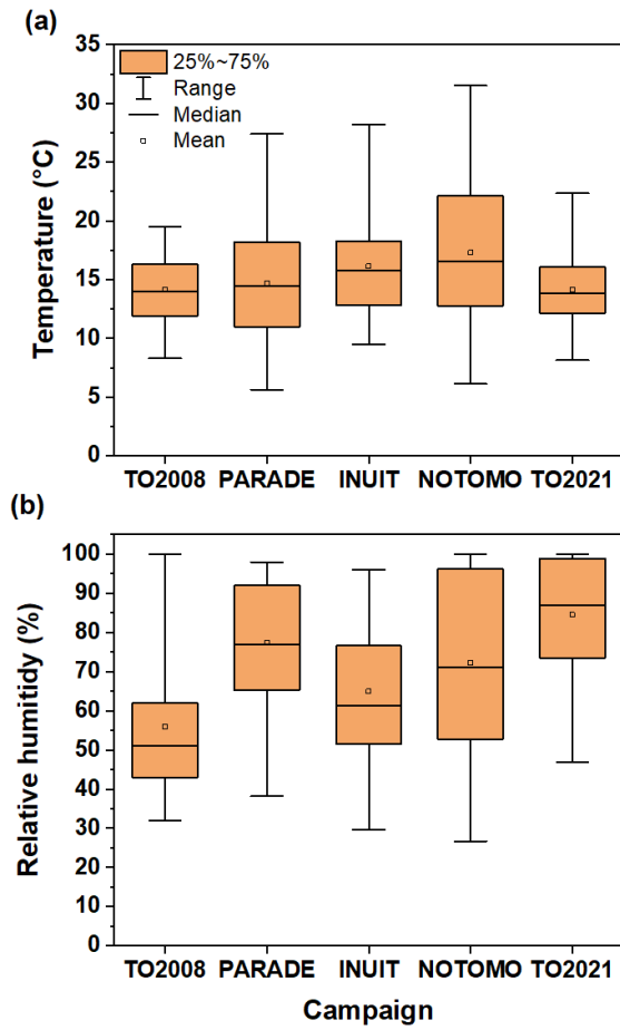
885 Figure 12: Distributions of (a) temperature and (b) relative humidity during five campaigns at the Kleiner Feldberg between 2008 and 2021. Boxes represent the range between the first and third quartiles, whiskers denote the full range of values.
