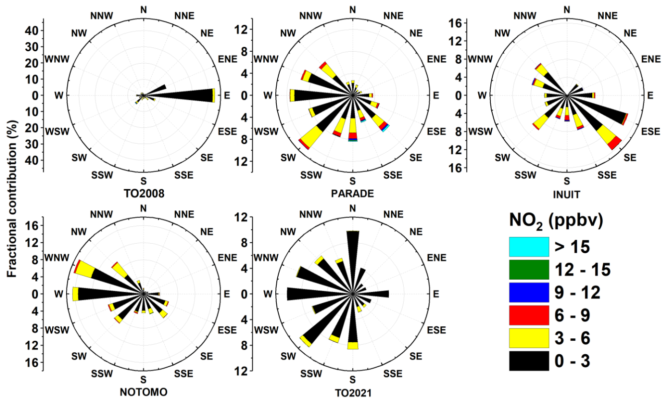
880 Figure 11: Wind roses indicating the dependence of NO 2 mixing ratio on the wind direction during TO2008, PARADE, INUIT, NOTOMO and TO2021. Wind directions were provided by HLNUG for TO2008 and NOTOMO, by a weather station in PARADE and INUIT (Drewnick et al., 2012) and by the German meteorological service DWD in TO2021.
