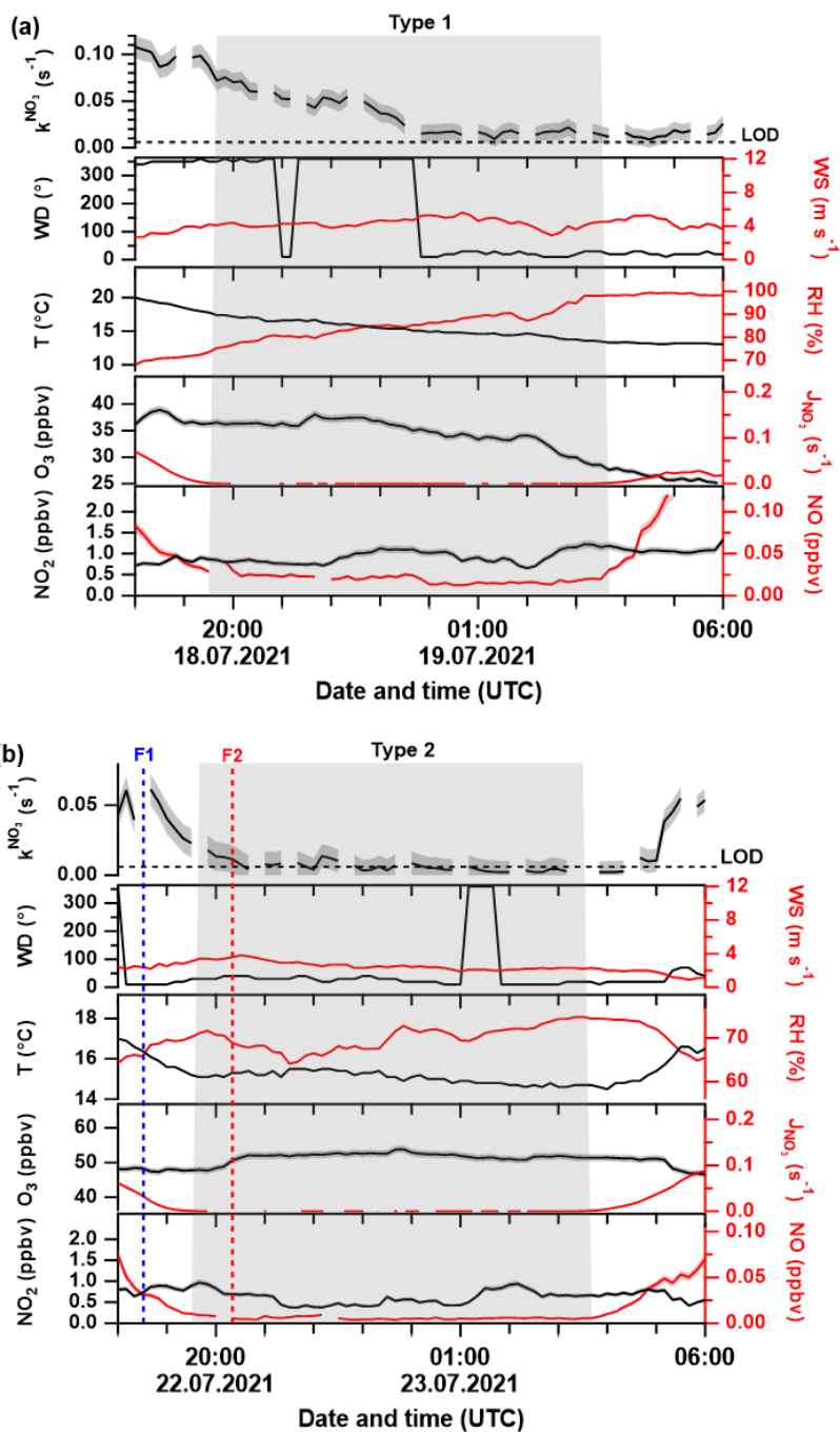
Figure 2: Time-series of directly measured NO_3 reactivity ( k^{NO_3} ) together with auxiliary measurements during Type-1 (a) and Type-2 nights (b). F1 and F2 mark times at which drone-assisted temperature and relative humidity profiles were measured. The grey-shaded area represents nighttime. Abbreviations are defined in caption of Fig.1. The shaded areas in the colour of the lines denote the corresponding uncertainty of the measured parameter.
