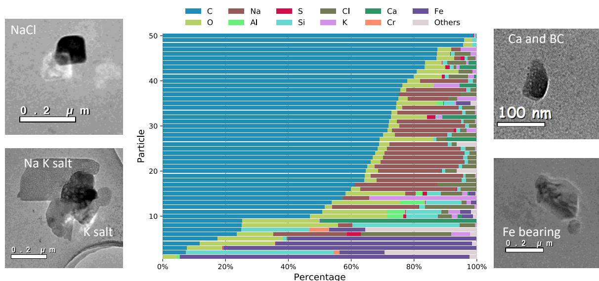
Figure 3. Elemental composition (mass percentage) and representative microphysical images of particles from TEM-EDX analysis for the collected sample (sampled at 2017/08/24 9:43-9:49 UTC, at 319.4 m) near ASI.
