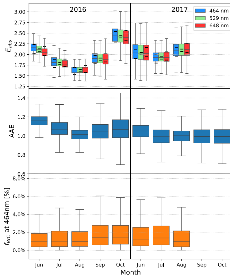
240 Figure 2. Monthly percentiles (10%, 25%, 50%, 75%, and 90%) of absorption enhancement E_{abs} , AAE (between 464 and 648 nm), and calculated BrC contribution to total absorption at 464 nm as box-whisker plots spanning the fire season in 2016 and 2017. E_{abs} is calculated by assuming an AAE of 1 for the fresh BC. The solid black lines in the upper panel indicate the upper and lower boundary of the calculated median E_{abs} when the AAE is in the range of 0.8 to 1.4.
