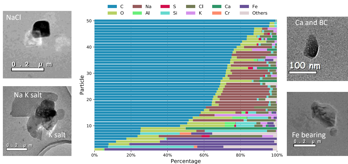
Figure 3. Elemental composition and representative microphysical images of particles from TEM-EDX analysis for the collected sample (sampled at 2017/08/24 9:43-9:49 UTC, at 319.4 m) near ASI.
