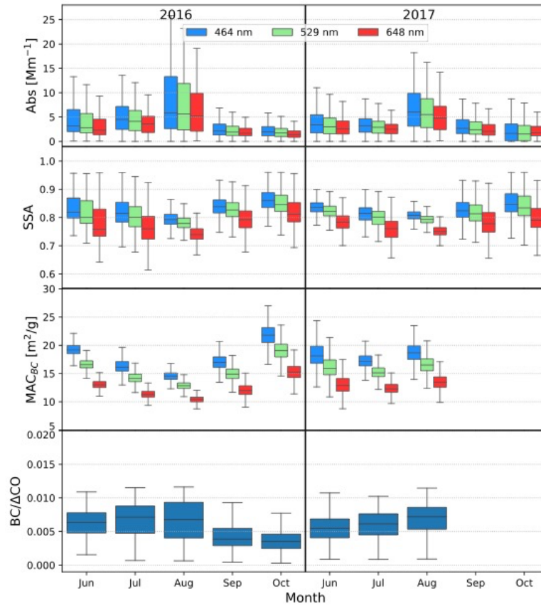
200 Figure 1. Monthly percentiles (10%, 25%, 50%, 75%, and 90%) of aerosol absorption coefficient, SSA, MAC_{BC} , and BC/\Delta CO as box-whisker plots spanning the fire season in 2016 and 2017. The light blue, green and red colours of absorption, SSA, and MAC_{BC} indicate observations at wavelengths of 464, 529, and 648 nm, respectively.
