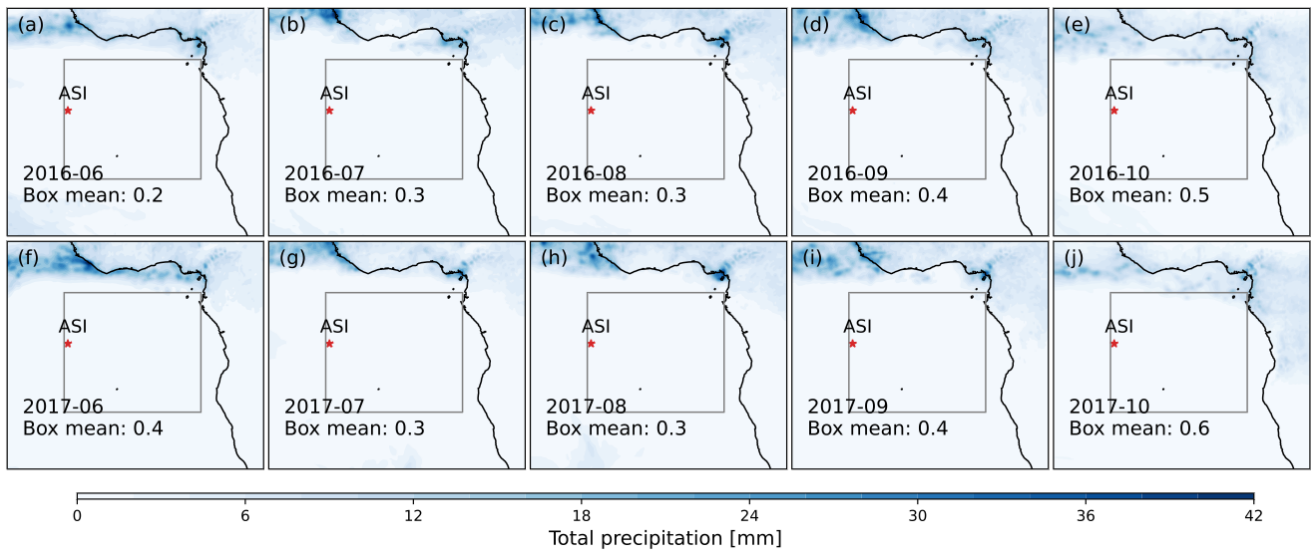
Figure 7. Same with Fig 6, but with precipitation.
