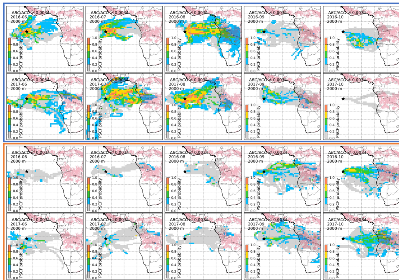
Figure 9. The spatial distribution of potential source contribution function (PSCF) during the African fire season in 2016 and 2017. The 7-day backward trajectories in the upper blue and lower orange rectangles indicate air mass flow when BC/\Delta CO > or \leq 0.0034 , respectively. Different colours indicate the probability of different transport paths of the plumes. Note the trajectories are initiated at an altitude of 2000 m at the sampling site (marked as the black star) on ASI. The pink areas on the continent indicate savannah, the main burning material in each month.
