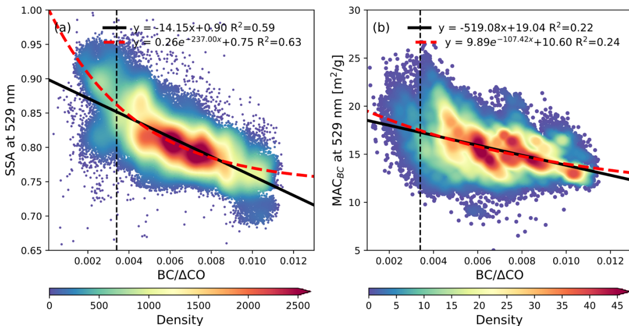
305 Figure 4. Relations of BC/ \Delta CO with (a) SSA and (b) MAC_{BC} at 529 nm wavelength. The solid black lines represent the linear regressions, and the red dash lines are the curve fitting with the function displayed in the legend. The colour scale indicates the density of the data in each plot. The vertical dashed black lines in each plot corresponding to BC/ \Delta CO = 0.0034
