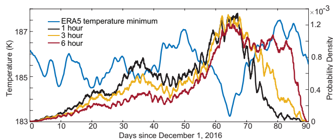
Figure 3. The daily running mean zonal minimum temperature averaged between 15°S and 15°N and 79 to 103 hPa for DJF 2017 from ERA5 data (blue), and the daily running mean PDFs of the time at which the cold point is observed by 1- (black), 3- (orange), and 6-h (red) trajectories. Trajectories are run in reverse from the end of this timeframe, so the distribution shifts to the left with increased transit times.
