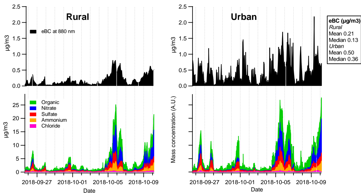
375 Figure 8. Concentrations of eBC and PM 1 chemical species at both sites during overlapping urban and rural measurement period. 1 hour averages for eBC, 20 minutes for PM 1 chemical species. Absolute concentrations of PM 1 at the urban site was not possible to extract due to uncertainties in the calibration.
