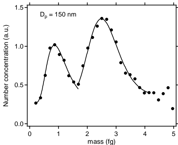
325 Figure 5. Measured DMA-APM spectrum for urban particles with a diameter of 150 nm (black markers). The spectrum is the average number concentration (arbitrary units) of eleven samples from all sampling days. Two lognormal fits are shown in black.
