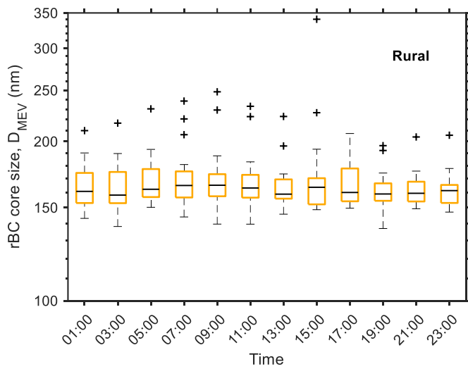
Figure 4. Box-plot showing the daily pattern of rBC GMD (2 h averages) as measured by the SP2, at the urban and rural sites. Boxes show the median, 25 th and 75 th percentiles, with values more than 1.5 below or above those considered outliers (+).
