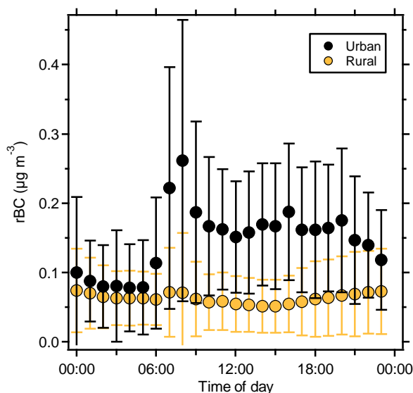
235 Figure 2. Diurnal cycles of rBC mass concentrations ( \pm 1\sigma ) from the urban and rural sites as measured by the SP2. Values are averages of data collected during 34 (rural) and 41 (urban) days of sampling.
