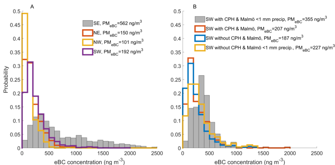
325 Figure 7. Trajectory analysis of different air mass origins, with corresponding median eBC mass concentrations in the legend. Panel A shows histograms with the observed eBC from the Aethalometer at Hyltemossa from year 2018 for air masses originating from SE, NE, NW and SW as defined in Fig. S3. Panel B shows the eBC histogram from all SW air masses with or without influence from the Copenhagen (CPH) and Malmö region.
