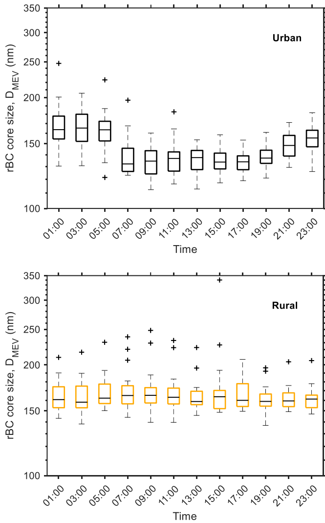
Figure 4. Box-plot showing the daily pattern of rBC GMD (2 h averages) as measured by the SP2, at the urban and rural sites. Boxes show the median, 25 th and 75 th percentiles, with values more than 1.5 below or above those considered outliers (+).
