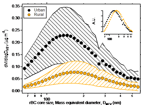
Figure 3. Average mass-size distribution of BC cores for the urban (black) and rural (orange) campaigns. Filled areas show \pm 1\sigma . 290 Insert shows the normalized distribution for comparison of the modes. Dip at 270 nm is due to erroneous stitching of high and low gain detector channels.
