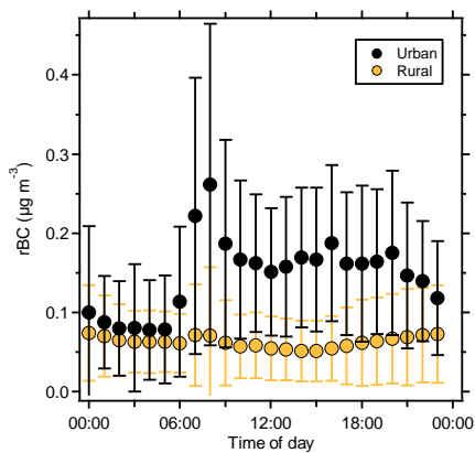
240 Figure 2. Diurnal cycles of rBC mass concentrations ( \pm 1\sigma ) from the urban and rural sites as measured by the SP2. Values are averages of data collected during 34 (rural) and 41 (urban) days of sampling.
