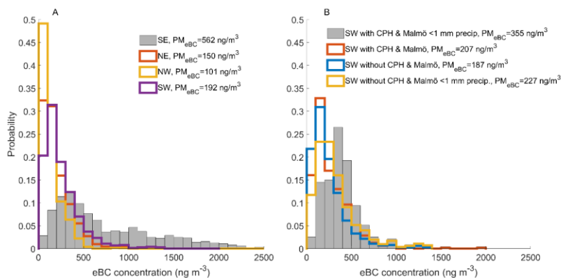
360 Figure 7. Trajectory analysis of different air mass origins, with corresponding median eBC mass concentrations in the legend. Panel A shows histograms with the observed eBC from the Aethalometer at Hyltemossa from year 2018 for air masses originating from SE, NE, NW and SW as defined in Fig. S3S4. Panel B shows the eBC histogram from all SW air masses with or without influence from the Copenhagen (CPH) and Malmö region.
