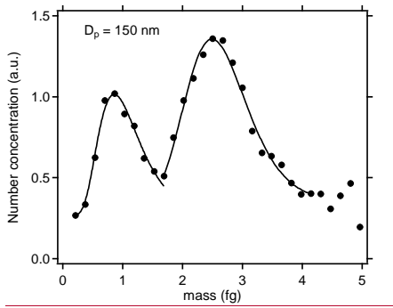
330 Figure 5. Measured DMA-APM spectrum for urban particles with a diameter of 150 nm (black markers). The spectrum is an the average number concentration (arbitrary units) of eleven samples from all sampling days. Two lognormal fits are shown in black.
