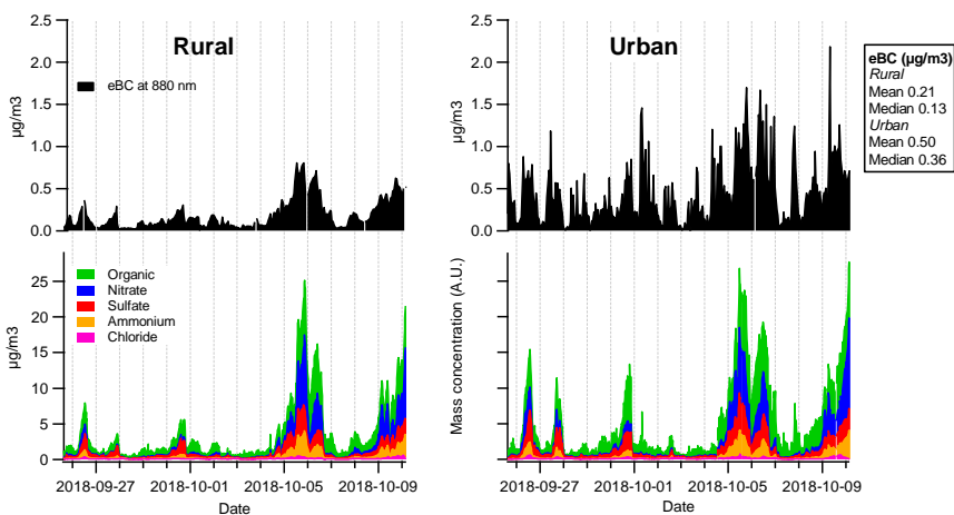
Figure 8. Concentrations of eBC and PM 1 chemical species at both sites during overlapping urban and rural measurement period. 1 hour averages for eBC, 20 minutes for PM 1 chemical species. Absolute concentrations of PM 1 at the urban site was not possible to extract due to uncertainties in the calibration.
