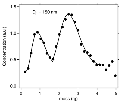
300 Figure 5. Measured DMA-APM spectrum for urban particles with a diameter of 150 nm (black markers). The spectrum is an average of eleven samples from all sampling days. Two lognormal fits are shown in black.
