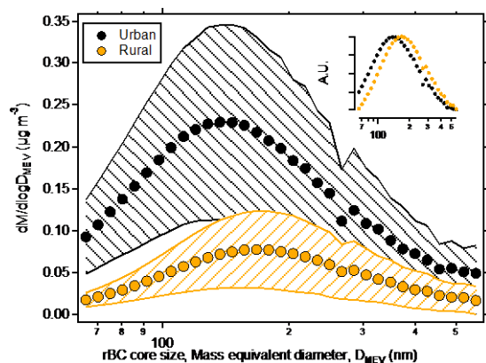
260 Figure 3. Average mass-size distribution of BC cores for the urban (black) and rural (orange) campaigns. Filled areas show \pm 1\sigma . 265 Insert shows the normalized distribution for comparison of the modes. Dip at 270 nm is due to erroneous stitching of high and low gain detector channels.
