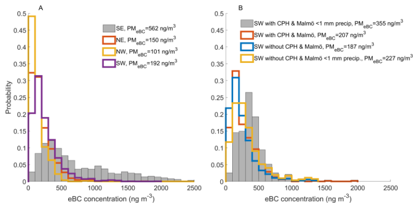
335 Figure 7. Trajectory analysis of different air mass origins, with corresponding median eBC mass concentrations in the legend. Panel A shows histograms with the observed eBC from the Aethalometer at Hyltemossa from year 2018 for air masses originating from SE, NE, NW and SW as defined in Fig. S3. Panel B shows the eBC histogram from all observations corresponding to SW air masses with or without influence from the Copenhagen (CPH) and Malmö region.
