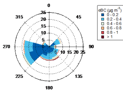
Figure 6. Wind rose showing the frequency of different wind directions (30° resolution) during the rural campaign and corresponding concentrations of eBC.
