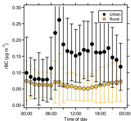
Figure 2. Diurnal trends of rBC mass concentrations ( \pm 1\sigma ) from the urban and rural sites as measured by the SP2. Values are averages of data collected during 34 (rural) and 41 (urban) days of sampling.
