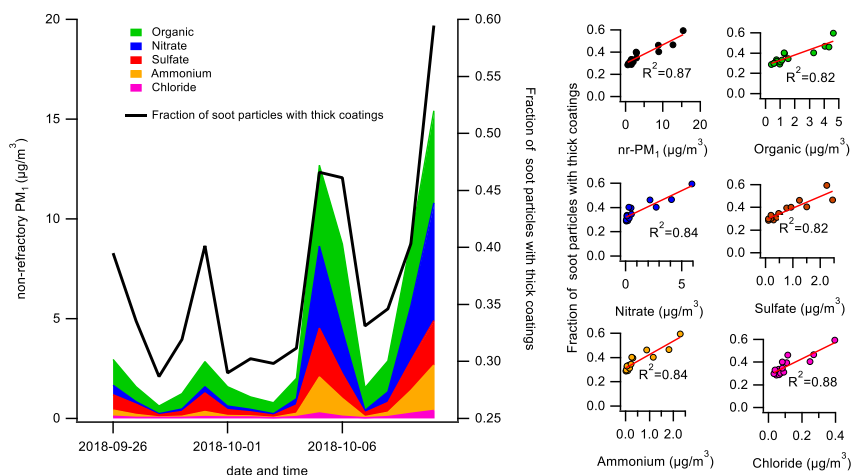
Figure 89. Comparison of chemically resolved non-refractory PM 1 concentration and the fraction of thickly coated BC cores, with a mass equivalent diameter corresponding to ~136 nm, in the urban setting. Left: time series. Right: scatterplots of thickly coated BC particle fraction vs non refractory-PM 1 and subcategories thereof. 24 hour averages.
