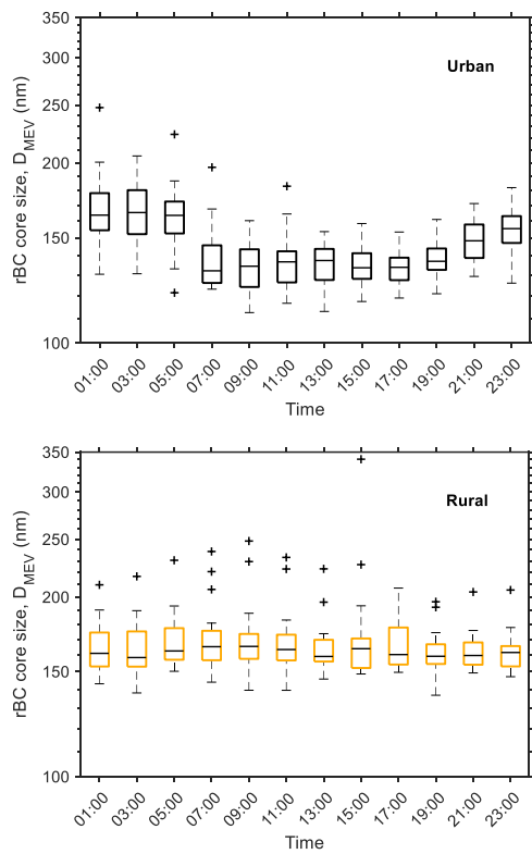
295 Figure 34. Box-plot showing the daily pattern of rBC GMD (2 h averages) as measured by the SP2, at the urban and rural sites. Boxes show the median, 25 th and 75 th percentiles, with values more than 1.5 below or above those considered outliers (+). At the urban site, the influence of local traffic shifts the size distribution to lower diameters when traffic intensity is highest.
