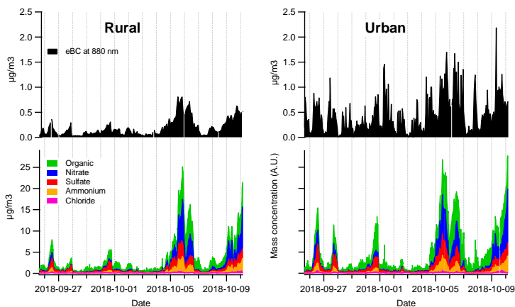
Figure 78. Concentrations of eBC and PM 1 chemical species at both sites during overlapping urban and rural measurement period. 1 hour averages for eBC, 20 minutes for PM 1 chemical species. Absolute concentrations of PM 1 at the urban site was not possible to extract due to uncertainties in the calibration.
