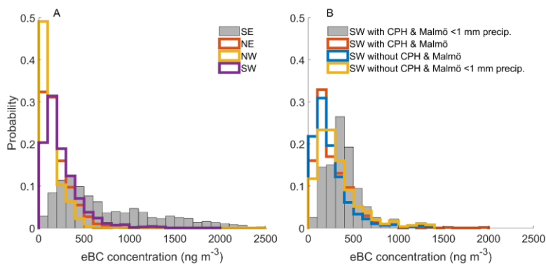
Figure 67. Panel A shows histograms with the observed eBC from the Aethalometer at Hyltemossa from year 2018 for air masses originating from SE, NE, NW and SW as defined in Fig. S2S3. Panel B shows the eBC histogram from all observations corresponding to SW air masses with or without influence from the Copenhagen and Malmö region.
