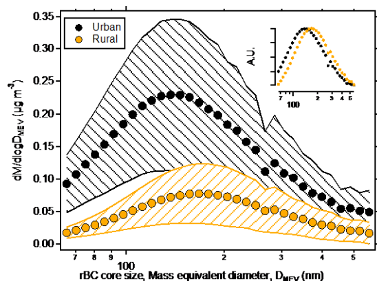
Figure 23. Average mass-size distribution of BC cores for the urban (black) and rural (orange) campaigns. Filled areas show \pm 1\sigma . Insert shows the normalized distribution for comparison of the modes. Dip at 270 nm is due to erroneous stitching of high and low gain detector channels.
