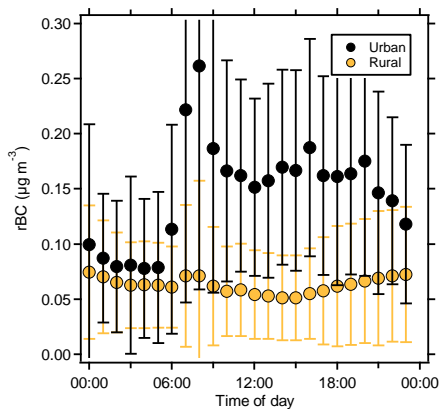
Figure 12. Diurnal trends of rBC mass concentrations ( \pm 1\sigma ) from the urban and rural sites as measured by the SP2. Values are averages of data collected during 34 (rural) and 41 (urban) days of sampling.
