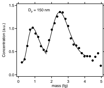
300 | Figure 45. Measured DMA-APM spectrum for urban particles with a diameter of 150 nm (black markers). The spectrum is an average of eleven samples from all sampling days. Two lognormal fits are shown in black.
