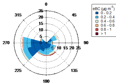
305 | Figure 56. Wind rose showing the frequency of different wind directions (30° resolution) during the rural campaign and corresponding concentrations of eBC.
